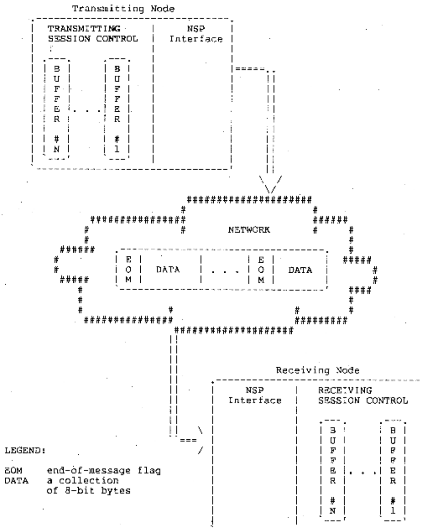
Figure 2. Model of Data Flow as Seen by Session Control.
