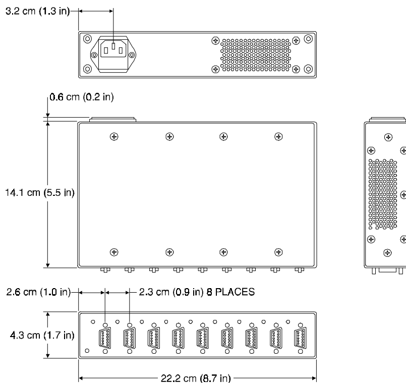
Figure B-1 Mechanical Dimensions
