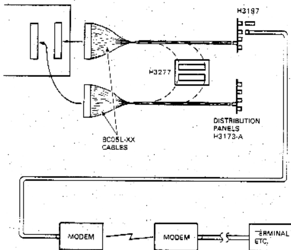
Figure 4-2 Using Loopback Connectors in EIA-232-D Installations
