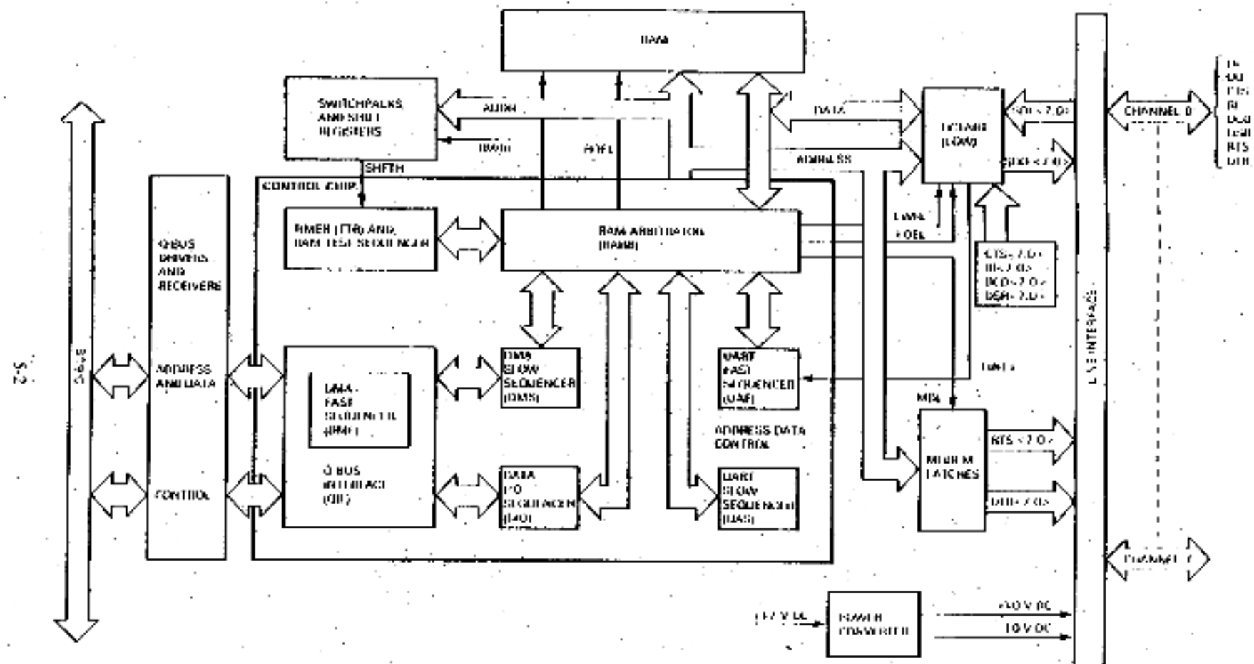
Figure 5-1 DHQII Block Diagram
