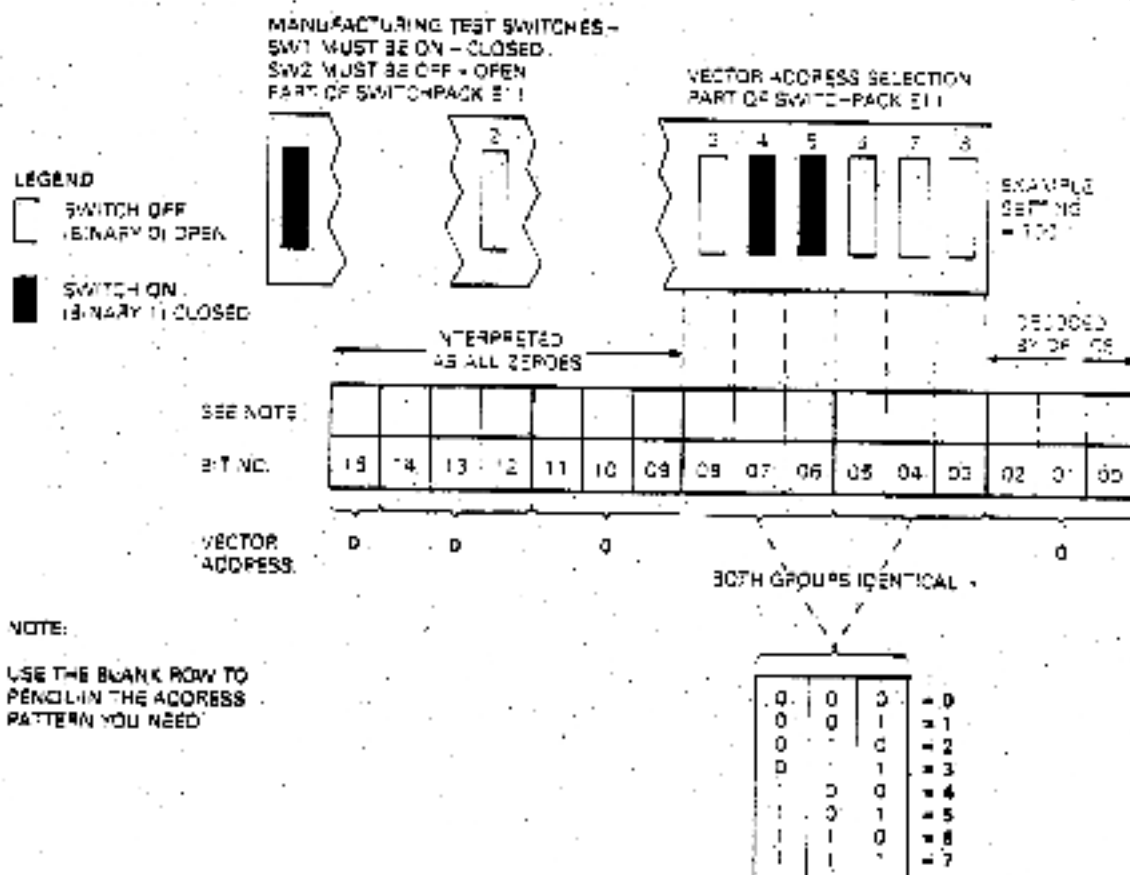
Figure 2-3. Setting the Vector Address
