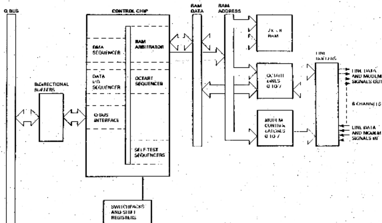
Figure 1-5 DHQ11 Functional Block Diagram
