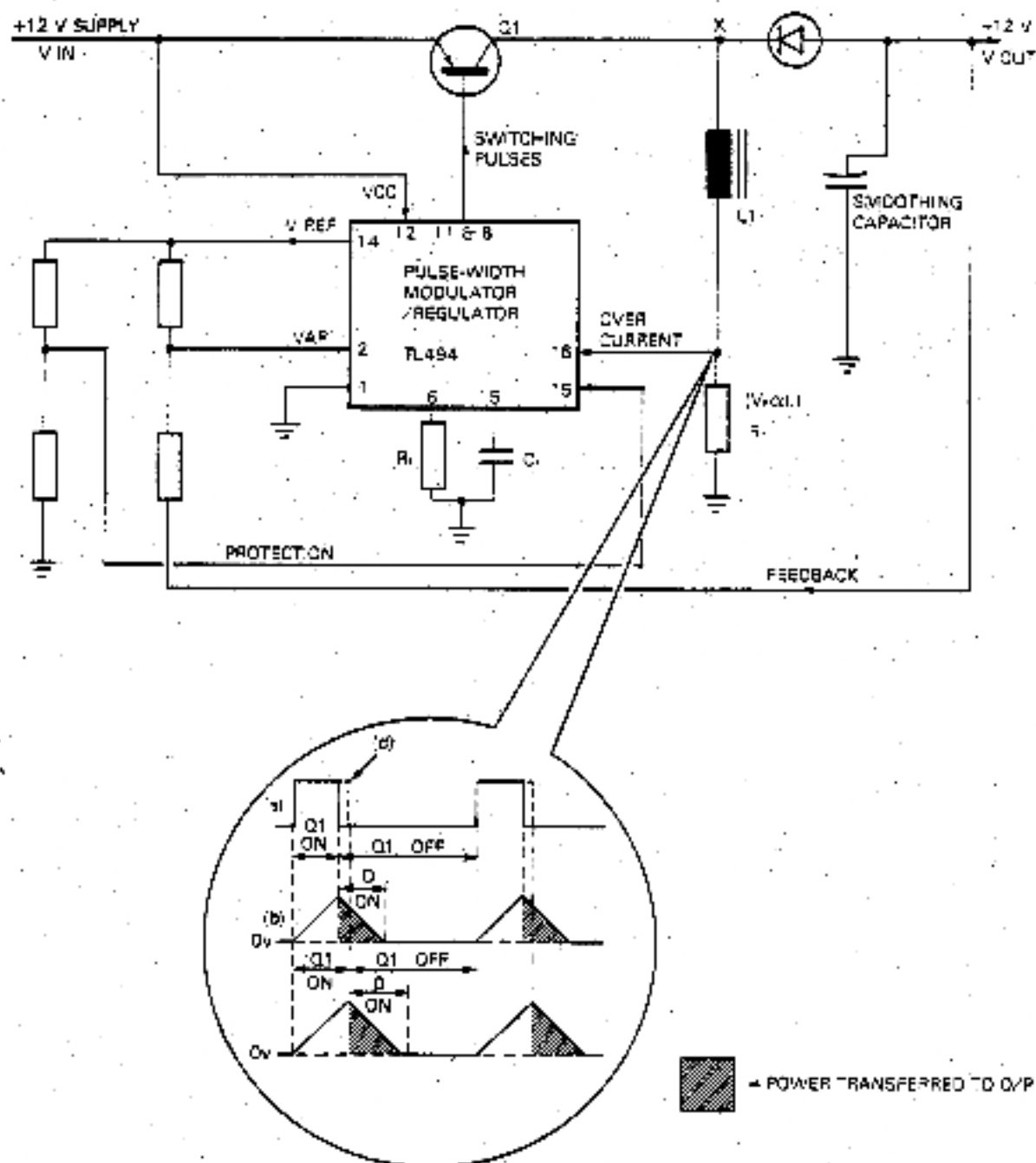
Figure 5-6 Voltage Converter
