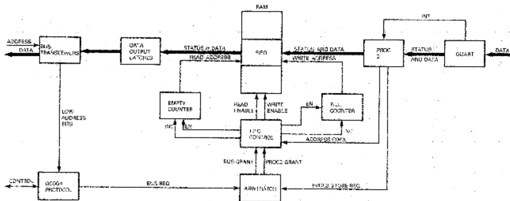
Figure 4-14 Receiving a Character
