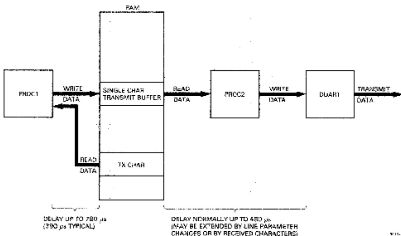
Figure 4-10 Single-Character Transmit
