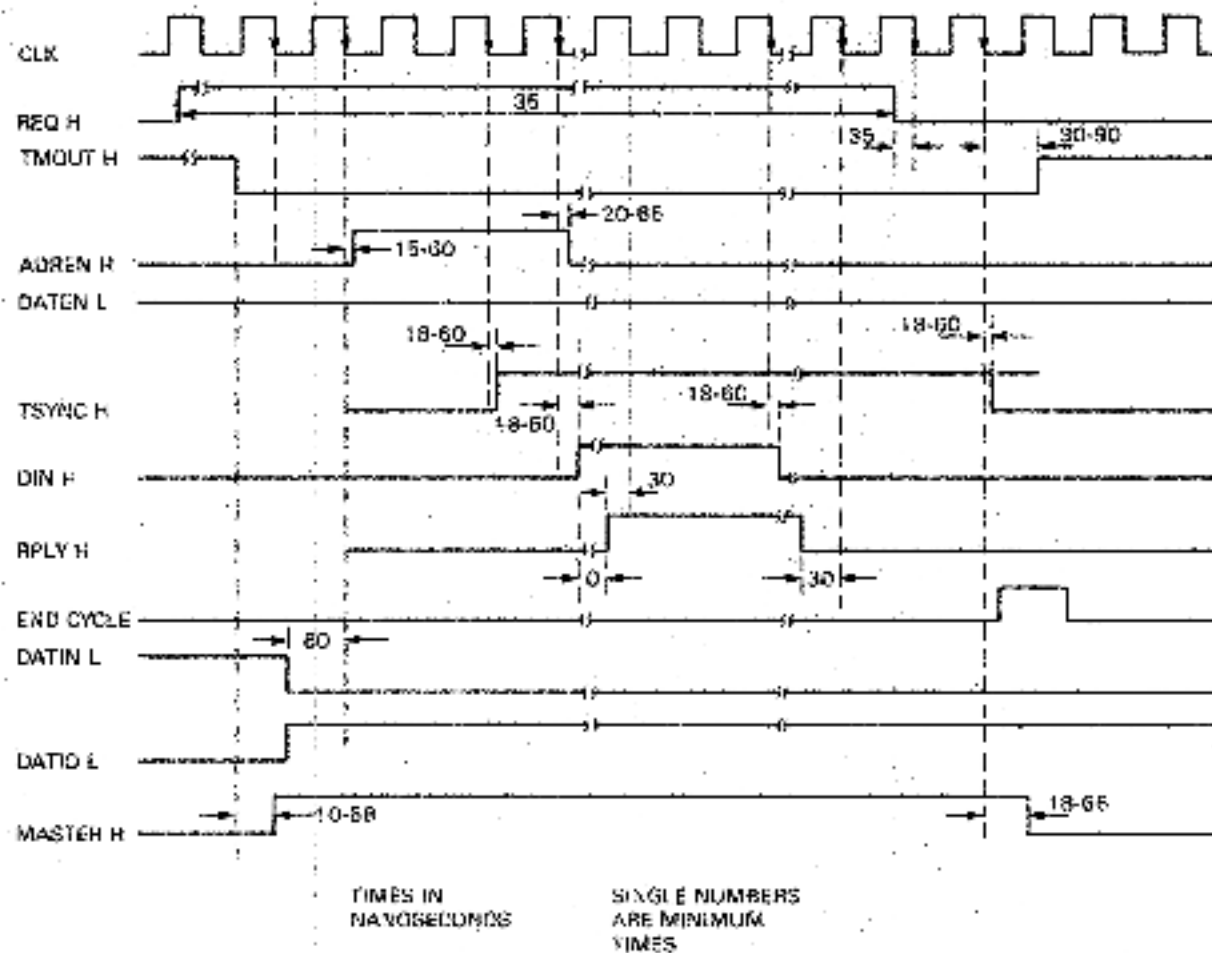
Figure A-19 DC010 Timing Diagram
