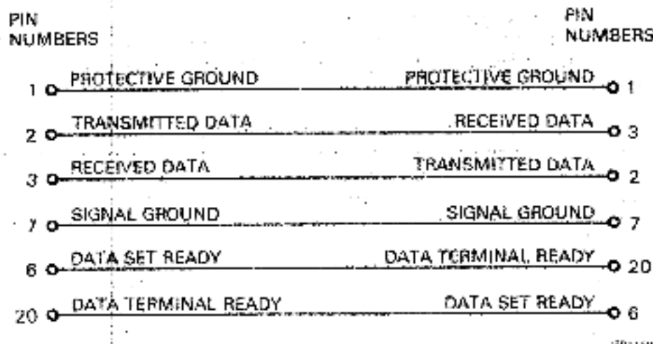
Figure 2-8 Null Modem Cable Connections
