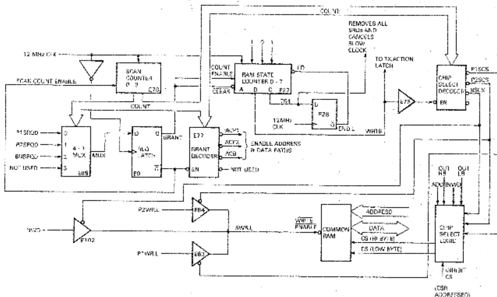
Figure 4-18 RAM Arbitration and Timing
