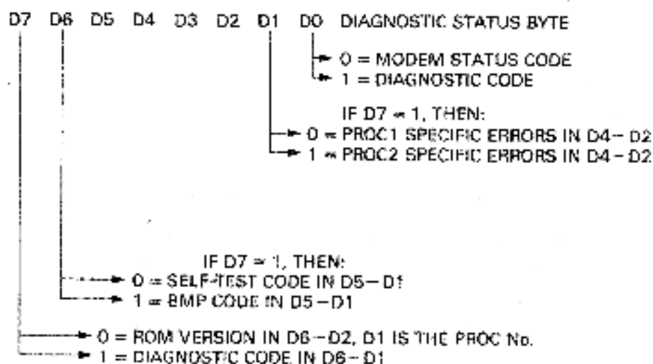
Figure 3-2 Diagnostic/Status Byte
