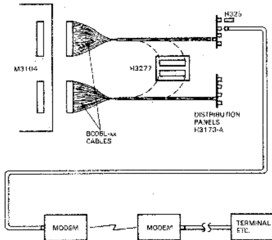
Figure 5-1 Troubleshooting Connection Diagram
