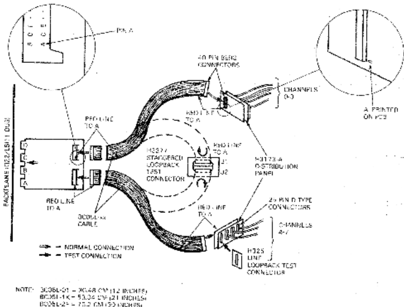
Figure 2-3 DHV11 Installation
