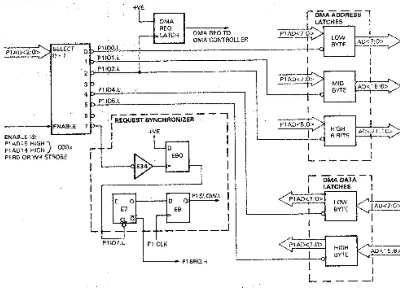
Figure 4-15 PROC1 I/O Decoding
