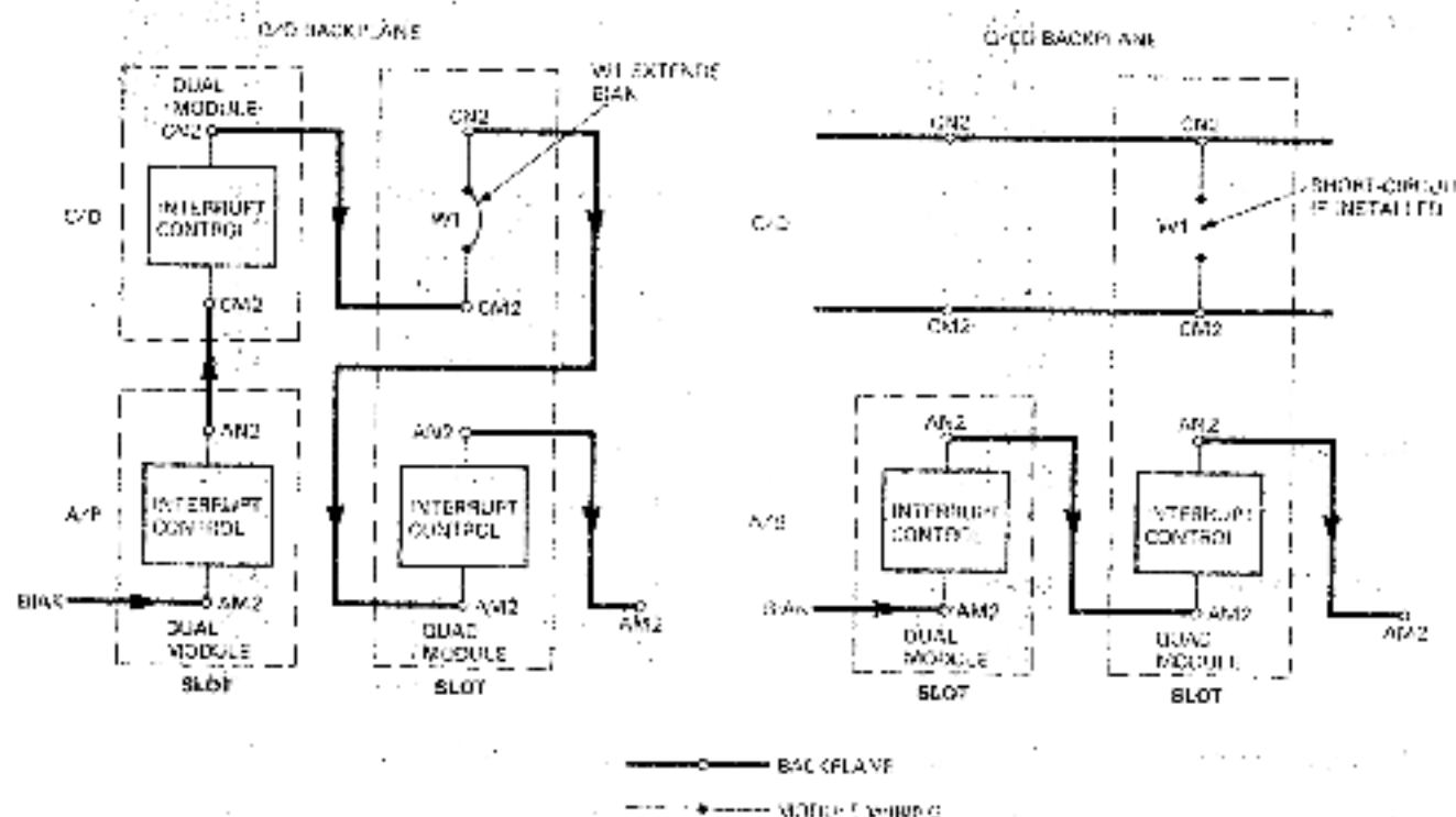
Figure 2-2 Bus Grant Continuity
