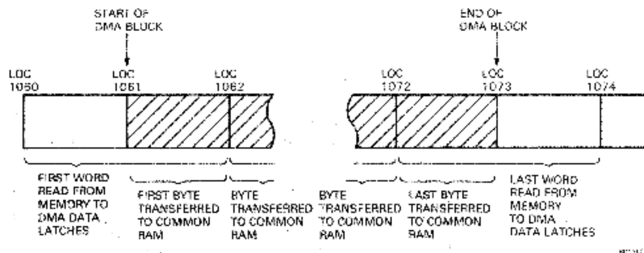
Figure 4-12 DMA Character Handling
