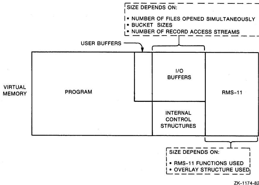
Figure 4-1: RMS-11 Task Structure
