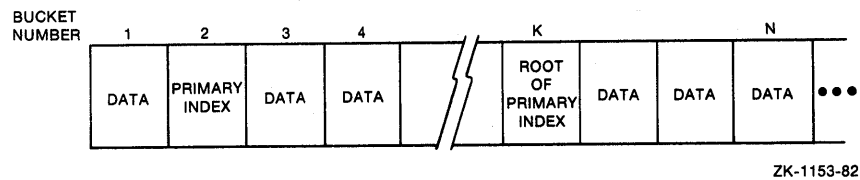
Figure 6-1: Single-Area Indexed File
