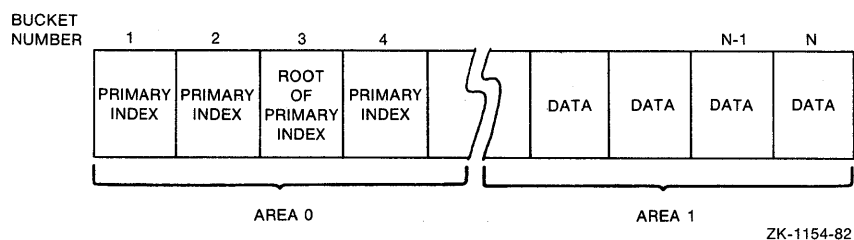
Figure 6-3: Two-Area Indexed File
