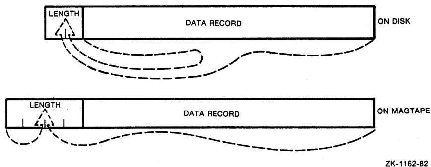
Figure 2-4: Count Field on Disk and Tape
