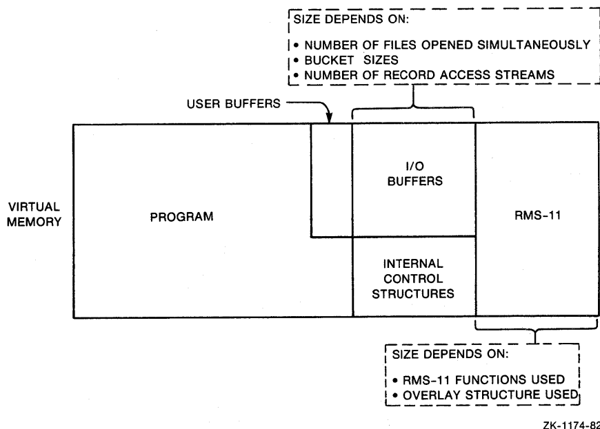
Figure 3-1: RMS-11 Task Structure
