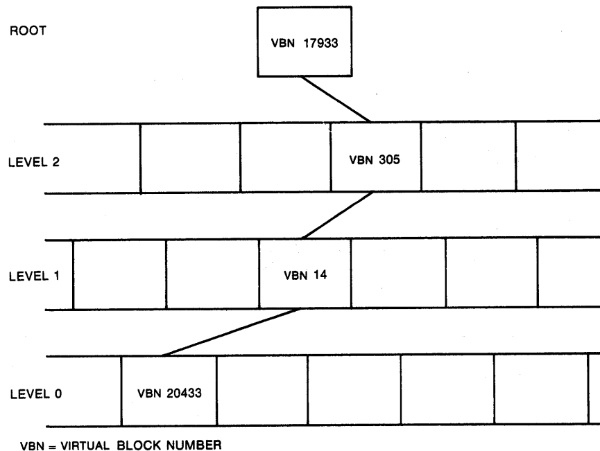
Figure 6-2: Example of Single-Area Indexed File
