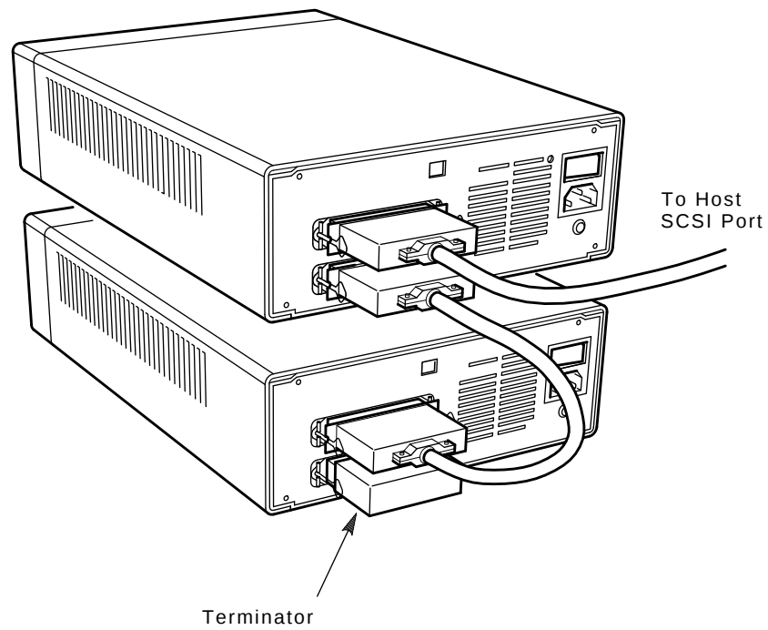
Figure 4-3 Connecting Two RRD40 Expansion Boxes
