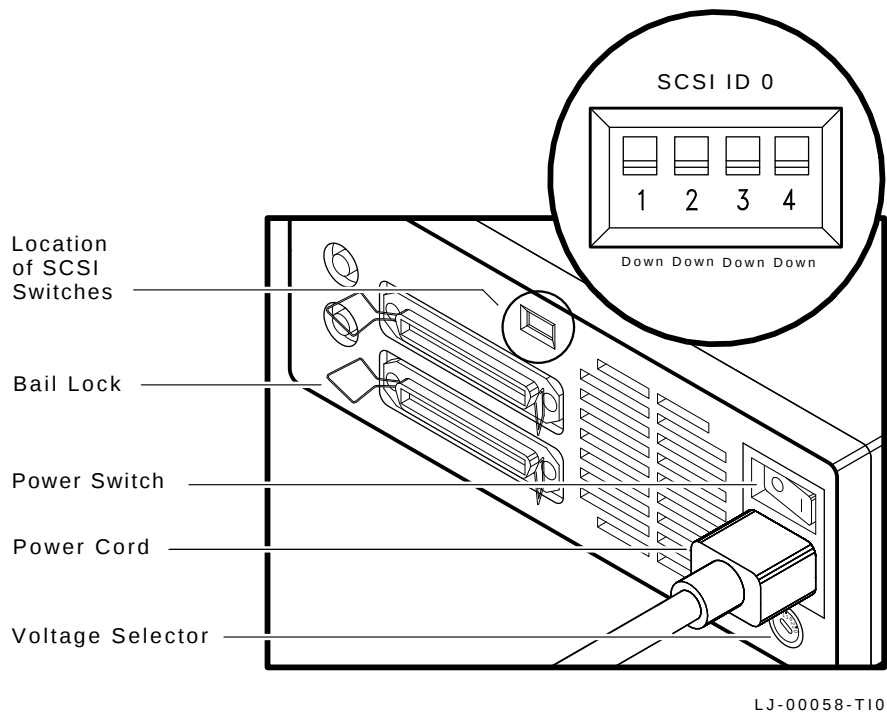
Figure 4-4 RRD40 Voltage Selector and SCSI ID Switch Positions
