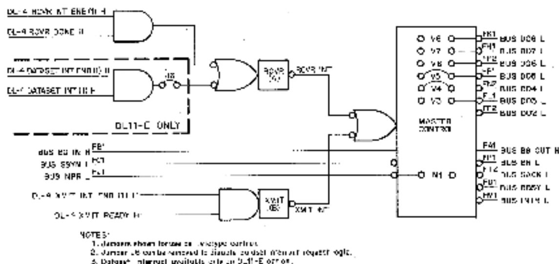
Figure 5-3 Internet Control Logic – Simplified Diagram
