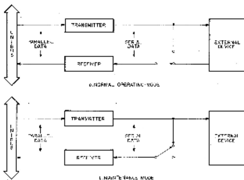
Figure 5-8. Operating Modes
