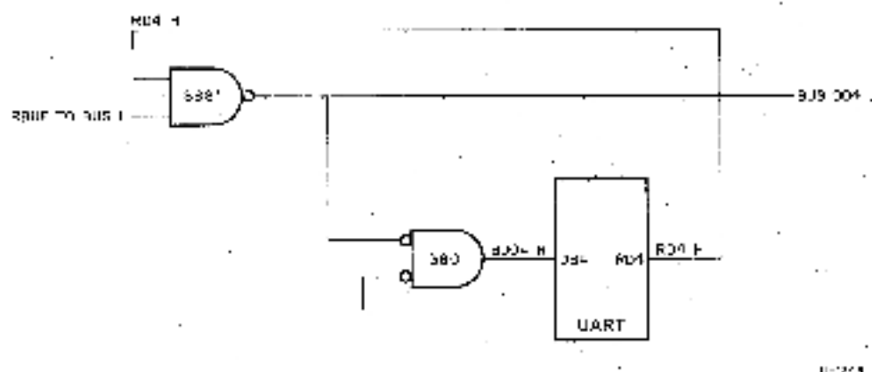
Figure 5-1 RBUF and XBUF Gating Logic - Simplified Diagram (one bit position)
