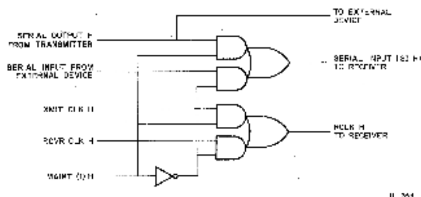
Figure 3-9 Maintenance Logic - Simplified Diagram
