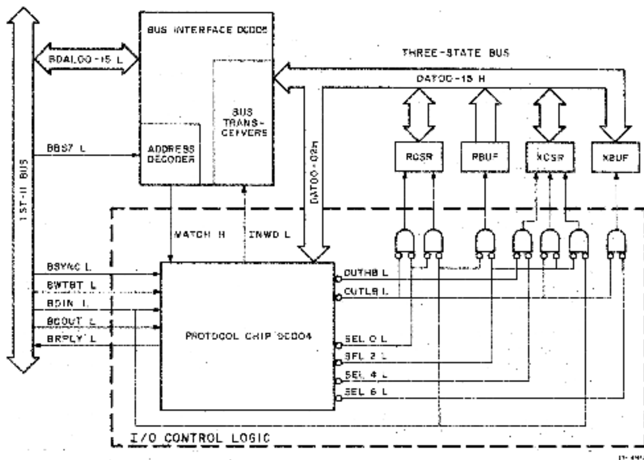
Figure 5-3 I/O Control Logic, Block Diagram
