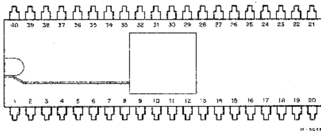
Figure A-12 UART Pin Locations
