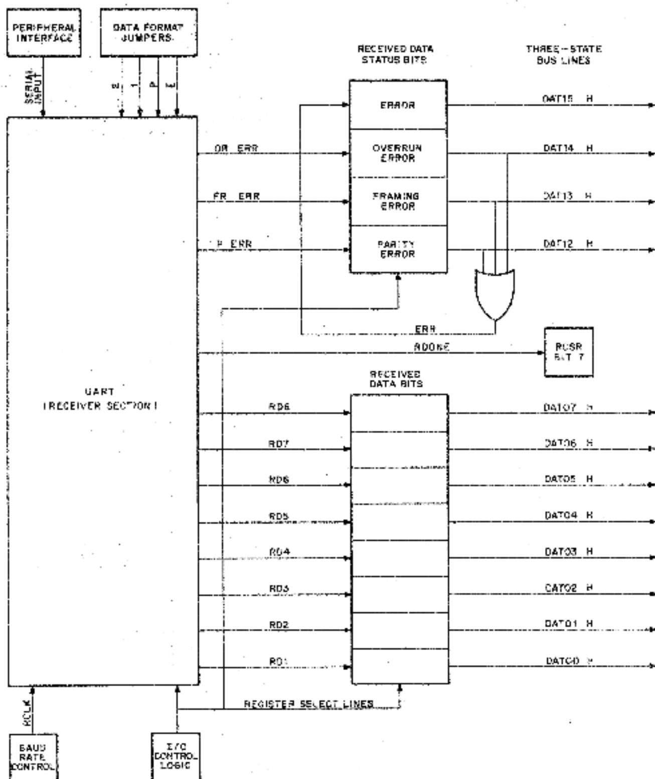
Figure S-12 DLV11-E and DLV11-F RBUP Data Flow
