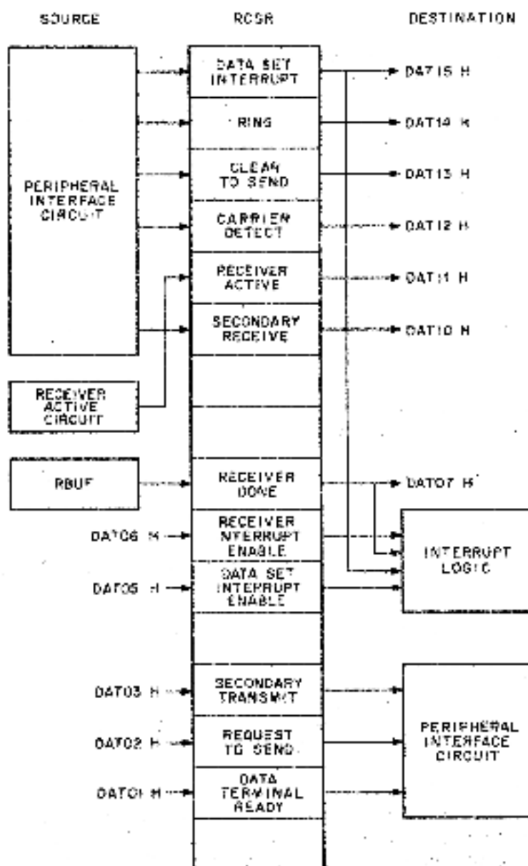
Figure 5-6 DLV11-E RCSR Data Flow
