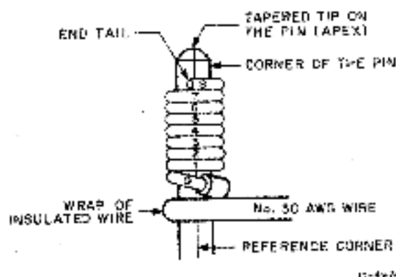
Figure B-1 Solderless Wrapped Connection on Wire Wrap Pin
