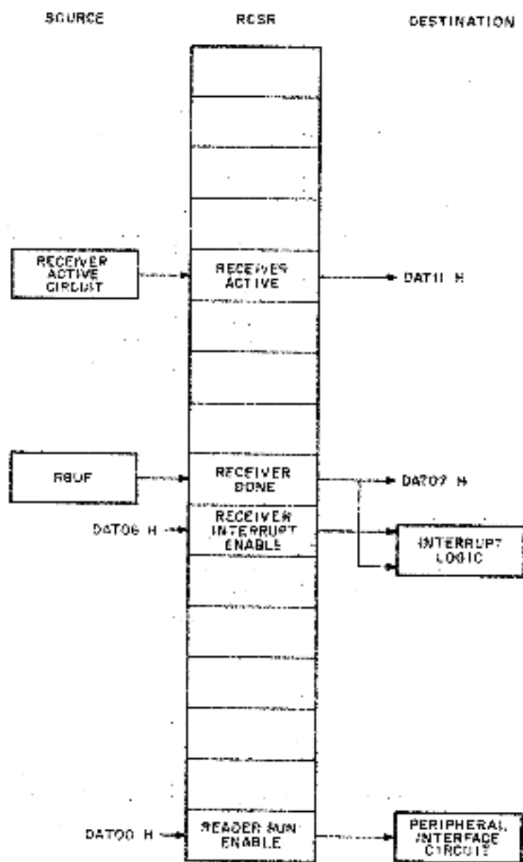
Figure 5-7 DLV11-F RCSR Data Flow
