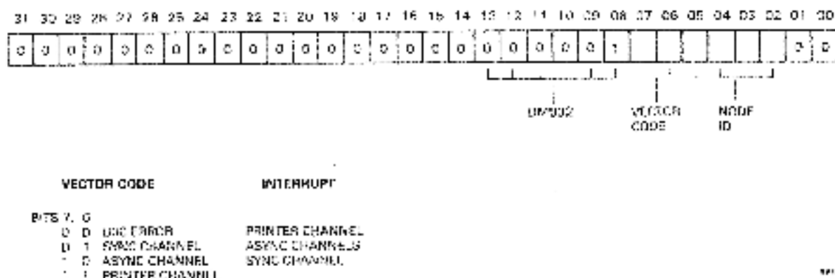
Figure 3-3 DMB32 Interrupt Vectors
