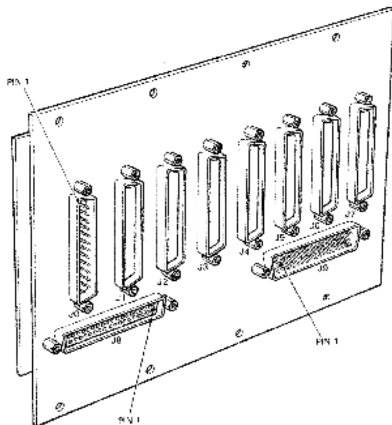
Figure 2-4 H3033 Distribution Panel (Front View)
