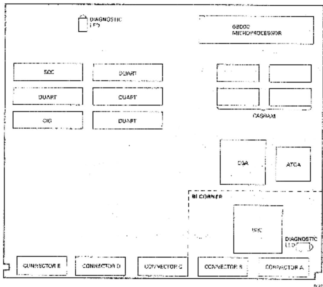
Figure 1-3 T1012 Module
