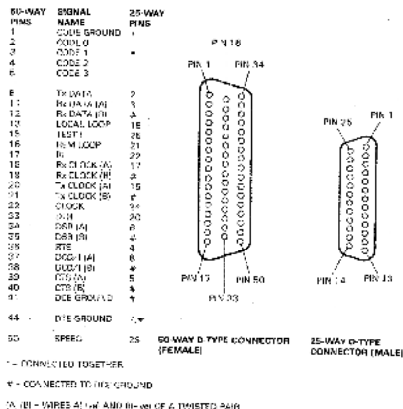
Figure 2-7 BC19D-02 (17-01110-01) Adapter Cable Detail
