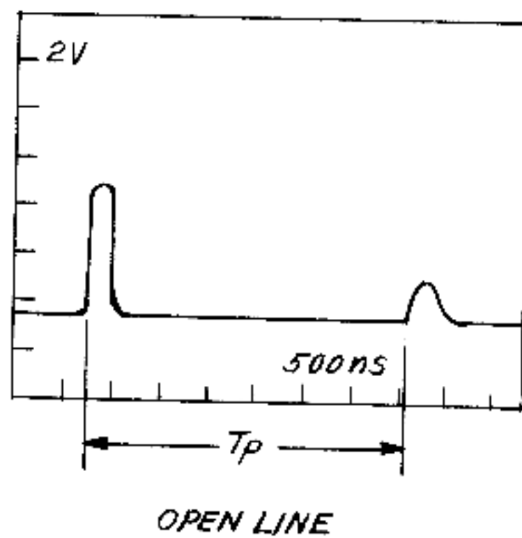
Figure 2-2 Signal Reflections from a Line Fault
