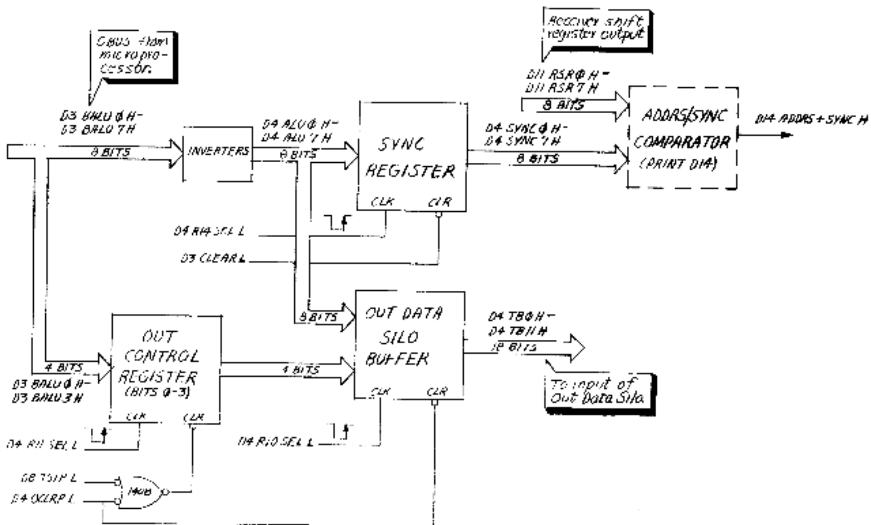
Figure 4-9 Block Diagram of OBUS and Associated Logic
