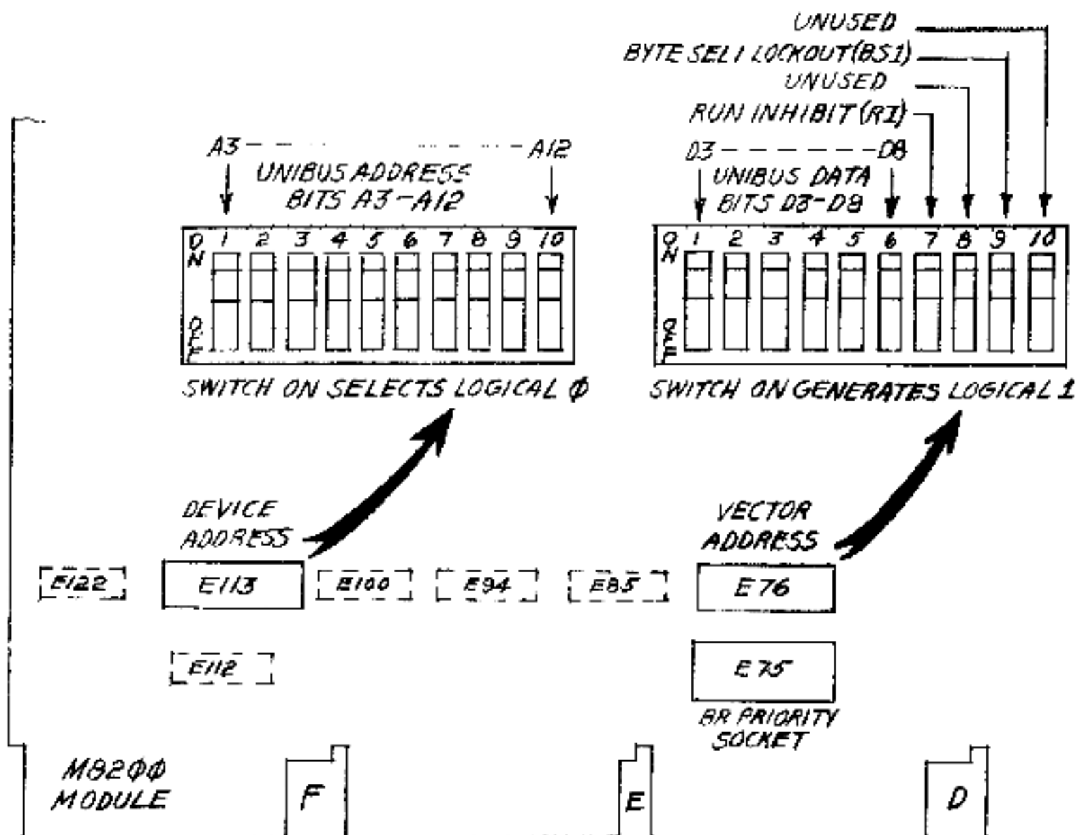
Figure 2-1 Microprocessor Device and Vector Address Switches
