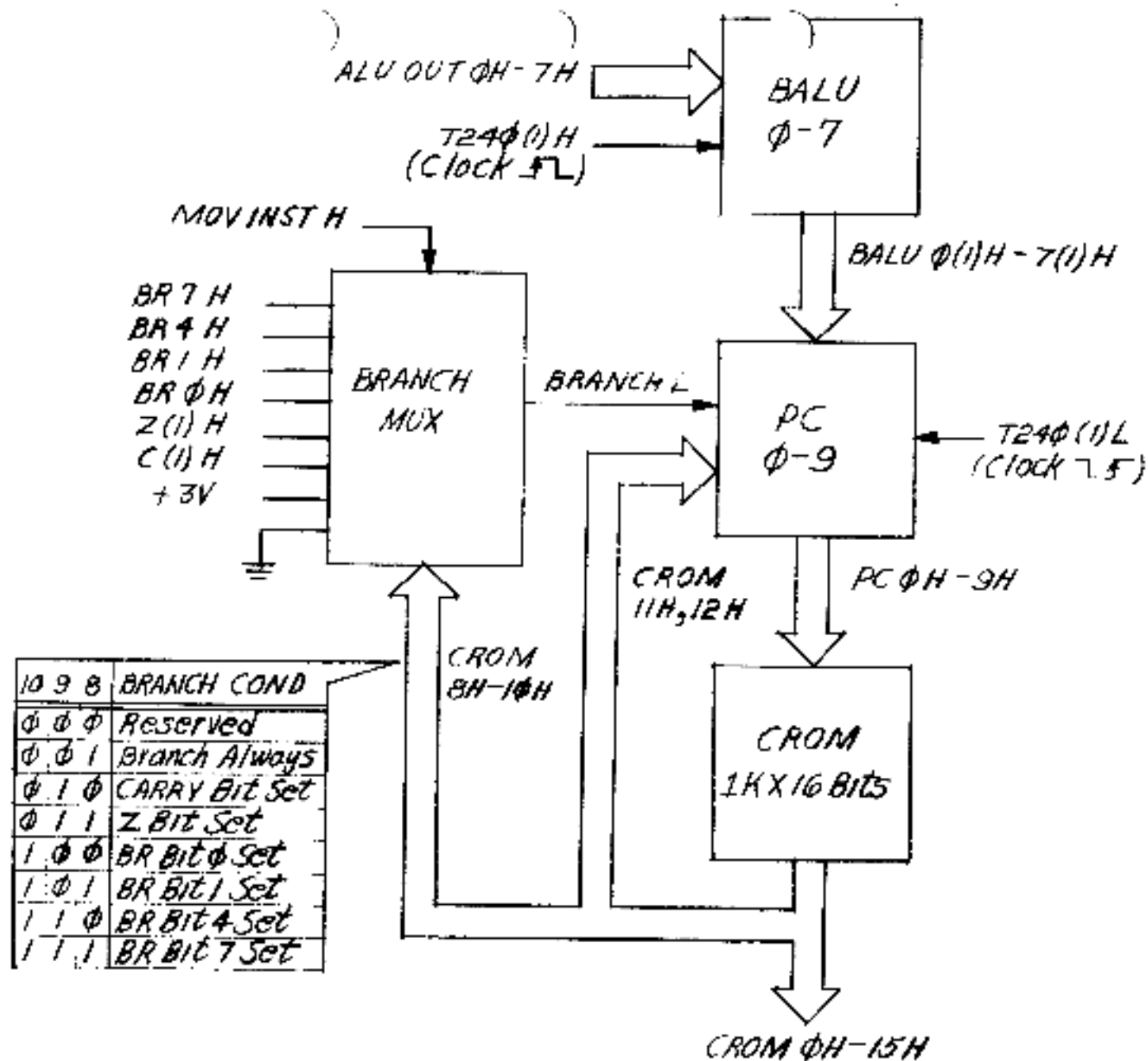
Figure 4-5 Block Diagram of Program Counter Control Logic
