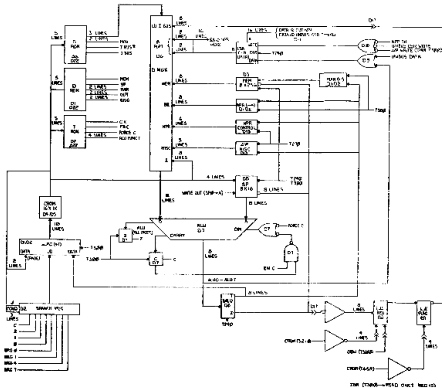
Figure 4-1 Microprocessor Block Diagram
