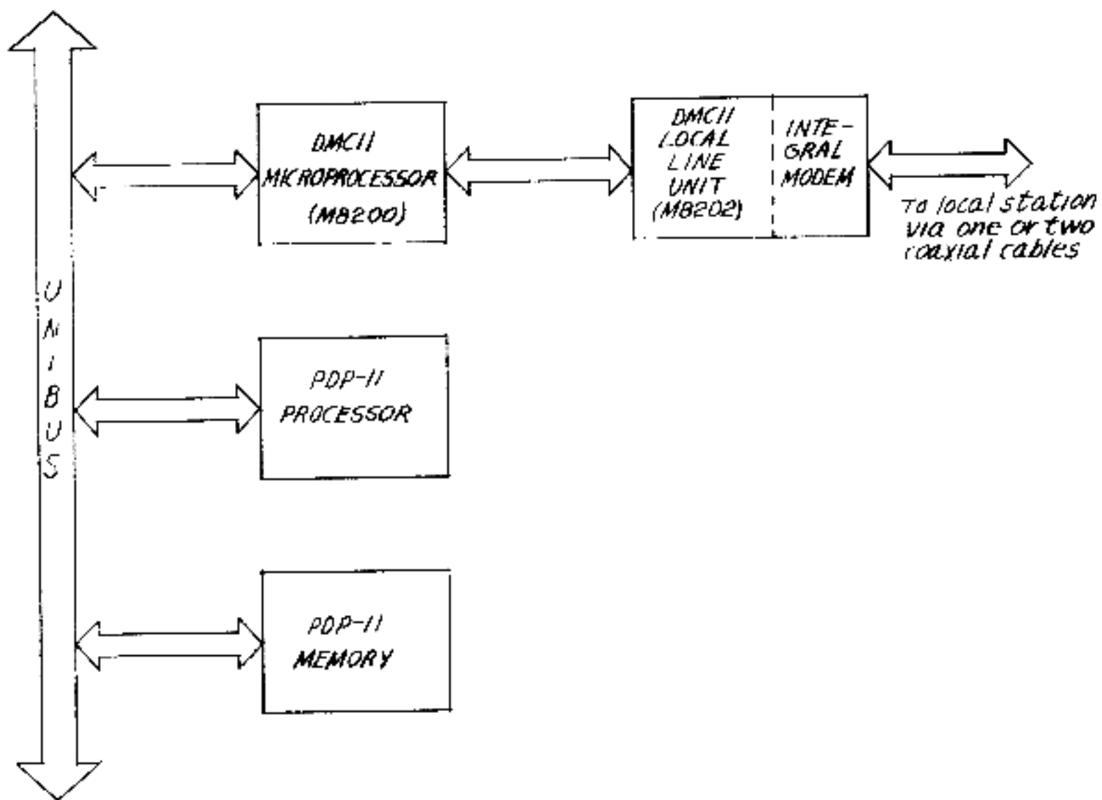
Figure 1-2 PDC11 Local Line Unit Interface
