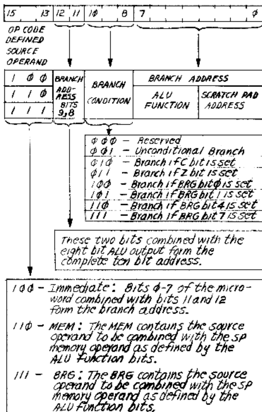
Figure 4-3 Branch Microinstruction Word Format
