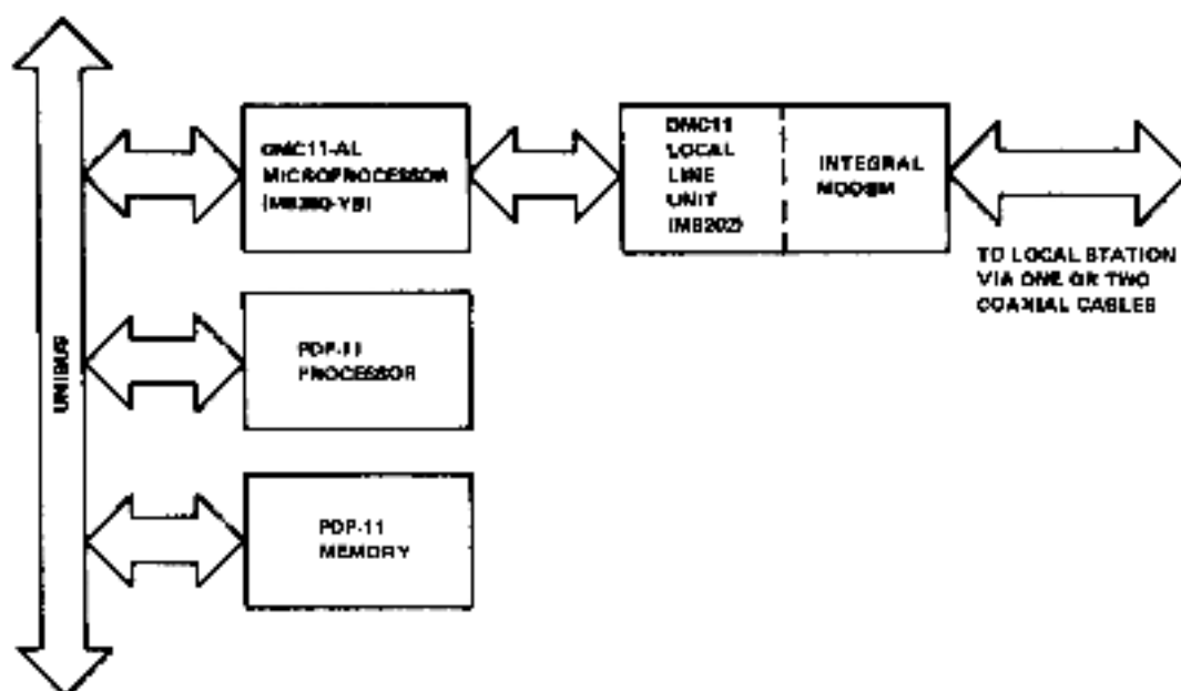
Figure 1-2 DMC11 Local Line Unit Interface
