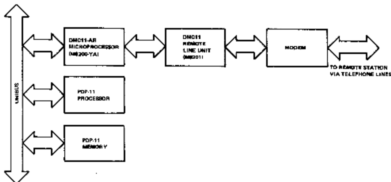
Figure I-1 DMC11 Remote Line Unit Interface
