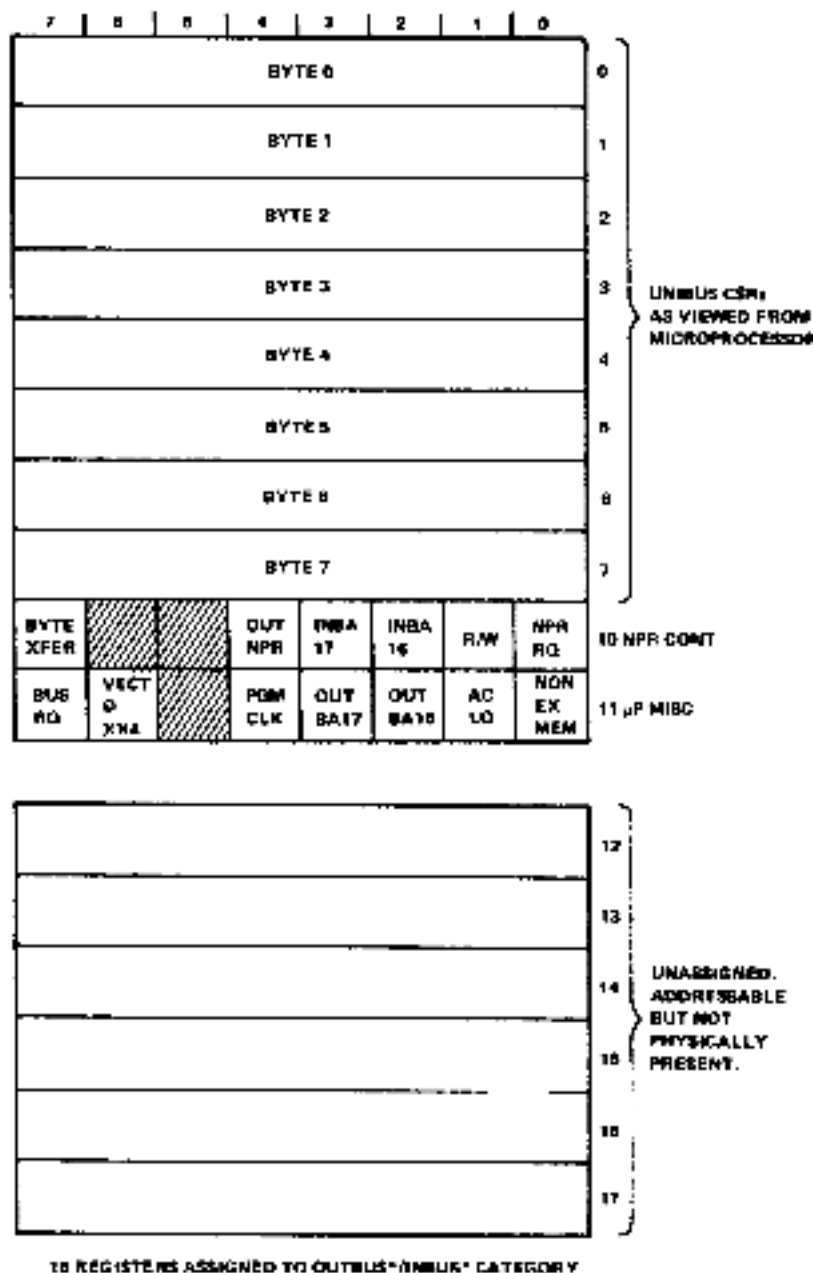
Figure 3-2 Microprocessor Registers
