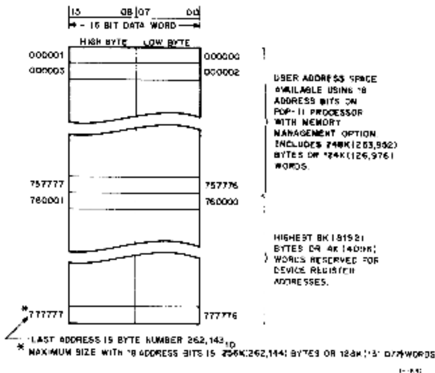
Figure A-1 Memory Organization for Maximum Size Using 18 Address Bits
