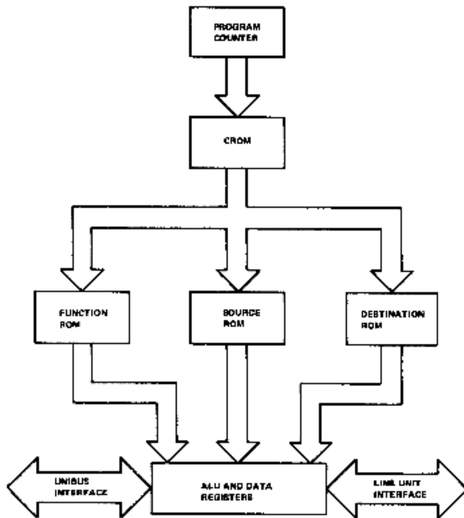
Figure 1-3 Microprocessor Simplified Block Diagram
