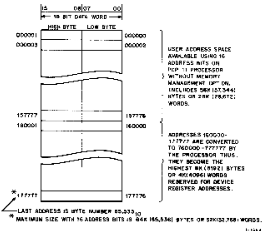
Figure A-2 Memory Organization for Maximum Size Using 16 Address Bits
