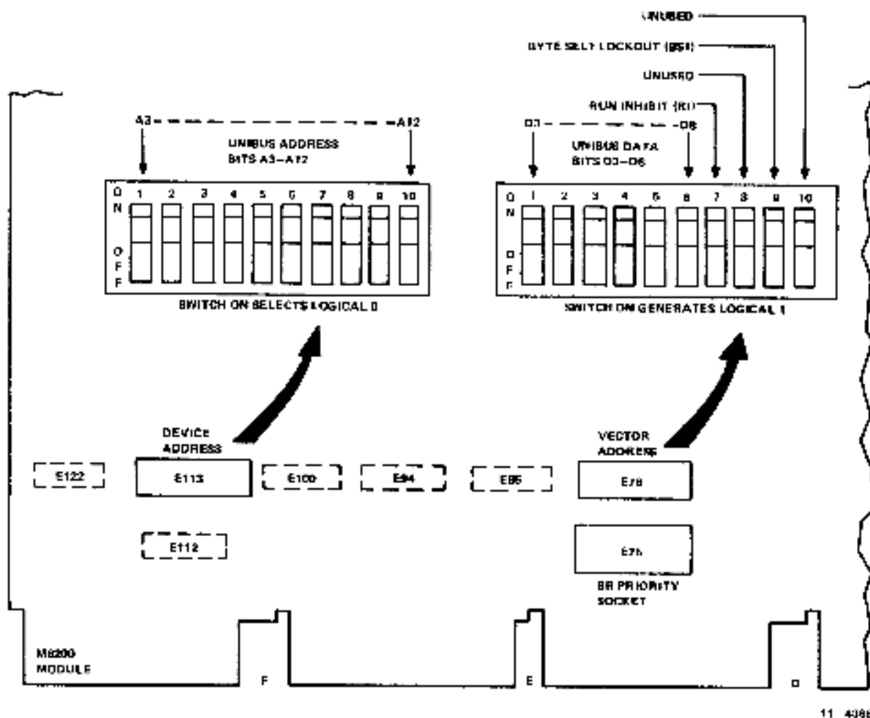
Figure 2-1 Microprocessor Device and Vector Address Switches
