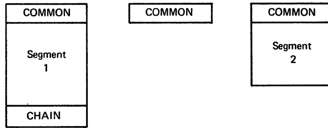
Figure 8-2 CHAIN with COMMON
