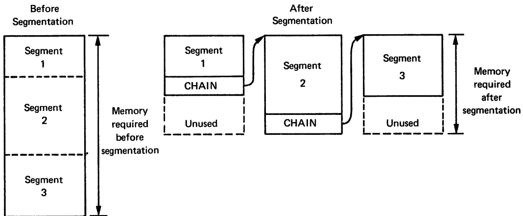
Figure 8-1 Segmenting a Program with the CHAIN Statement
