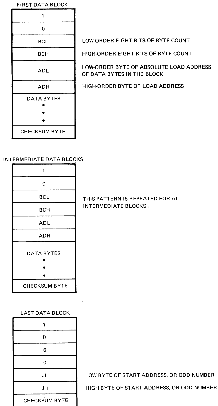
Figure 8–39: Absolute Binary Format (LDA)
