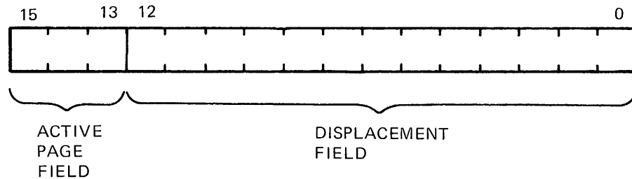
Figure 4-17: Virtual Address
