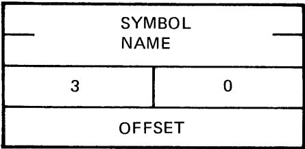
Figure 8–9: Transfer Address Entry Format (Entry Type 3)
