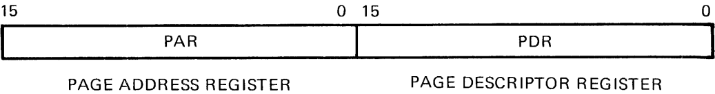
Figure 4–13: Active Page Register (APR)
