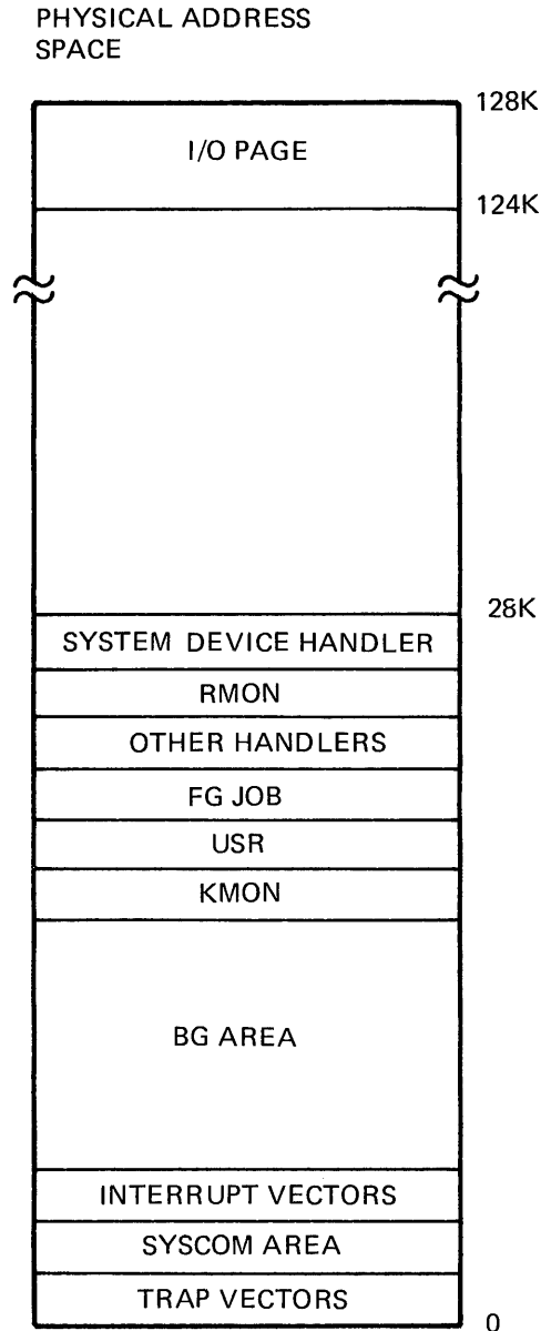
Figure 4–22: XM System Memory Layout
