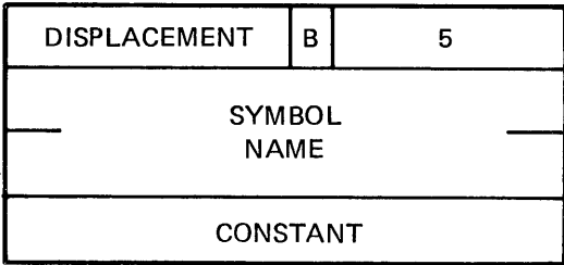
Figure 8–21: Global Additive Relocation (Entry Type 5)
