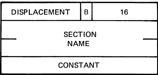
Figure 8–29: P-sect Additive Displaced Relocation (Entry Type 16)
