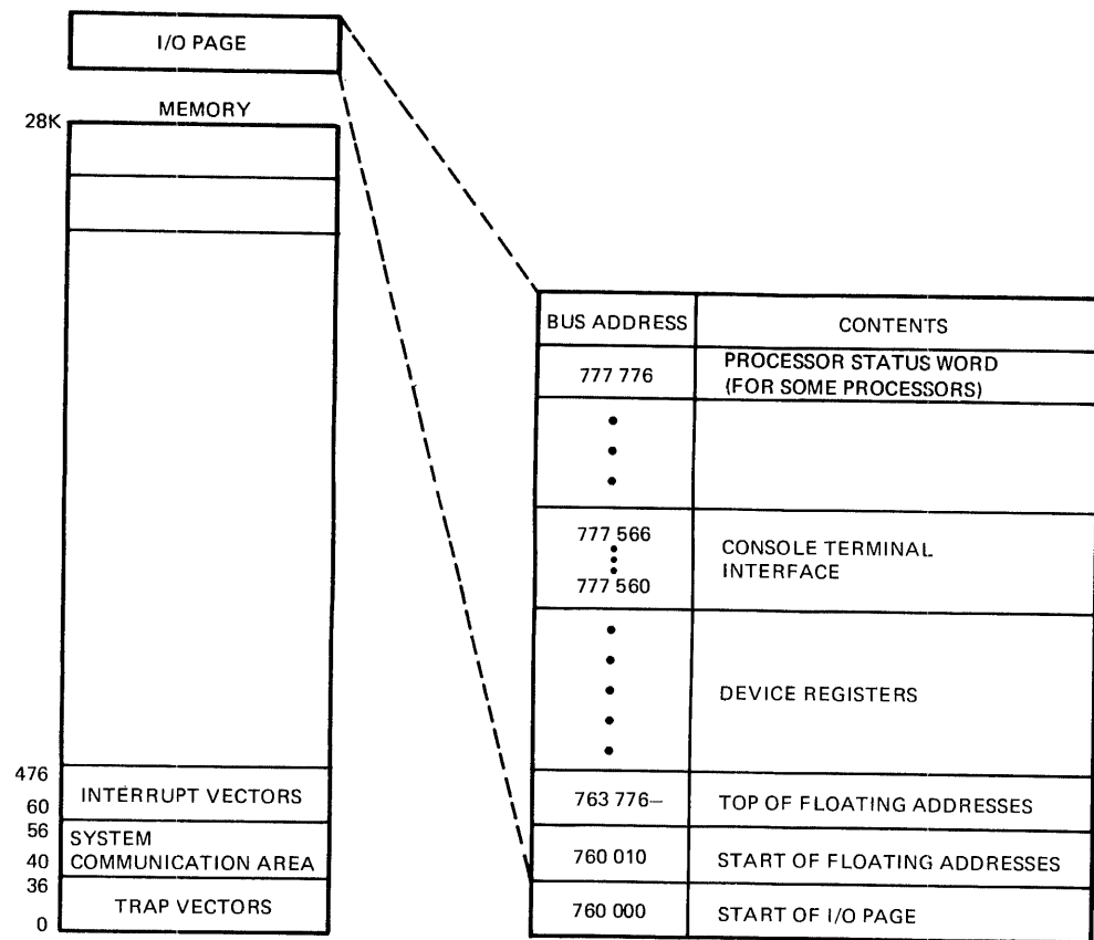
Figure 2-5: I/O Page
