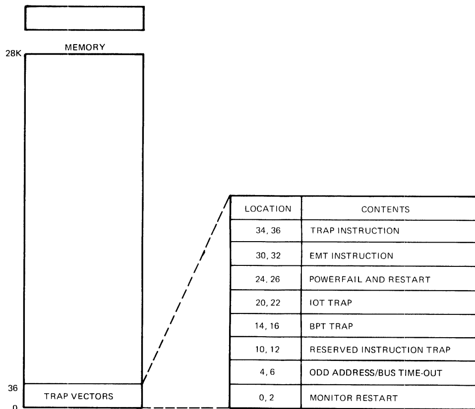
Figure 2-1: Trap Vector Area
