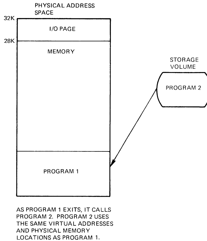
Figure 4–4: Overlaying
