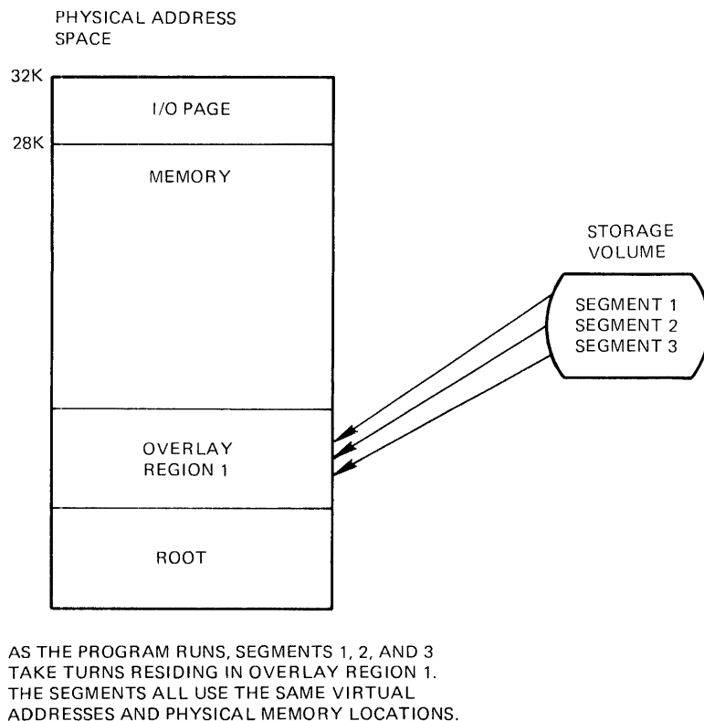
Figure 4–4: Overlaying
