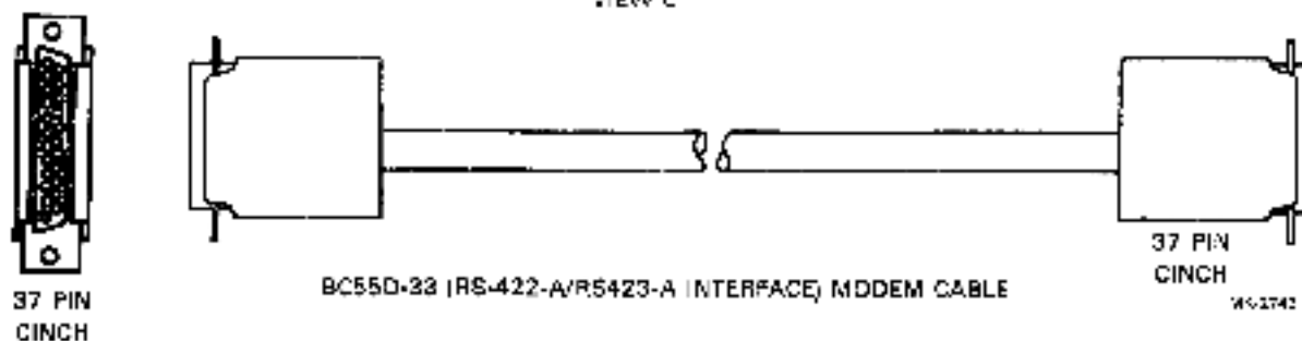
Figure 2-9 DMV11 Cable Drawings (Sheet 1 of 3)
