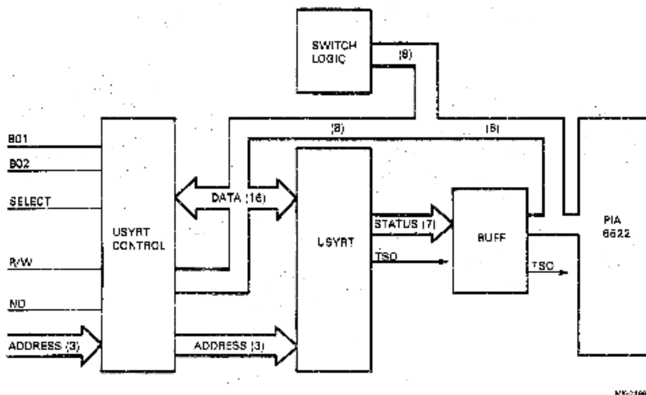
Figure 6-3 I/O Data Bus
