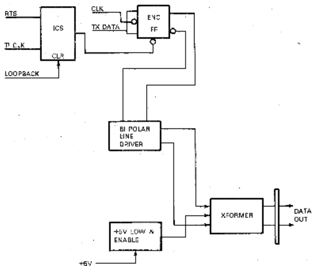
Figure 6-8 Integral Modem Transmitter
