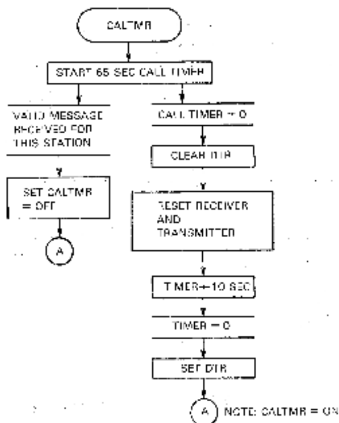
Figure D-7 Modern Control (Call Timer)
