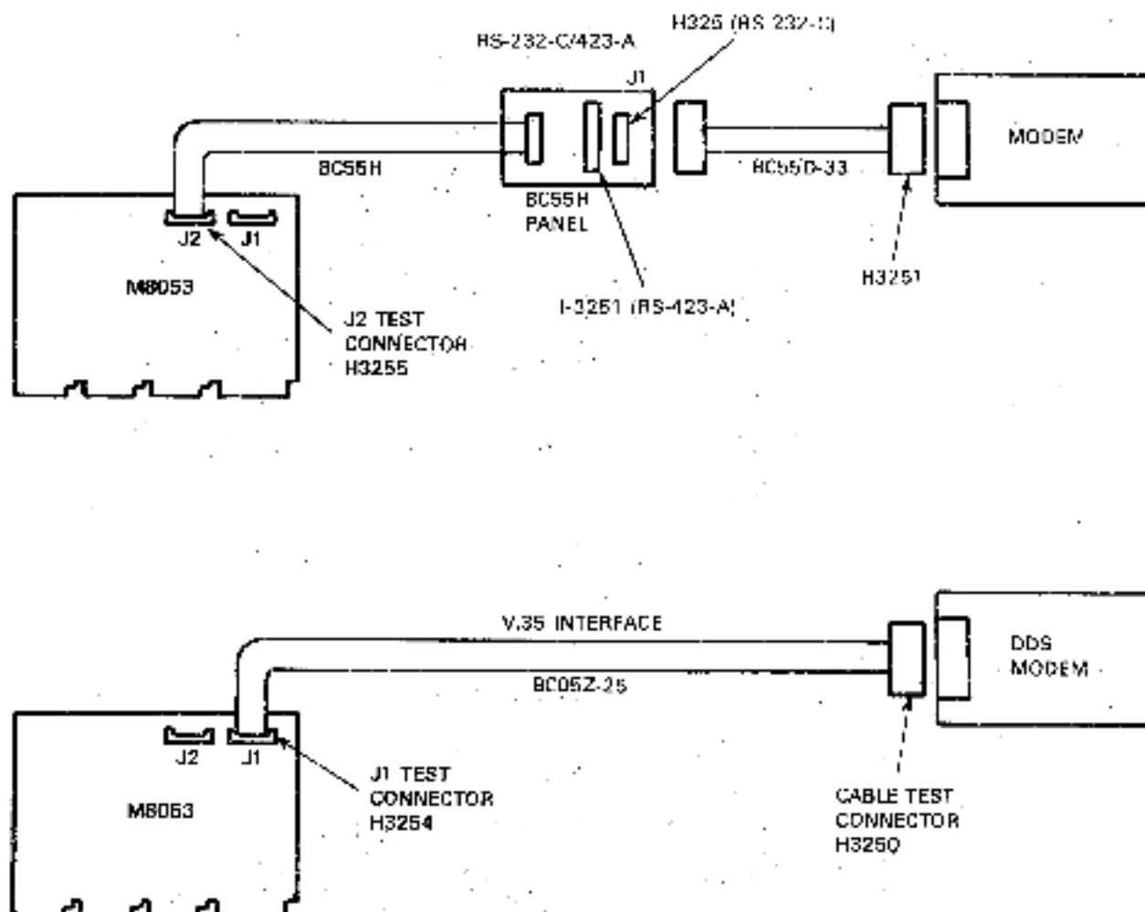
Figure 2-10 DMV11 Remote System Cabling Diagram
