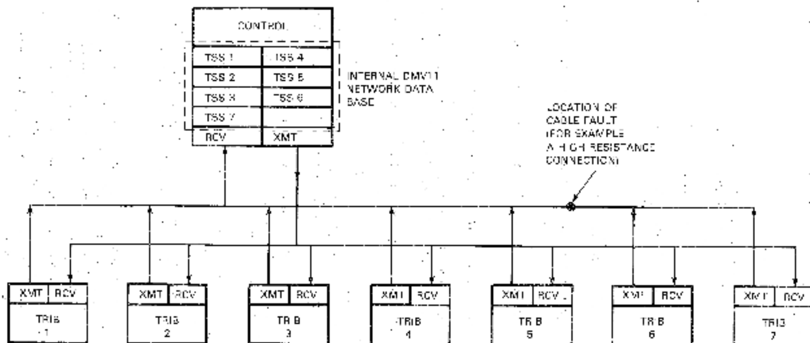
Figure 7-4 Full-Duplex Seven Tributary Multipoint Network
