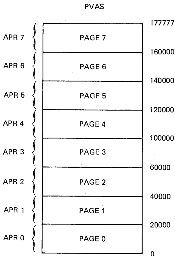
Figure 11–8: Program Virtual Address Space
