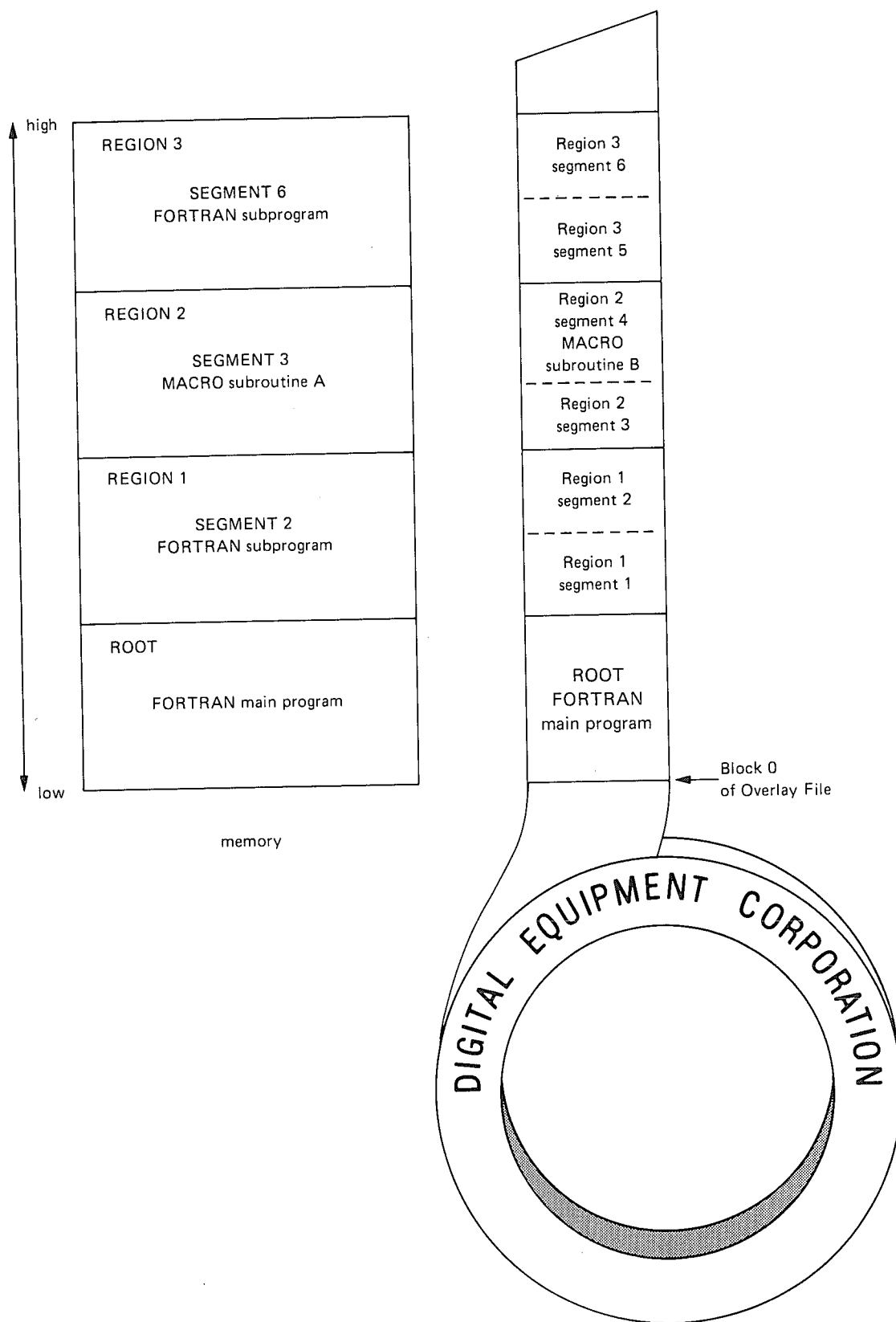
Figure 11-3: Sample Overlay Structure for a FORTRAN Program
