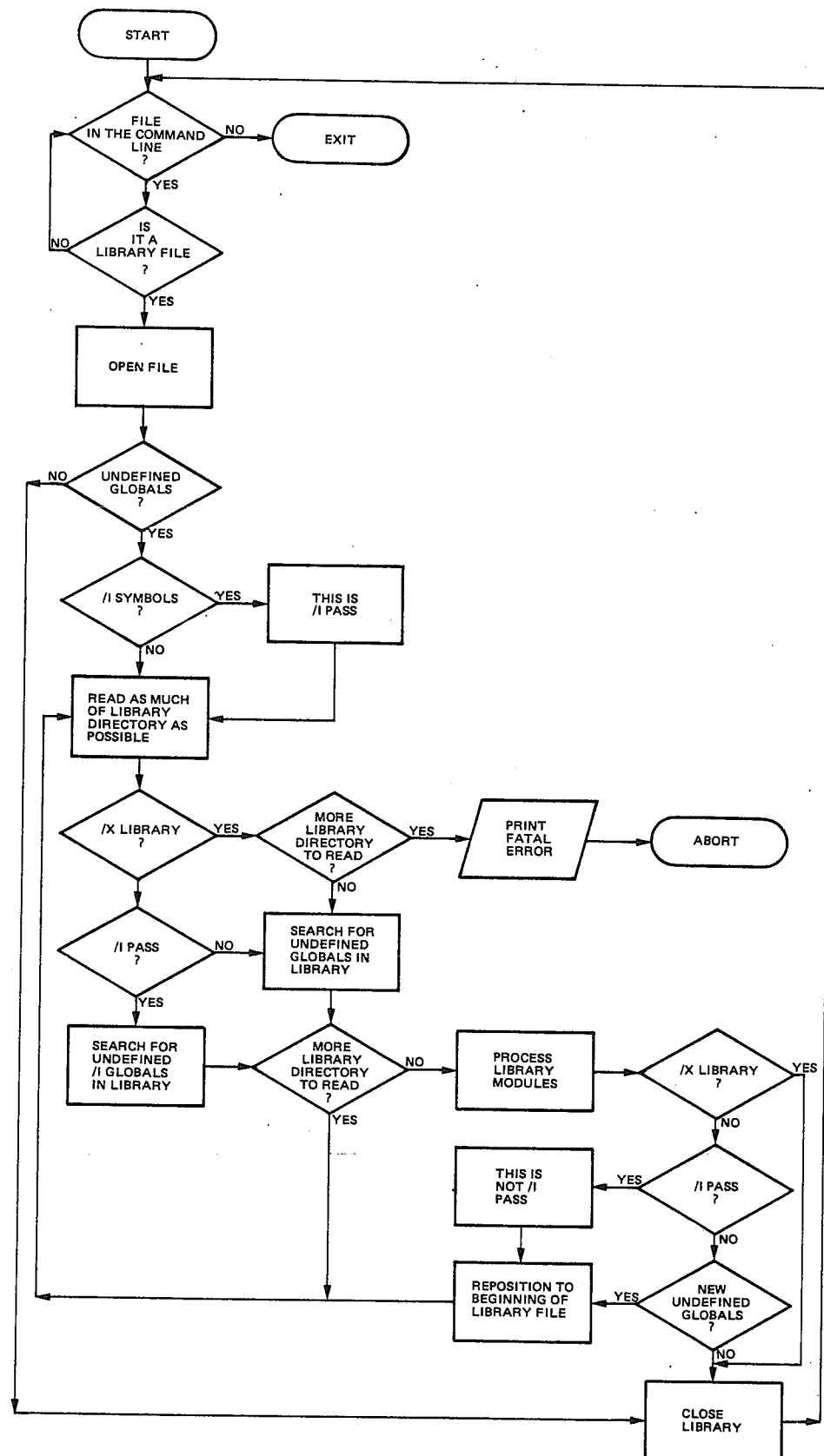
Figure 11-1: Library Searches
