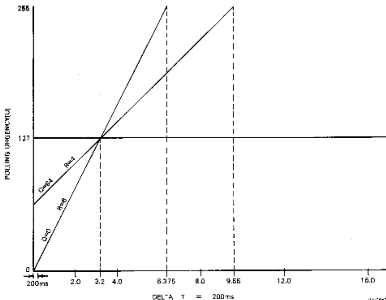
Figure S-2 Relationship Between Polling Parameters Q, R, and the Minimum Polling Interval
