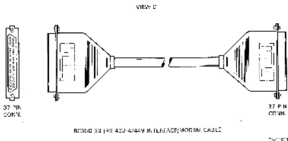
Figure 2-9 DMV11 Cable Drawings (Sheet 1 of 3)
