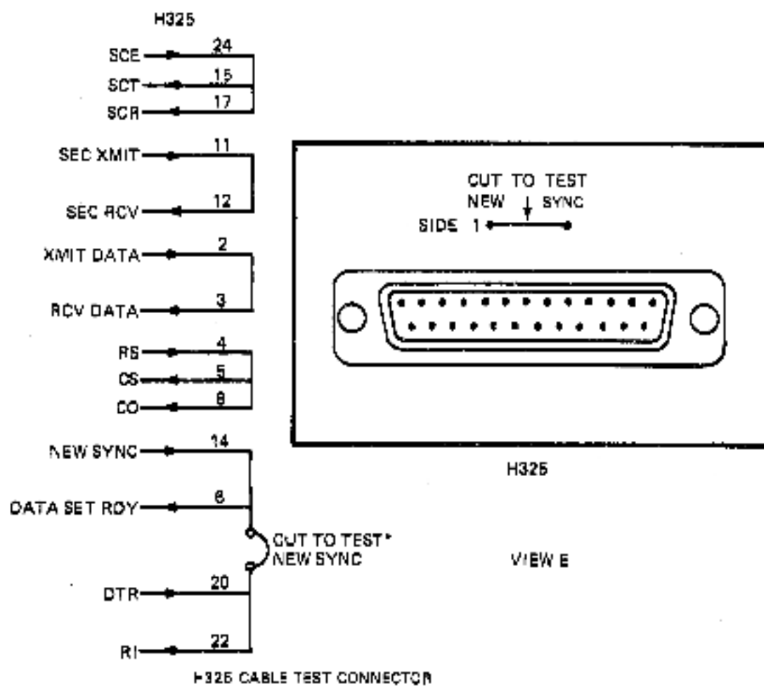
Figure 2-8 DMV:1 Test Connectors (Sheet 4 of 4)
