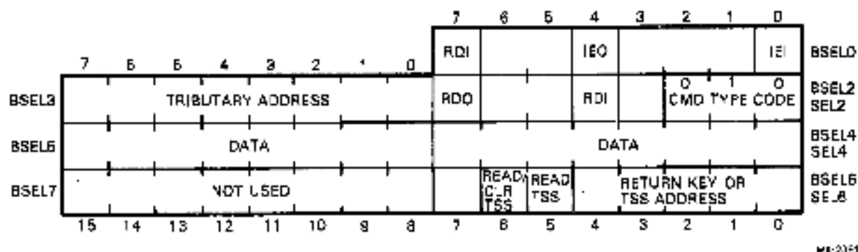
Figure 3-10 Information Response Format
