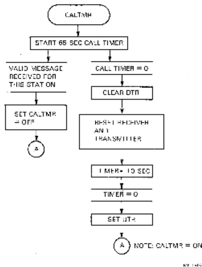
Figure D-7 Modem Control (Cal. Timer)
