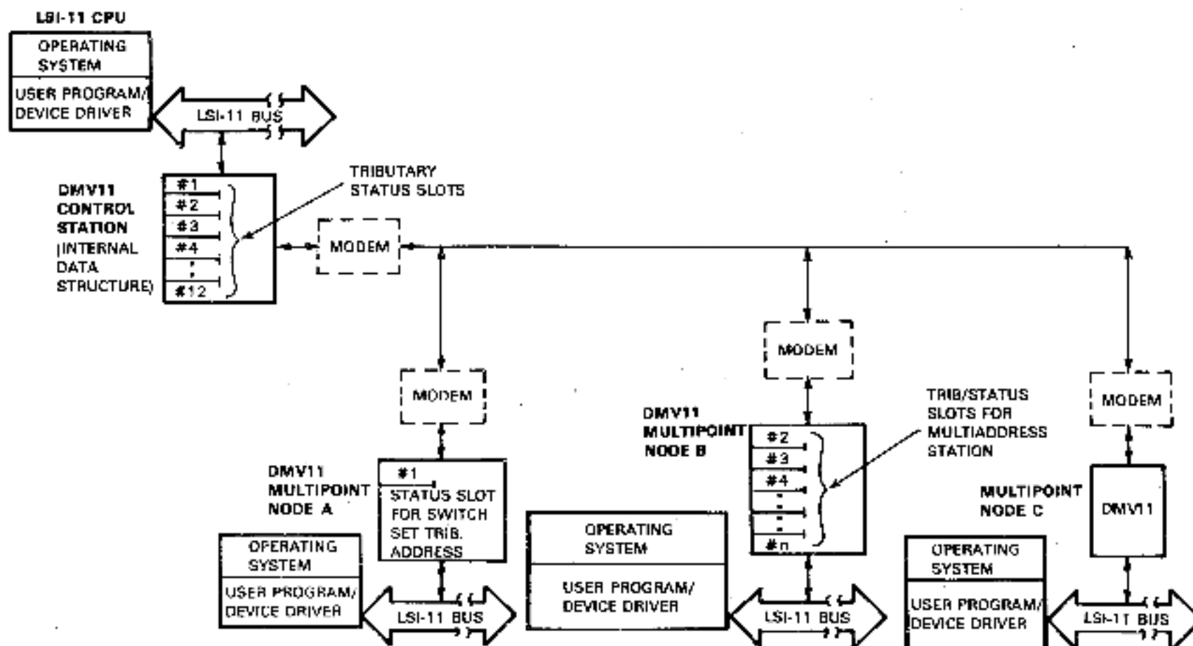
Figure 1-2 DMV11s Used in Multipoint Applications
