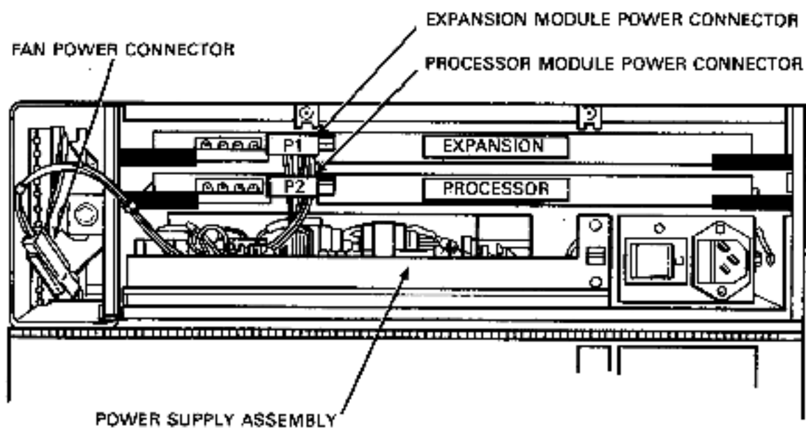
Figure 4-18 II3014 Power Supply Location
