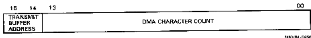
Figure 3-14 Indirect Register (IND.REG[3]<15:0>) Bit Map – Read/Write
