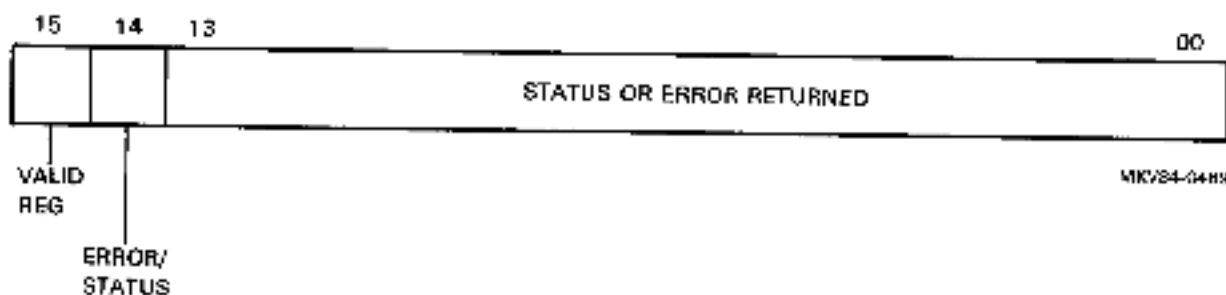
Figure 3-5 Diagnostic Control and Status Register DIAG.CSR<15:0> Bit Map – Read
