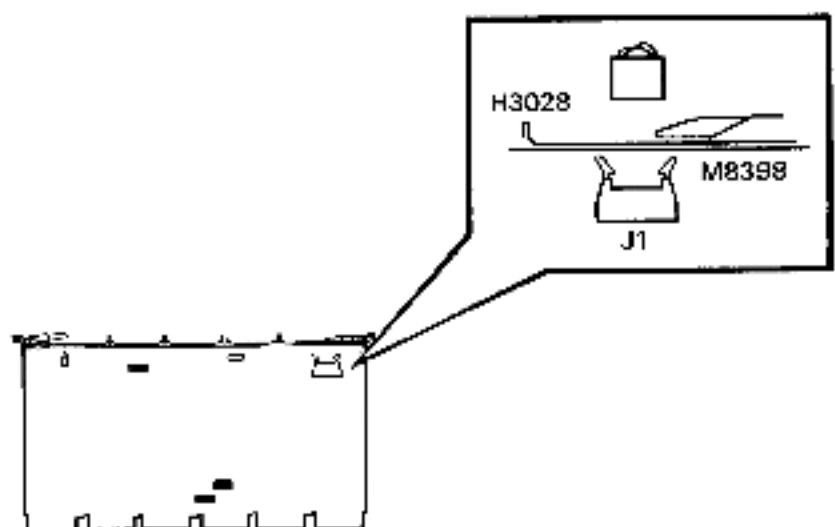
Figure 2-9 H3028 Loopback Connector Installed on M8398
