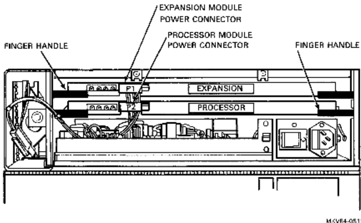
Figure 4-21 H3014 Expansion Module Location
