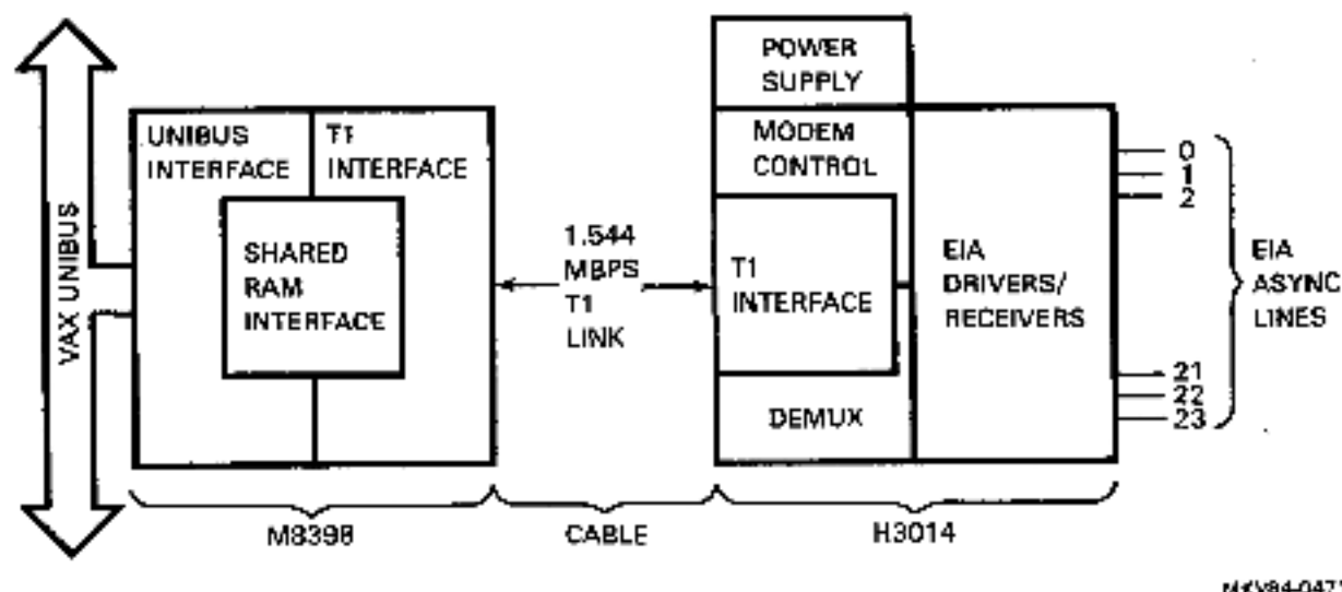
Figure 1-2 DMZ32 Functional Block Diagram
