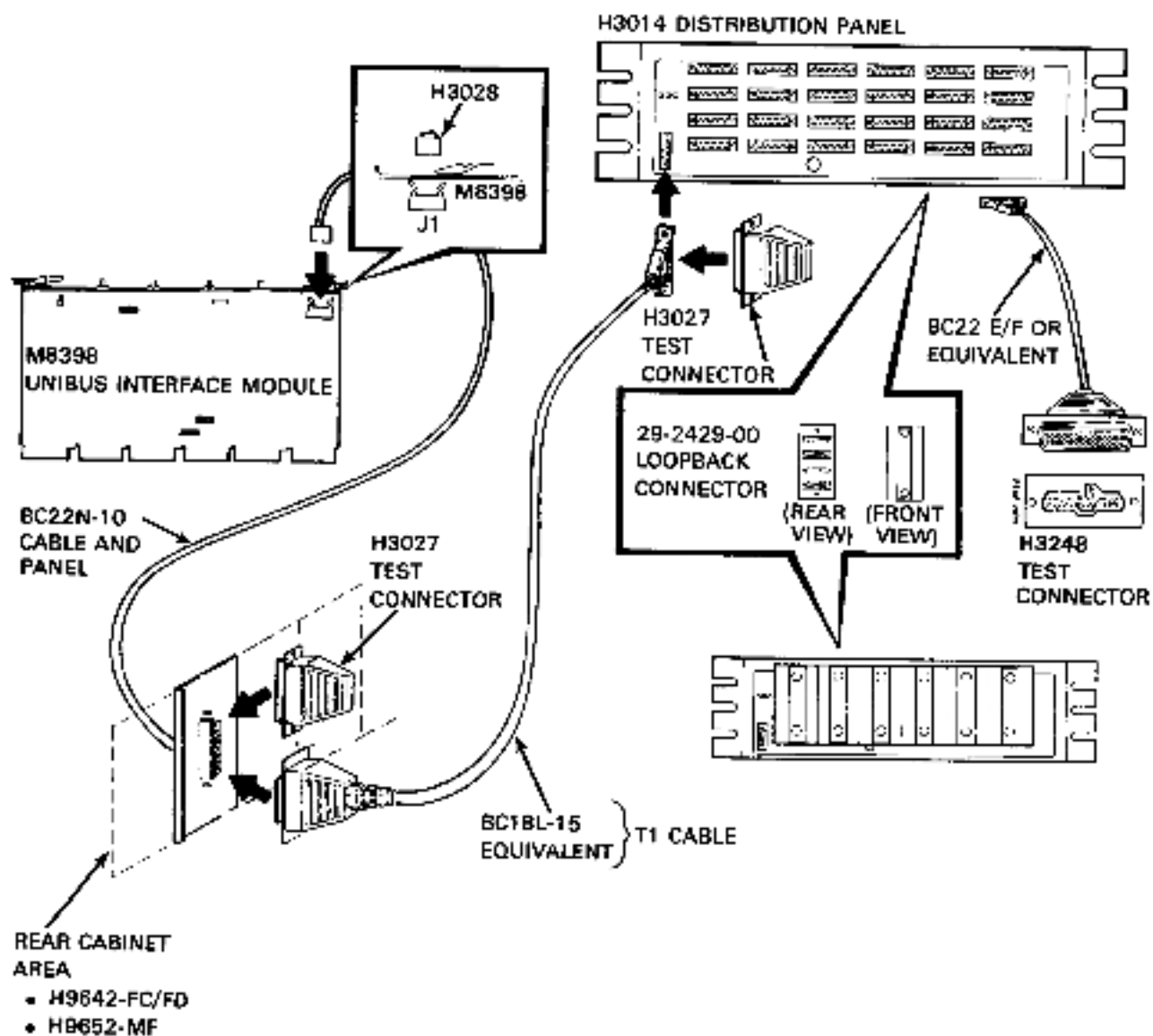
Figure 2-15 DMZ32 Installation Overview
