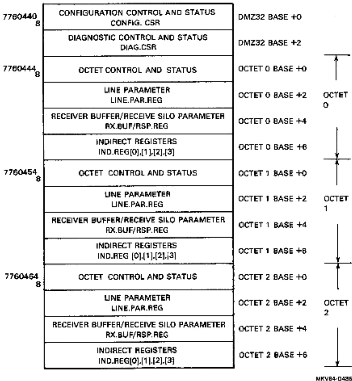
Figure 3-1 DMZ32 Word Allocation of Device Control/Status Registers
