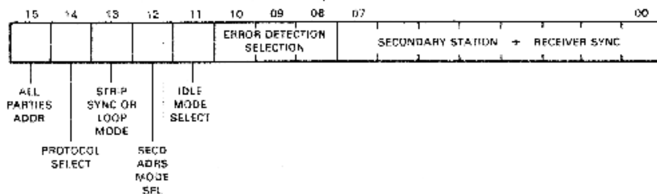
Figure 3-1 QMA DPV11 Register Configurations and Bit Assignments (Sheet 1 of 2)
