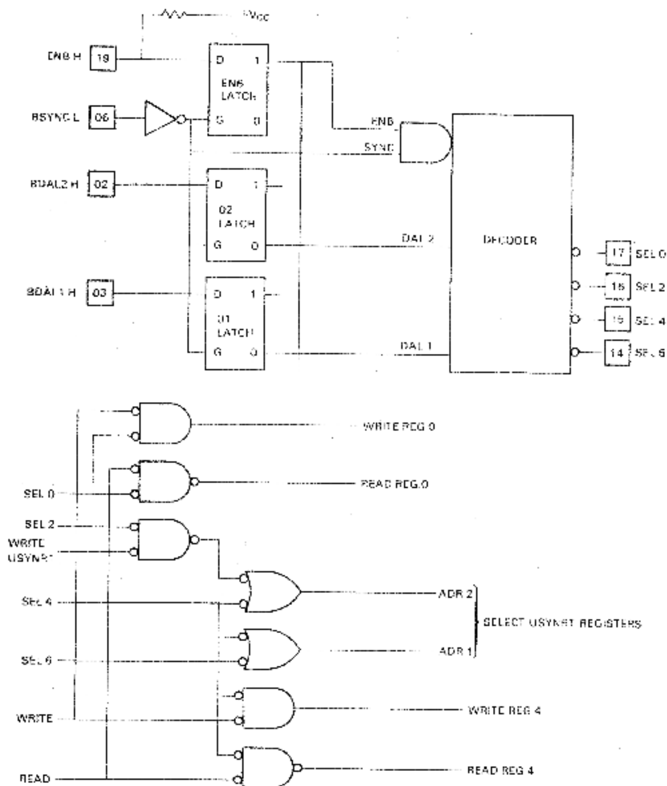
Figure 4-3 Register Decode
