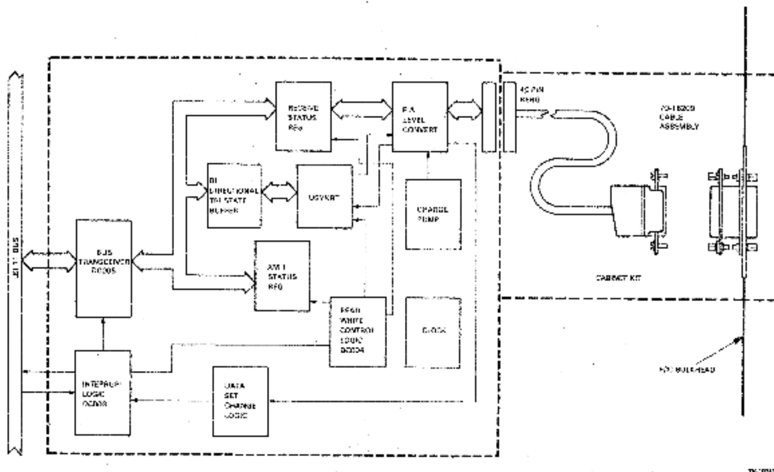
Figure 4-1 QMA DPV11 Block Diagram
