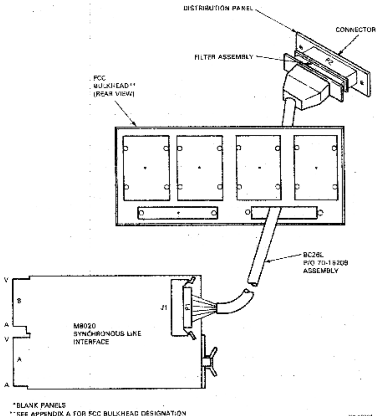
Figure 2-3 Distribution Panel Installation
