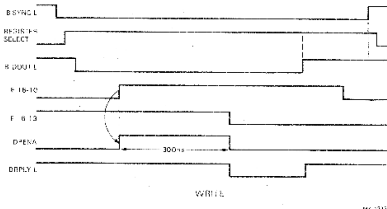
Figure 4-5 Timing for Write Operation
