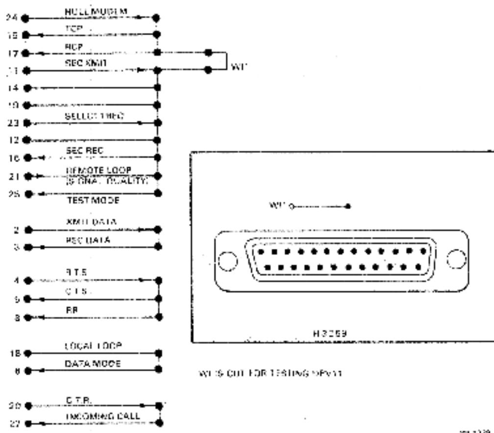
Figure 2-4 H3259 Turnaround Test Connector
