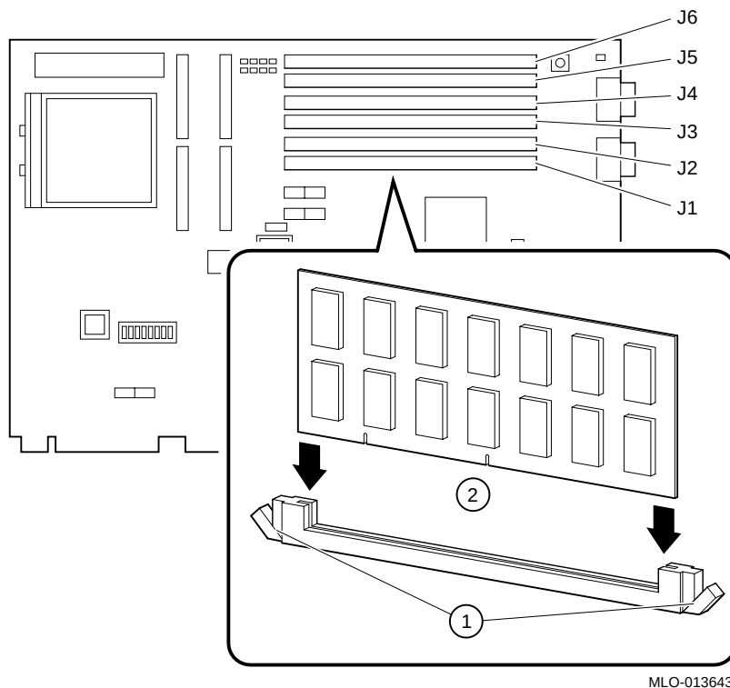
Figure 1-6 Installing the Memory
