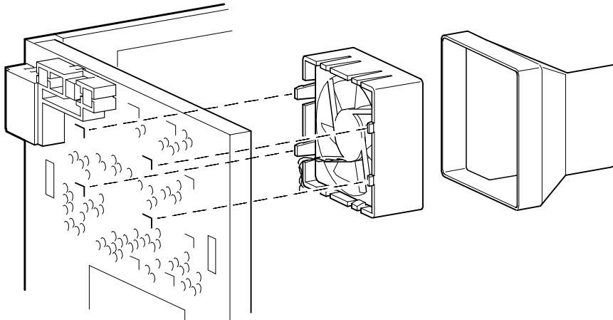
Figure 1-3 Removing Old Fan Pipe
