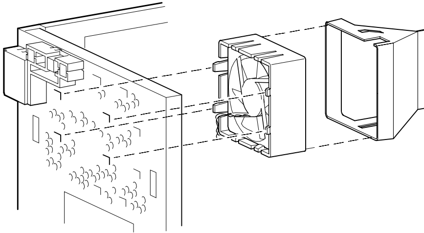
Figure 1-4 Installing the new Fan Pipe
