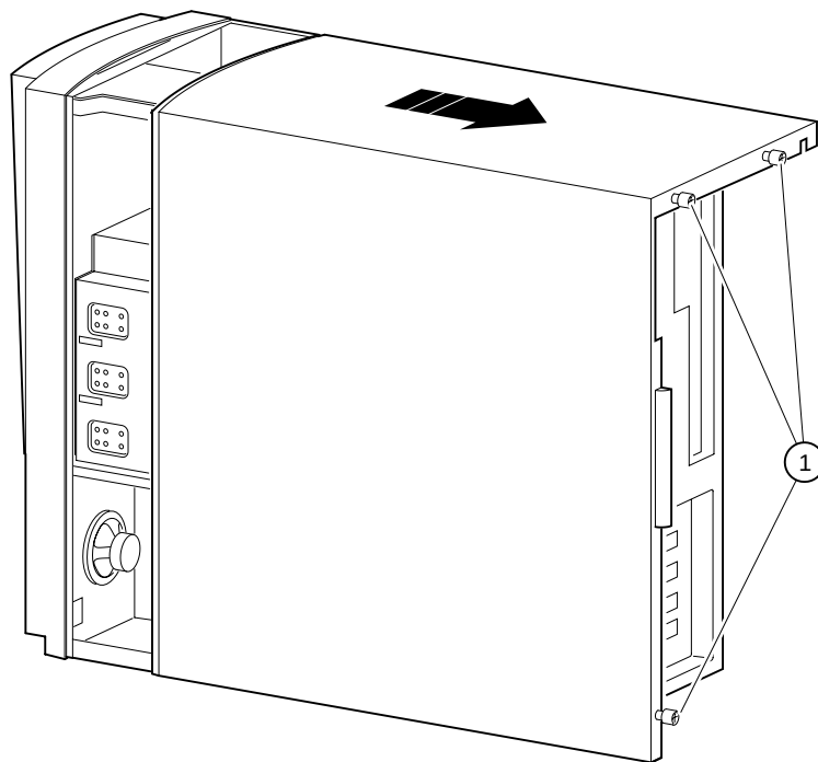
Figure 1-1 Unlocking and Removing the System Cover
