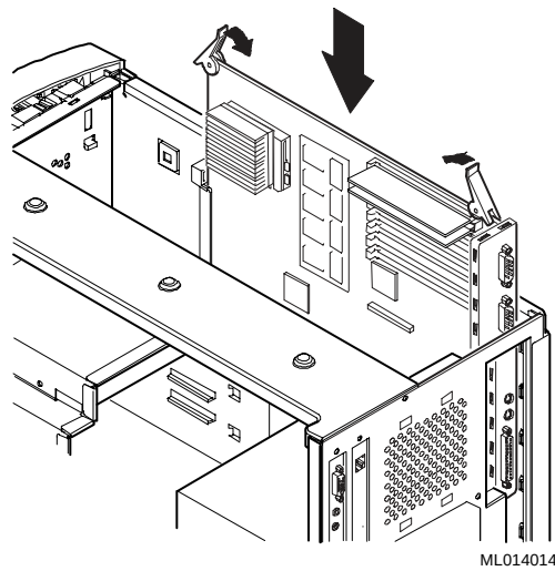
Figure 1-7 Installing the New MLB
