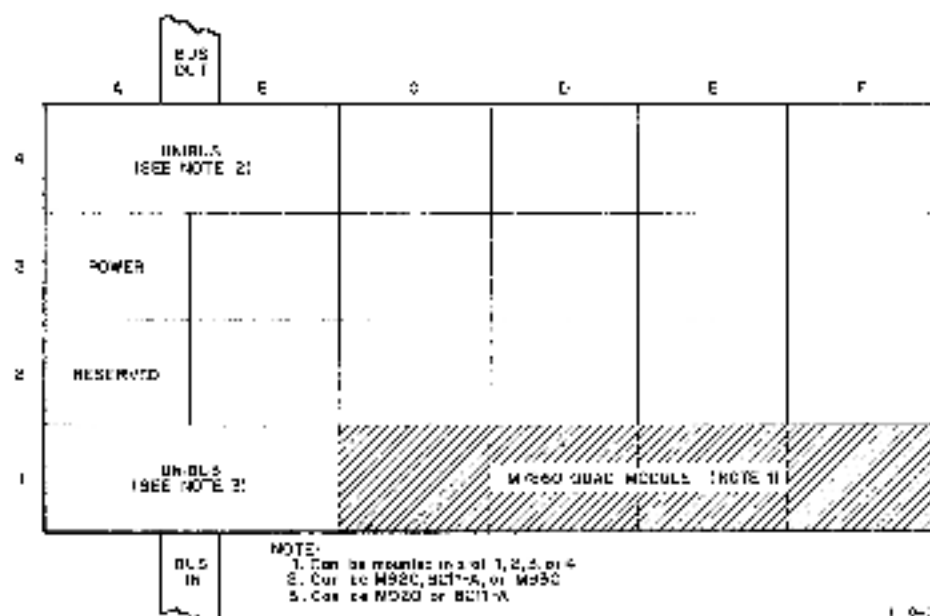
Figure 1-2. Typical M7960 Quad Module Mounting in a DD11-A.
