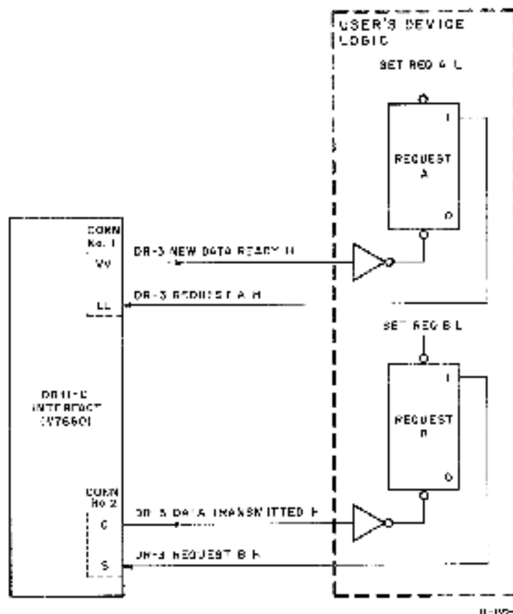
Figure 4-3 Request Line Control Logic
