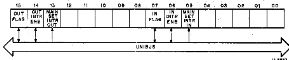
Figure 2-2 Status Register Data Flow (twrite/4read)
