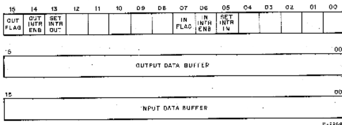
Figure 2-1 DR11-K Register Assignments
