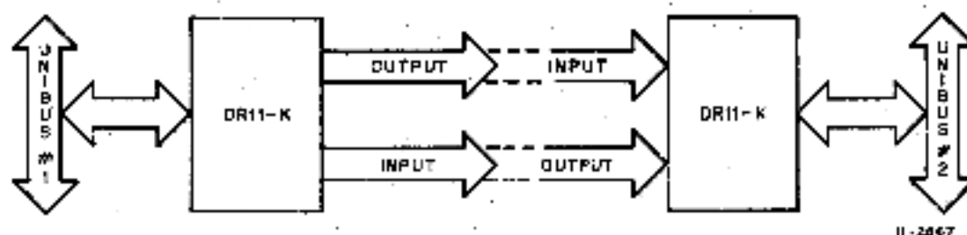
Figure 6-4 Block Diagram of Output Example 1
