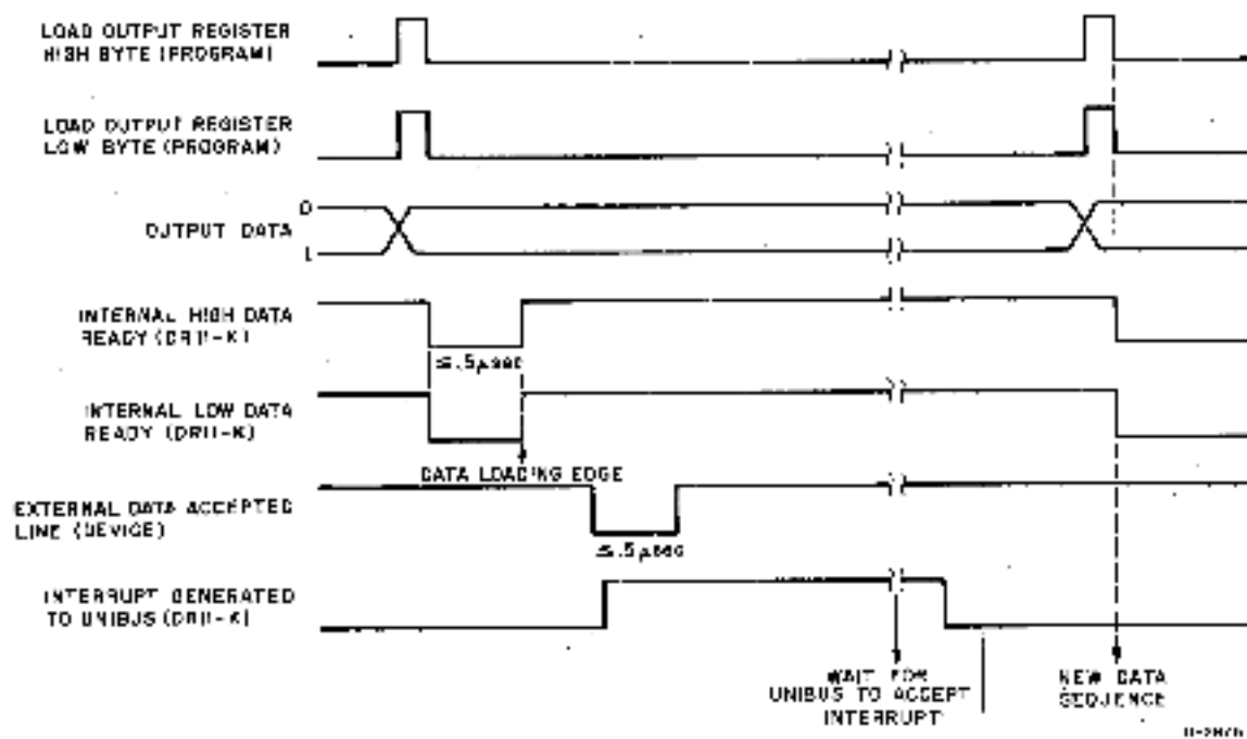
Figure 4-5 Data Output Timing Diagram
