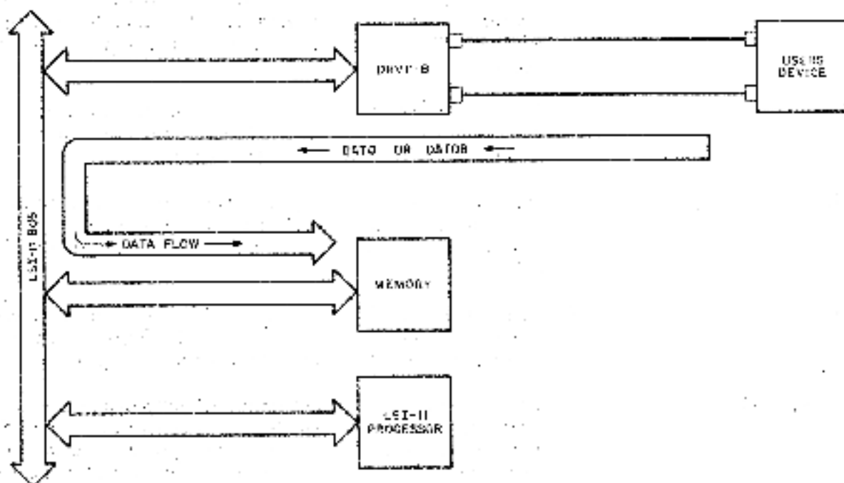
Figure 3-2 DMA DATO/DATOB Data Flow Diagram
