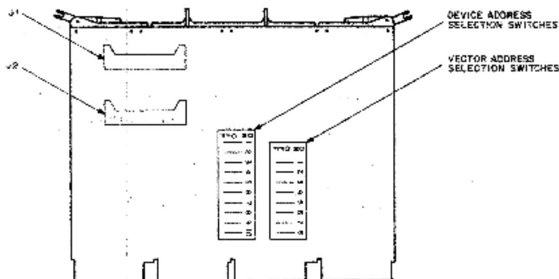
Figure 2-1 DRV11-B Connector and Switch Locations
