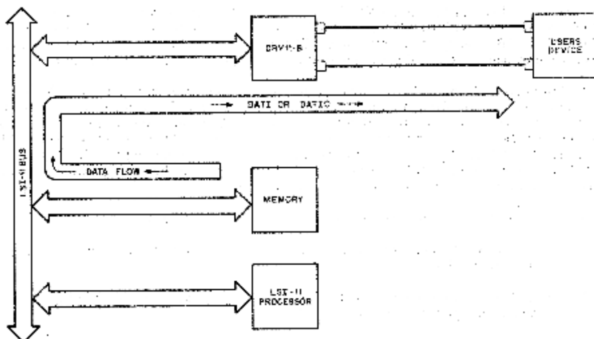
Figure 3-3 DMA DATI/DATIO Data Flow Diagram
