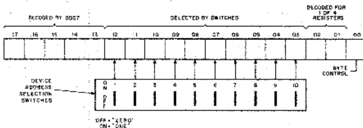
Figure 2-2 DRV11-B Device Address Select Format
