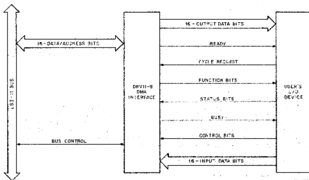
Figure 1-1 DRV11-B Simplified Interface Diagram
