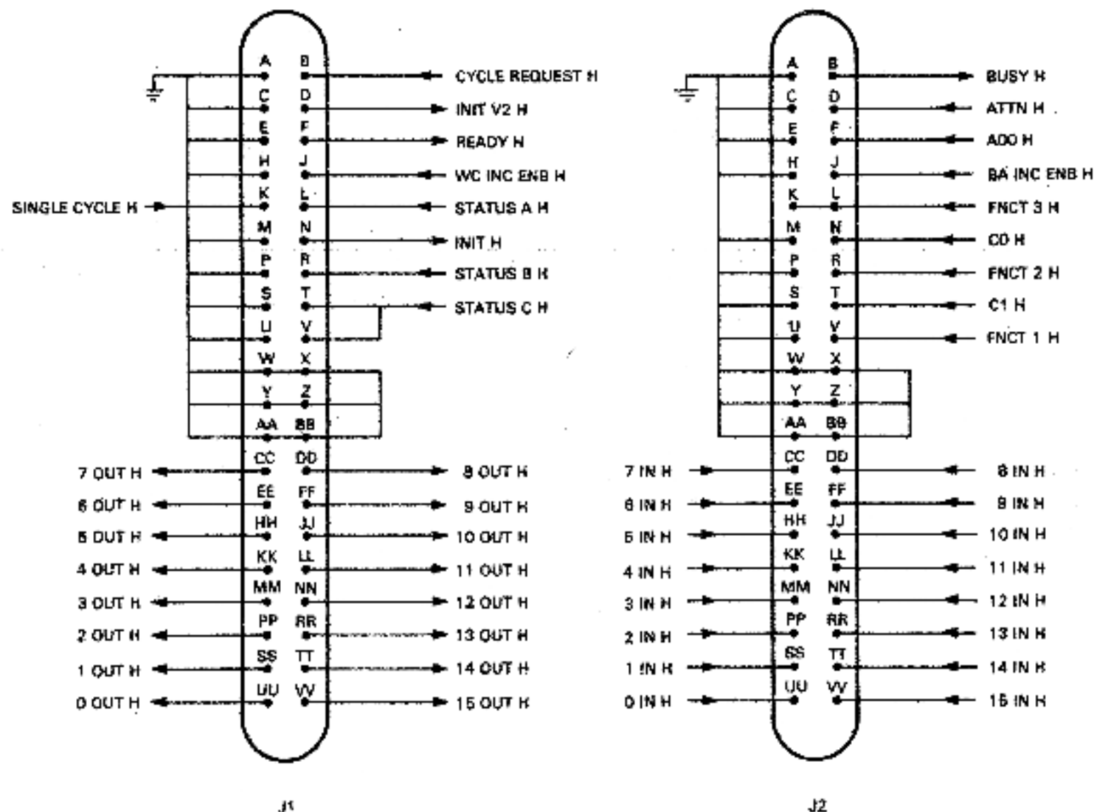
Figure 2-4 DRV11-WA Connector Pin Assignments
