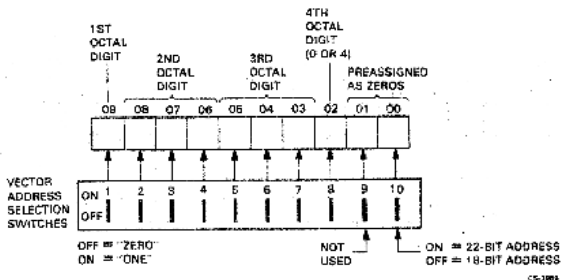
Figure 2-3 DRV11-WA Interrupt Vector Address Select Format
