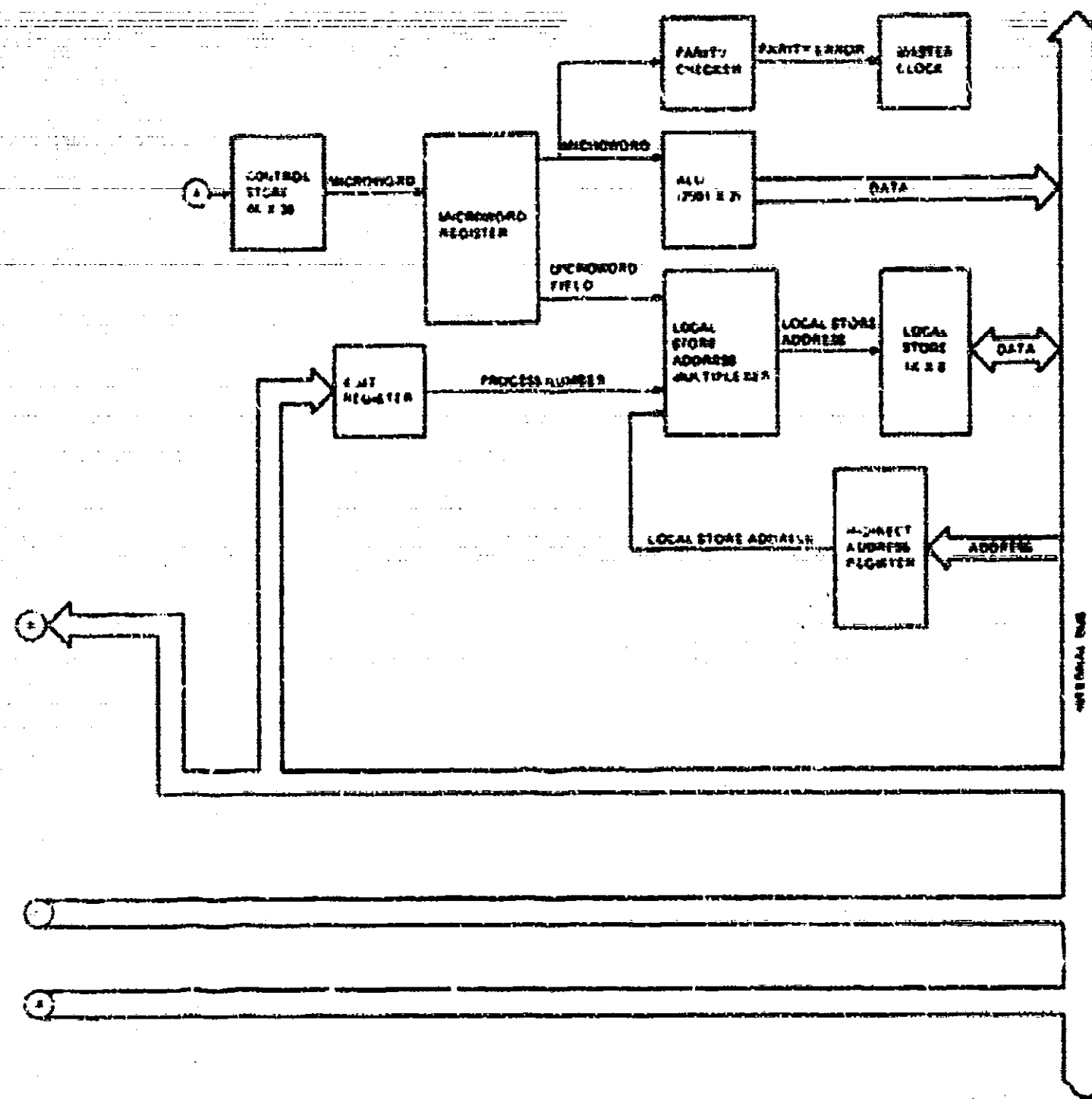
Figure 3-1 DMF32 Overview (Sheet 2 of 3)
