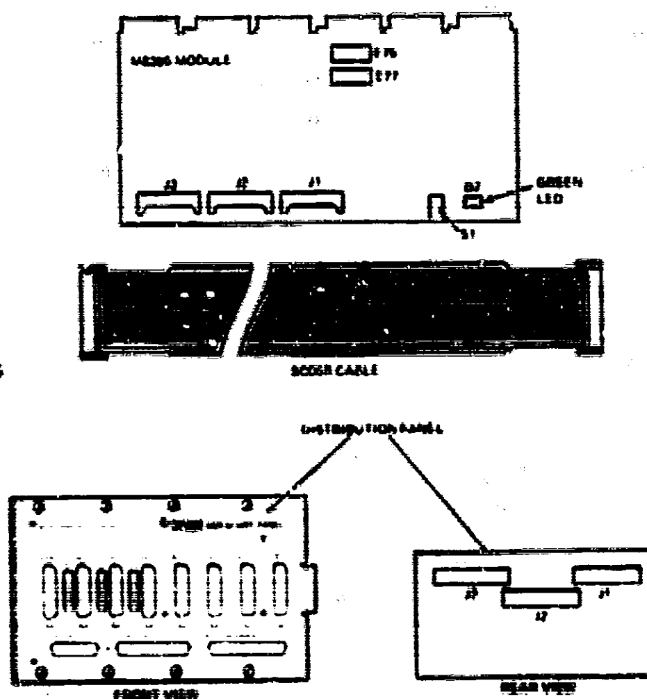
Figure 1-1 DMF32 Components
