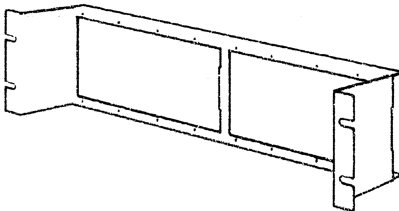
Figure A-3 119544-S1 Adapter Bracket
