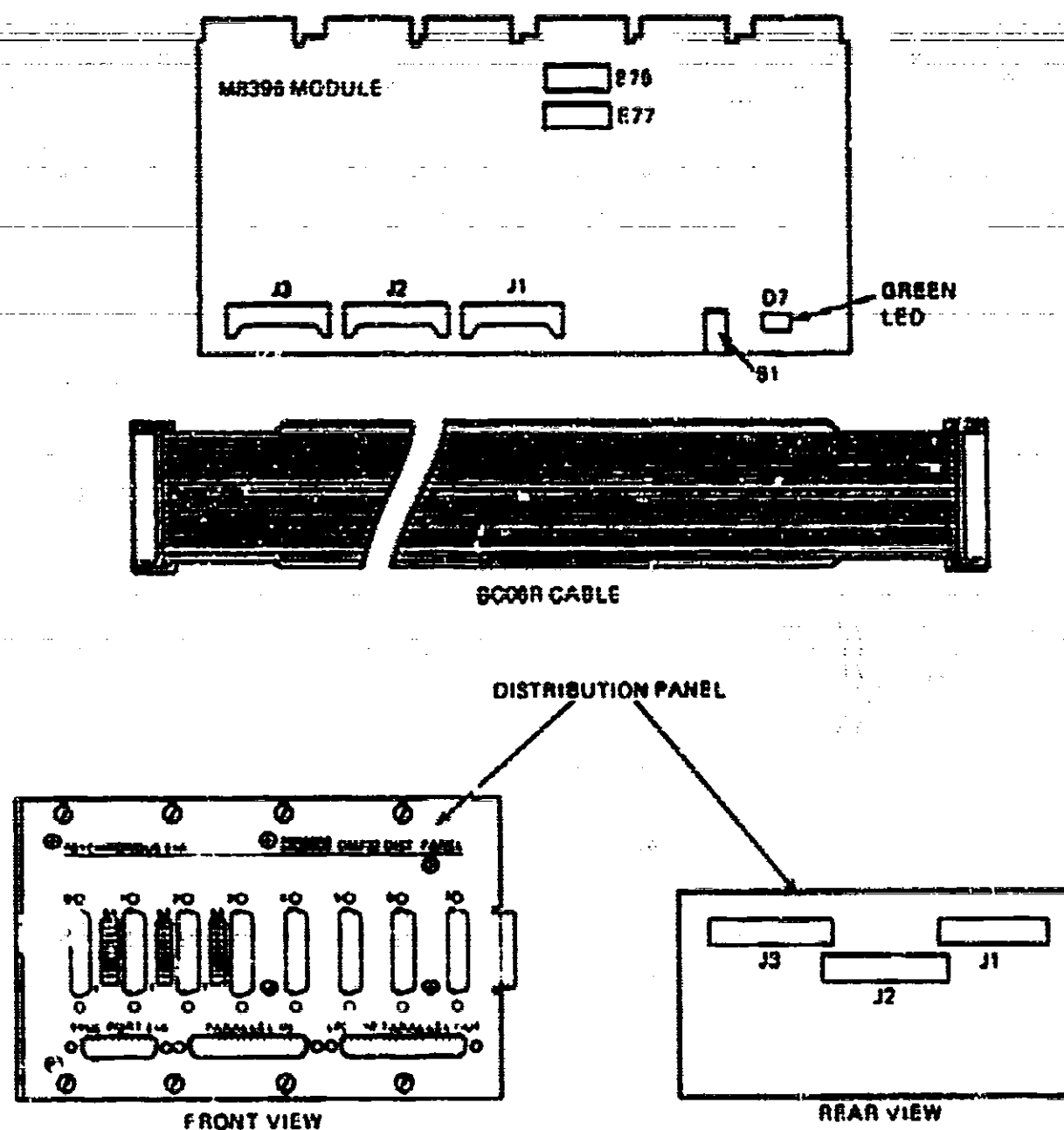
Figure 1-1 DMF32 Components
