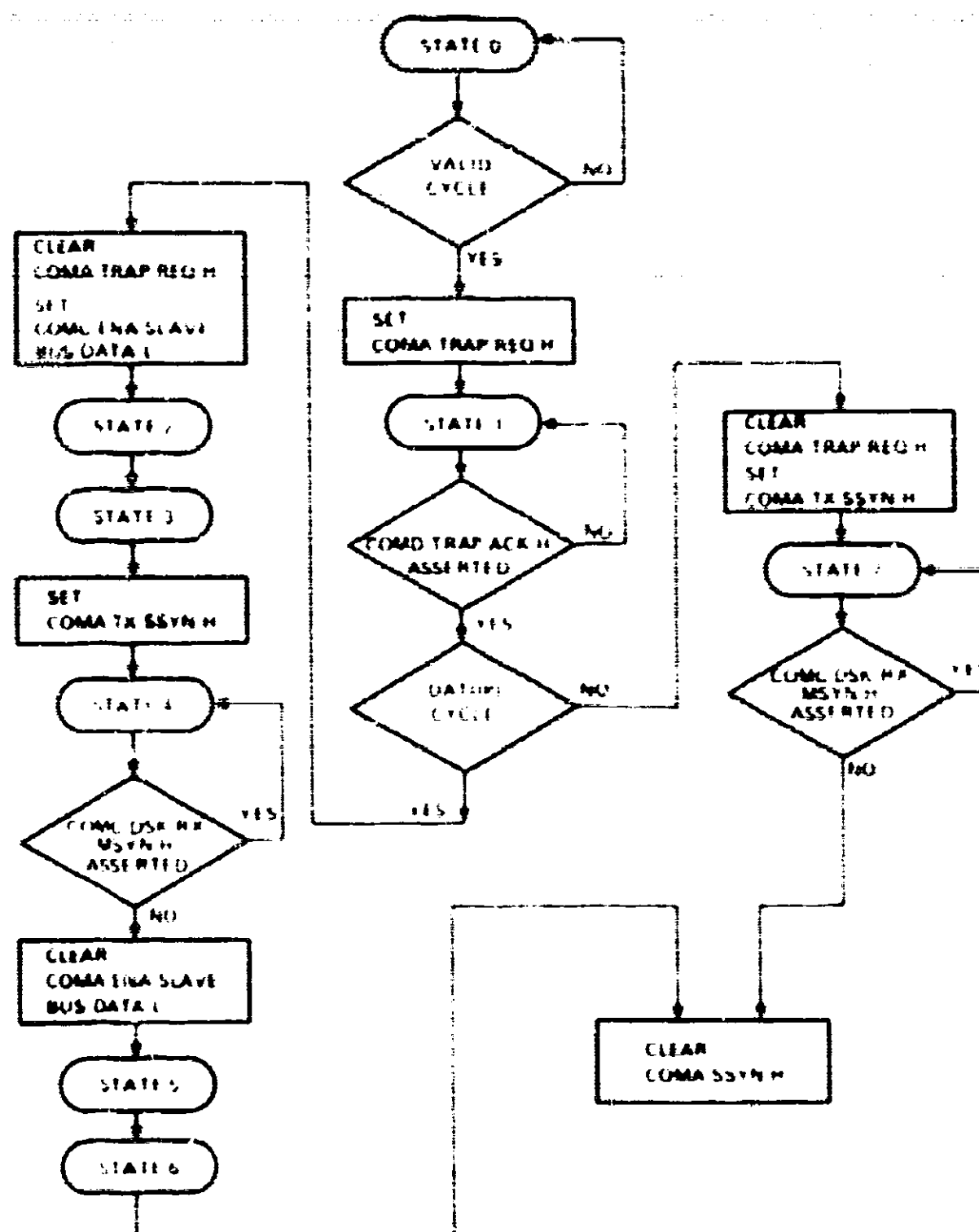
Figure A-7 Slave Control FSM Flow
