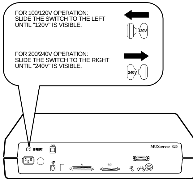
Figure 3–2: Supply Voltage Select Switch
