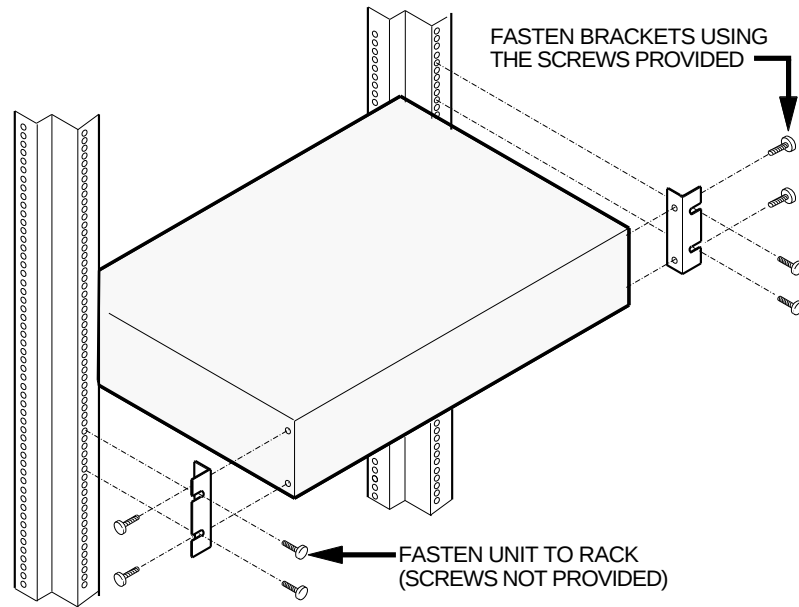
Figure 5-2: Rack Mounting the MUXserver 320
