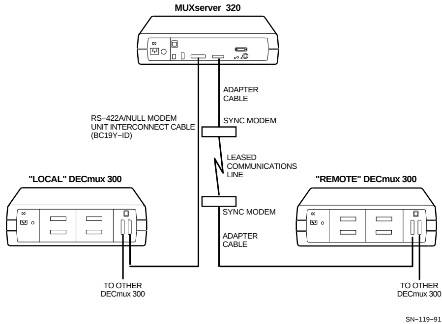
Figure 1-6: Synchronous Link Connections
