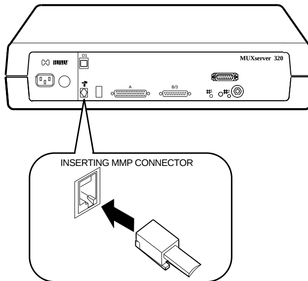
Figure 5–10: Connecting to the Supervisor Port Connector
