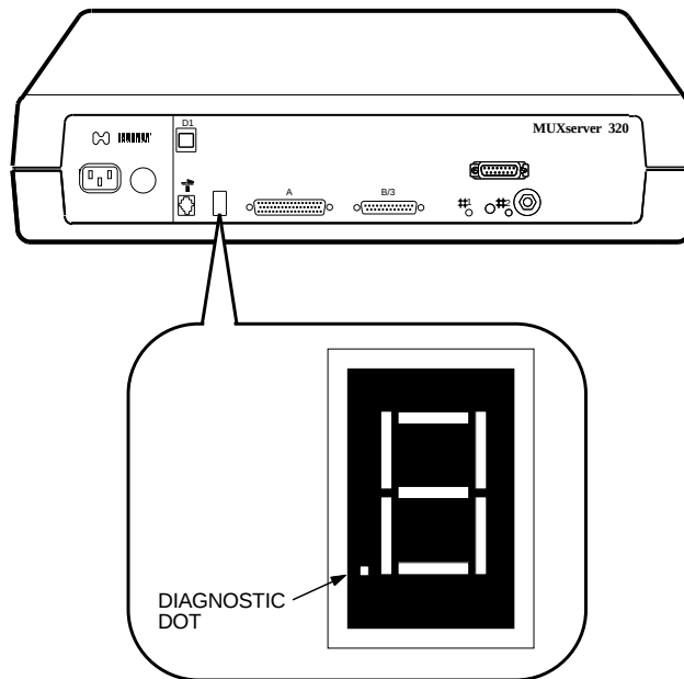
Figure 5-6: 7-Segment Display
