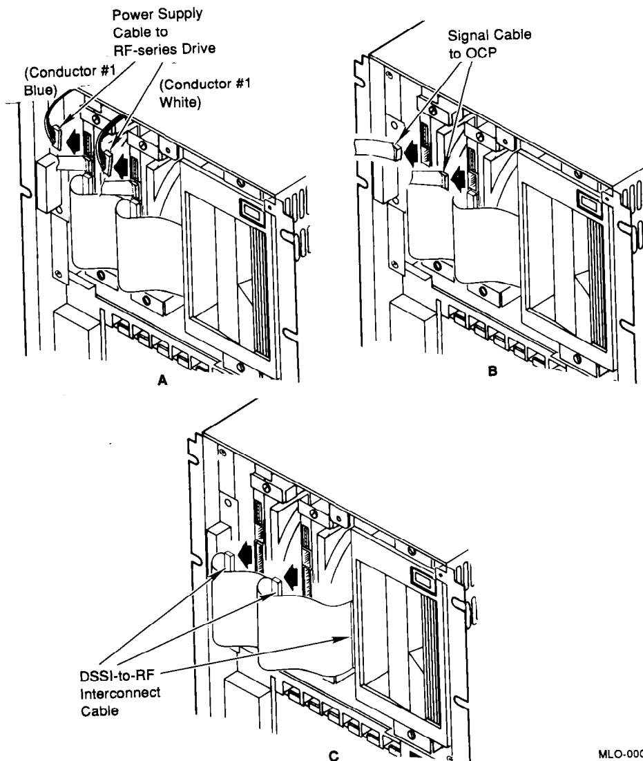
Figure 1-5 Removing the RF-Series Drive Cabling
