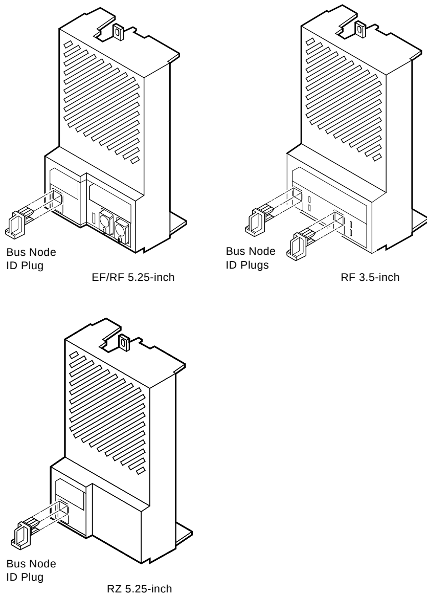
Figure 3-8 Installing the Bus Node ID Plug
