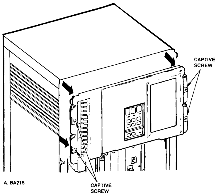
Figure 1-2 Removing the Media Faceplate
