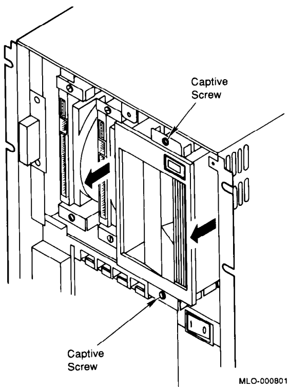
Figure 1-8 Removing the TK-Series Drive
