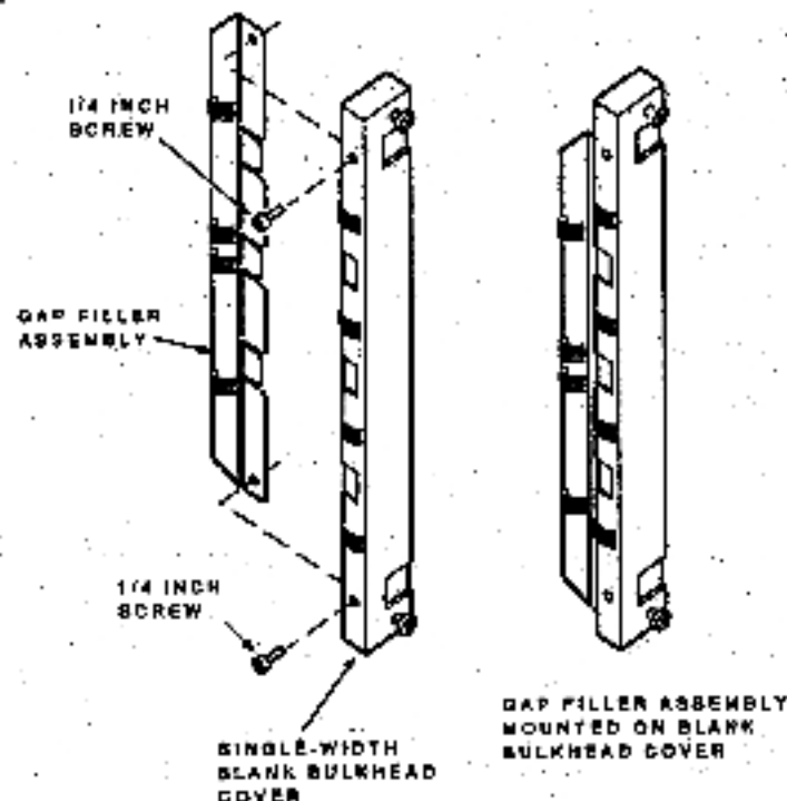
Figure 2-11 Attaching the Gap Filler Assembly
