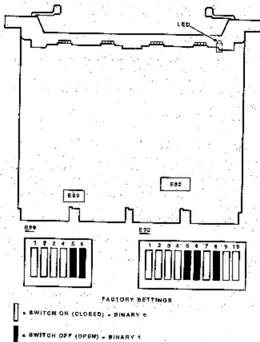
Figure 2-5 DSV11-SF Module Layout
