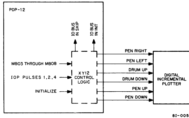
Figure 7-15 XY12 Block Diagram
