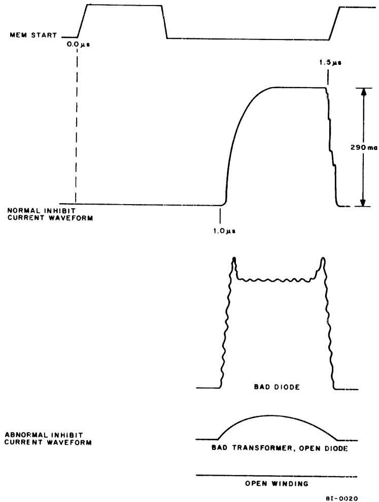
Figure 2-8 Representative Inhibit Current Waveforms
