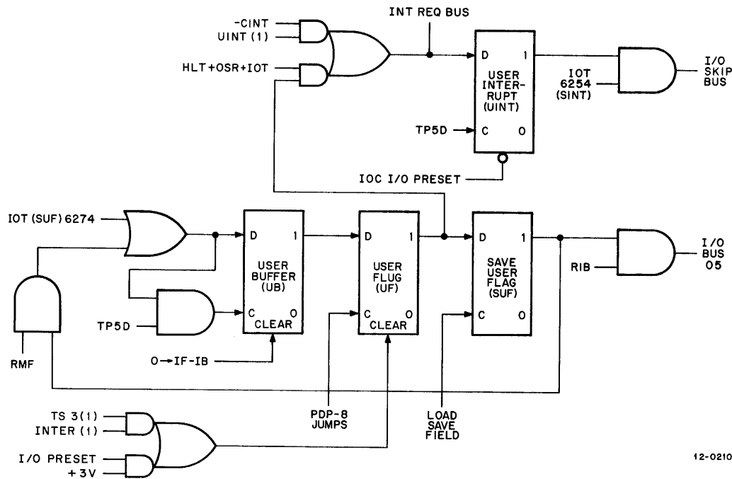
Figure 7-9 KT12 Simplified Block Diagram
