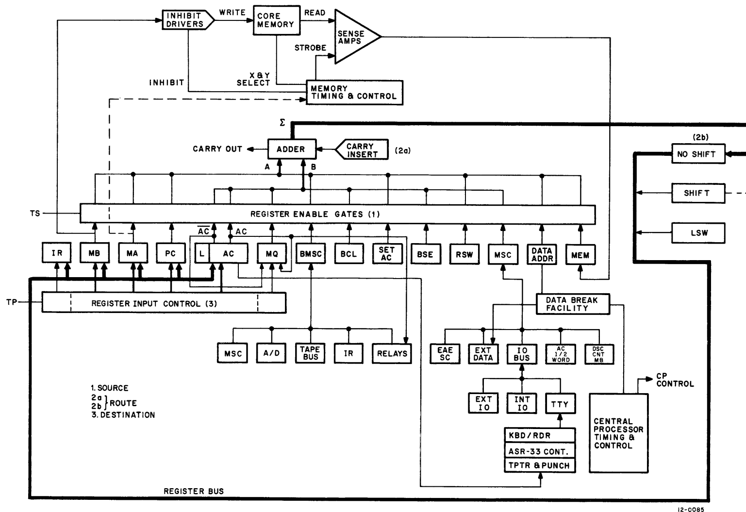
Figure 1-2 PDP-12 Data Flow
