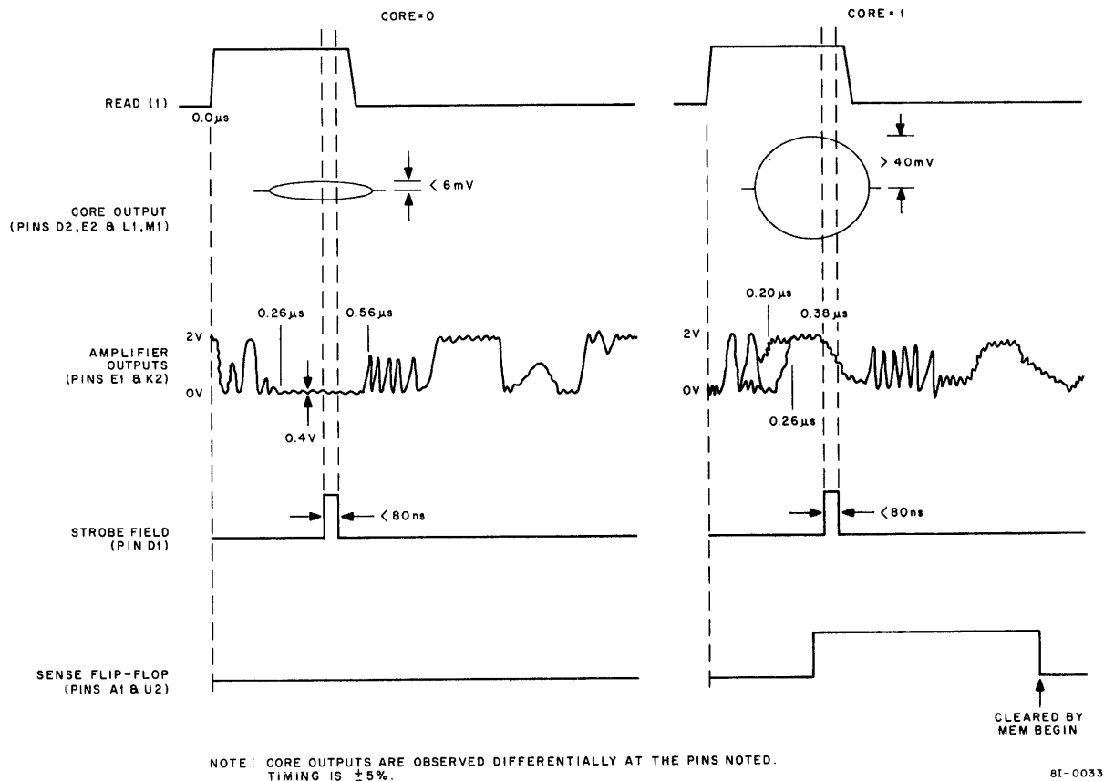
Figure 2-9 Representative Sense Amplifier Waveforms
