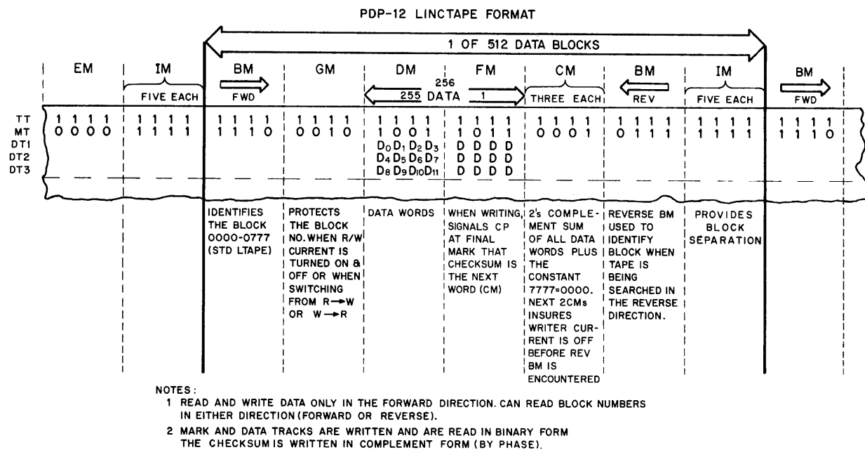
Figure 6-8 Standard LINCtape Detailed Format
