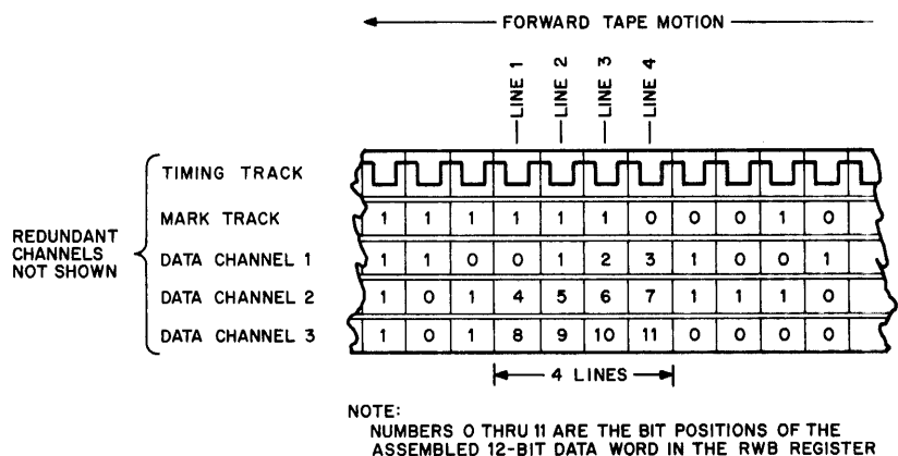
Figure 6-4 Track Allocation Showing Redundantly Paired Tracks
