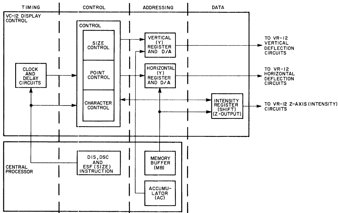
Figure 5-10 Display Addressing Block Diagram
