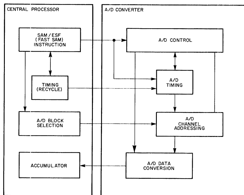
Figure 5-1 A/D Control General Block Diagram
