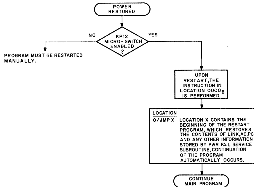
Figure 7-7 Typical Power Failure Program Service Routine
