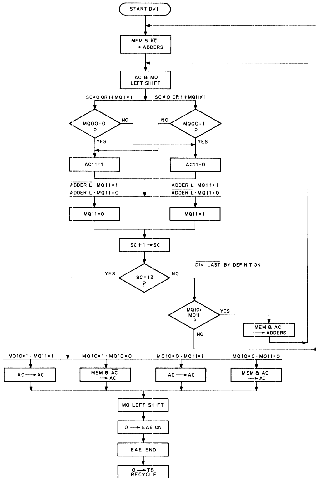
Figure 7-3 KE12 EAE DVI Flow Chart
