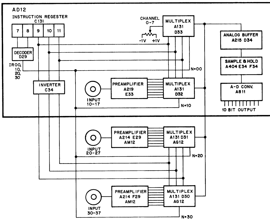
Figure 7-1 Multiplexer Selection
