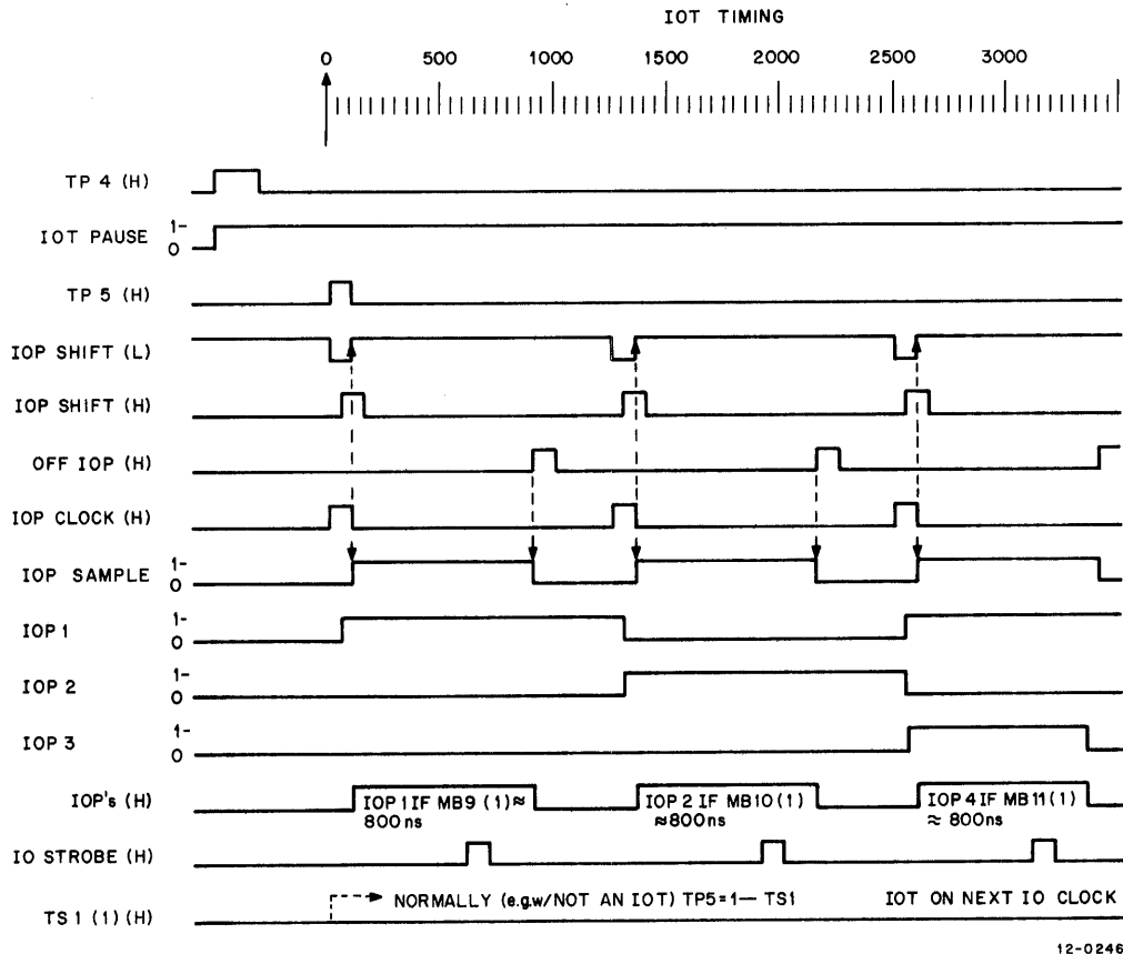
Figure 1-10 IOT Timing
