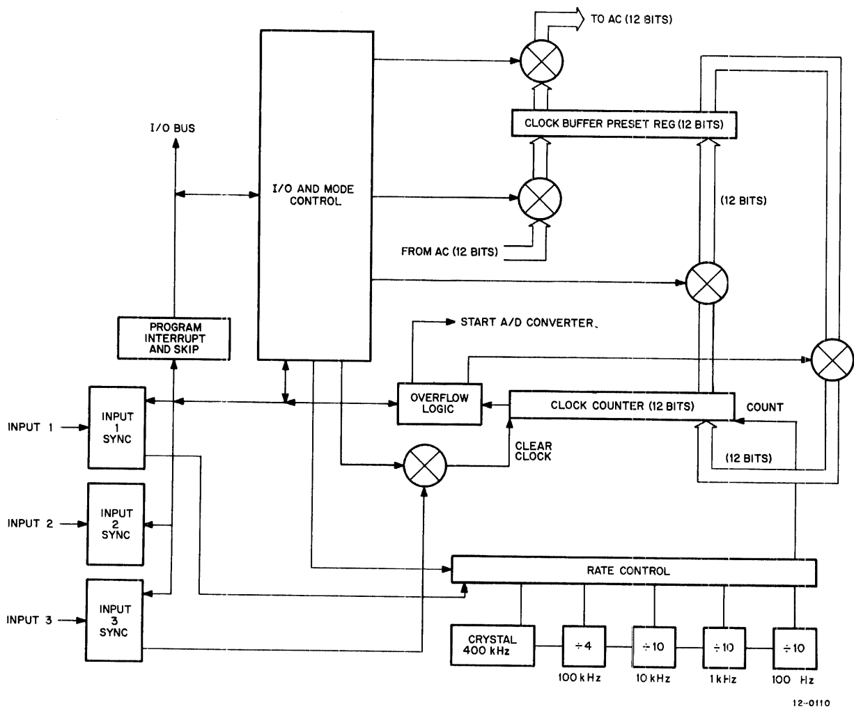
Figure 7-11 KW12-A Organization
