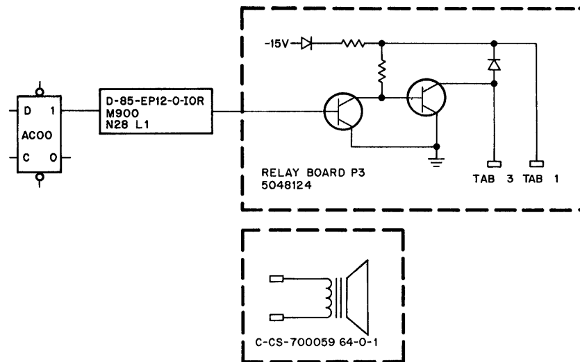
Figure 5-13 Speaker and Control
