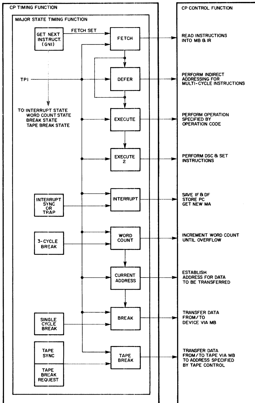
Figure 1-6 CP, Major State Block Diagram
