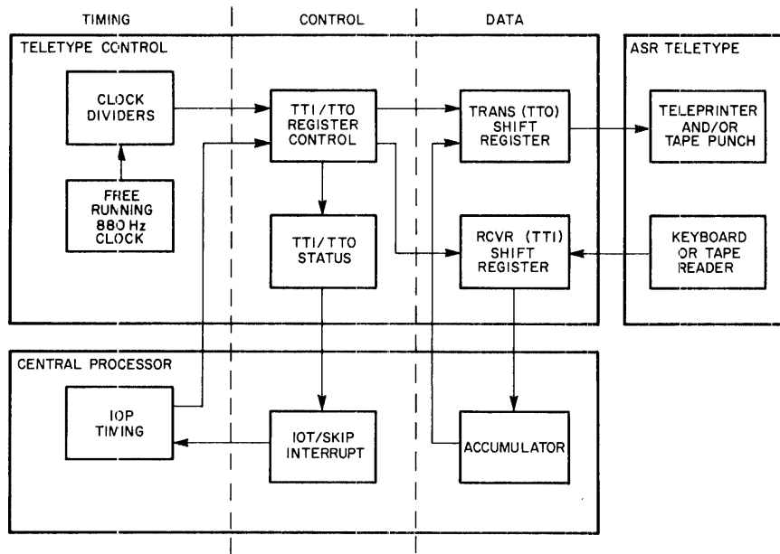
Figure 4-1 Teletype Control Block Diagram
