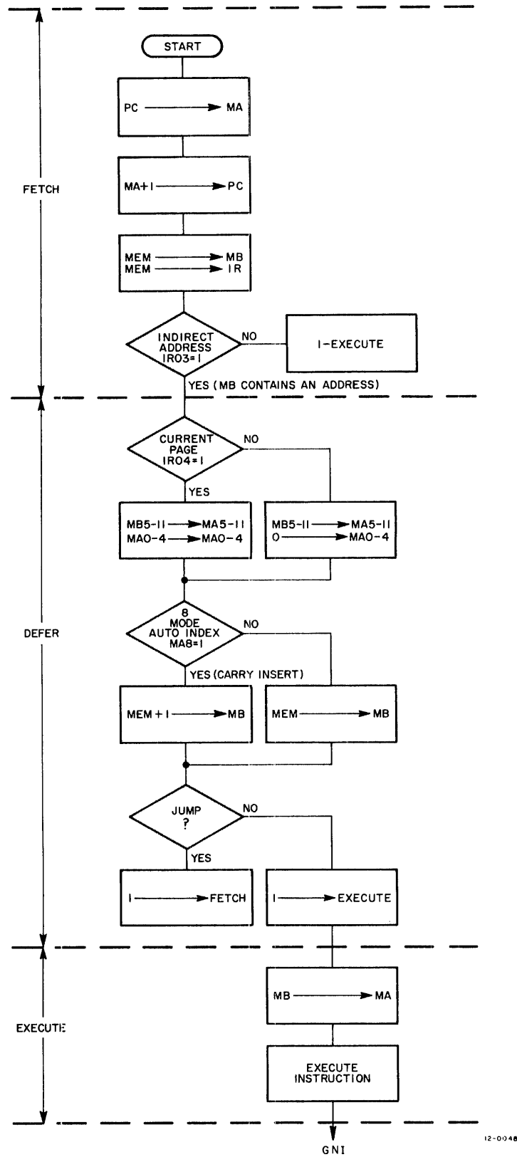
Figure 1-8 8-Mode Address Modification
