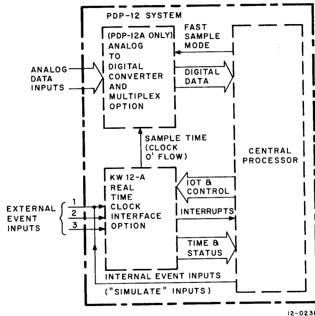
Figure 7-10 KW12-A Real Time Interface Functional Relationship
