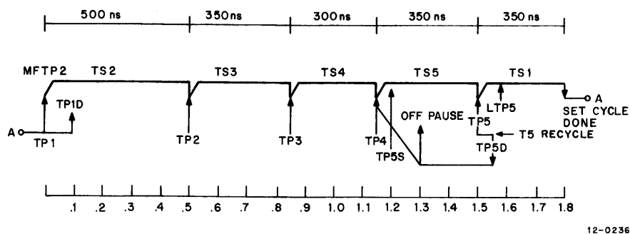
Figure 1-4 CP Timing Cycle: Time Pulses and Time States
