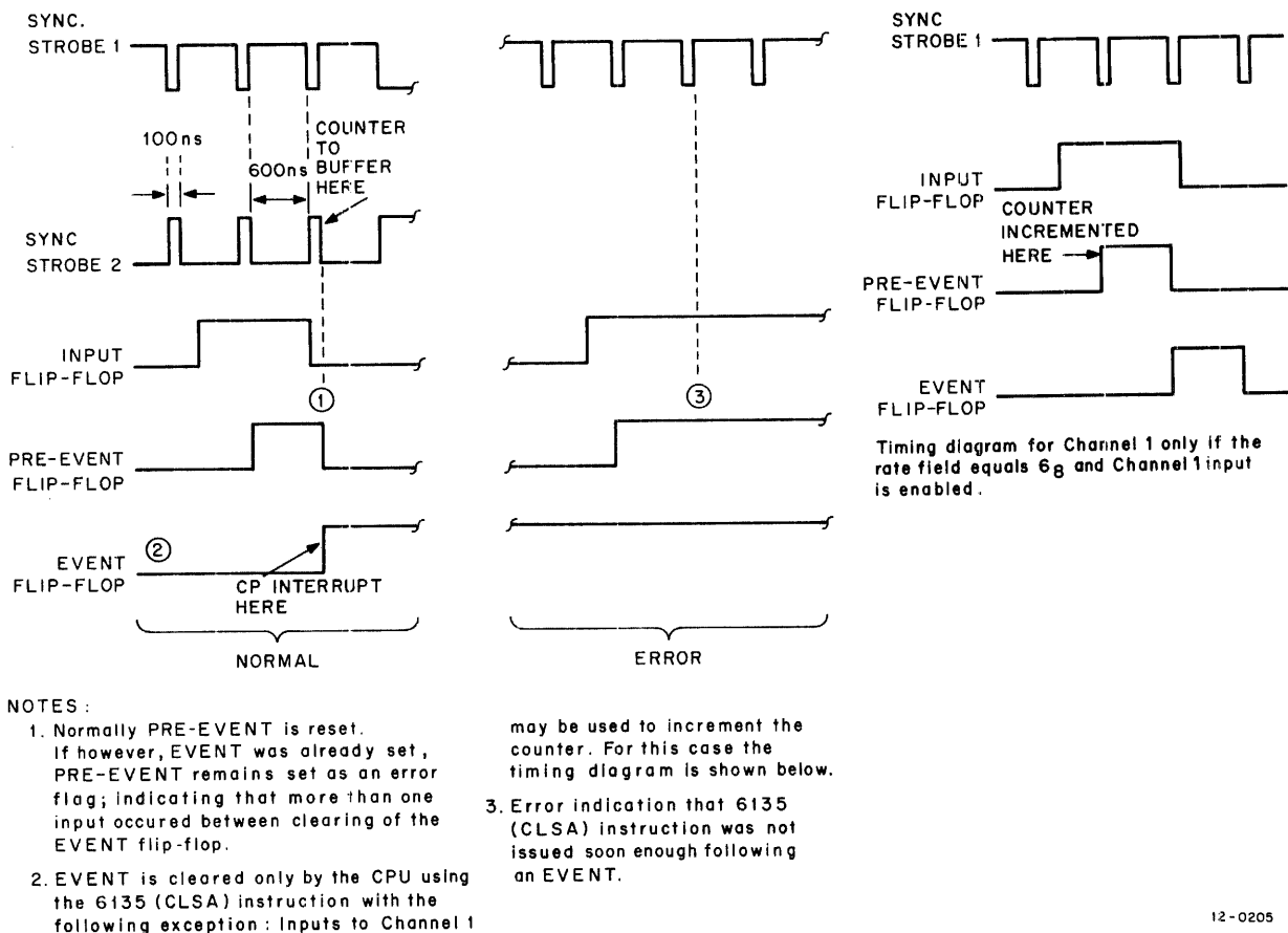
Figure 7-13 KW12-A Timing Diagram
