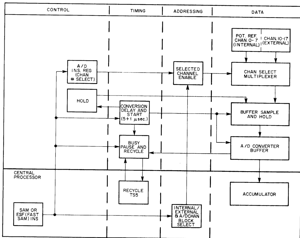
Figure 5-2 A/D Control Block Diagram
