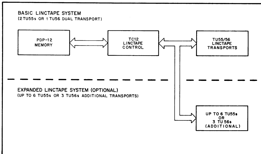
Figure 6-1 LINTape System Configuration
