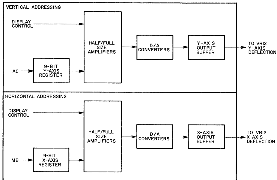
Figure 5-6 Display Control General Block Diagram
