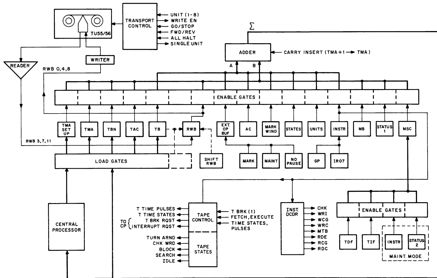
Figure 6-15 PDP-12 LINCTape Flow Diagram
