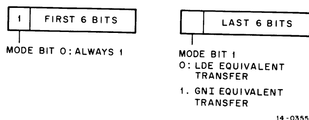
Figure 9-14 DC14-F Receiver Data Format
