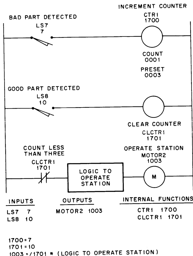
Figure 3-12 Up Counter Circuit and Boolean Equations to Shut Down a Station on Three Successive Bad Parts
