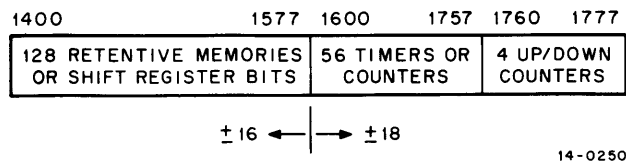
Figure 3-1 Internal I/O Groupings
