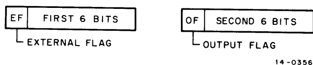
Figure 9-15 DC14-F Transmitter Data Format
