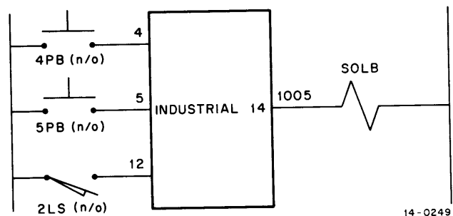
Figure 2-13 Typical Industrial 14 Wiring Diagram for Example 5, Simplified
