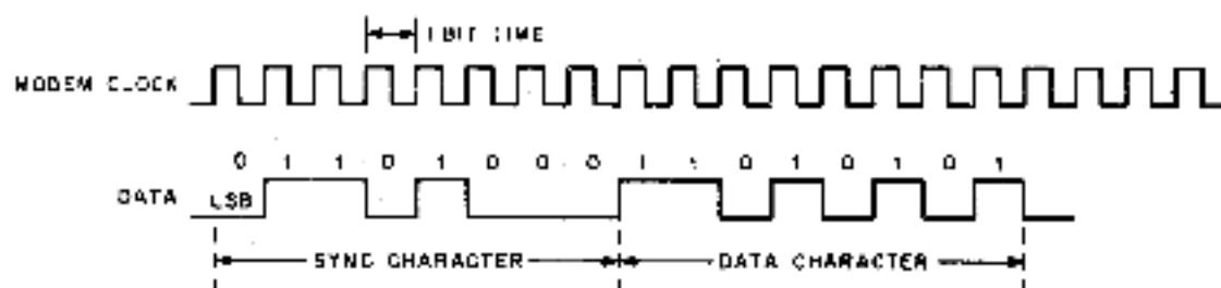
Figure 1-2 Synchronous Format
