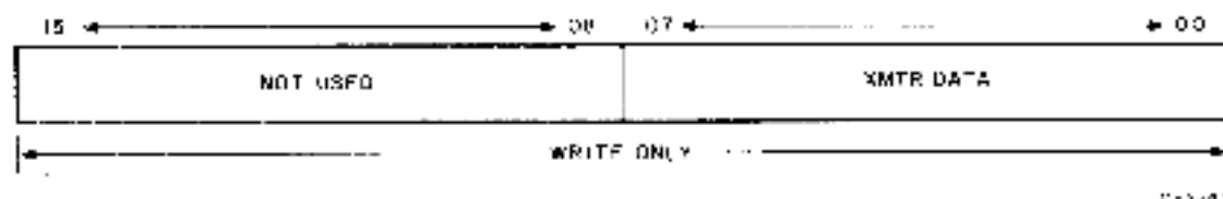
Figure 3-5 Transmitter Data Buffer (TXDBUF)
