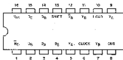
TOP VIEW OF IC
