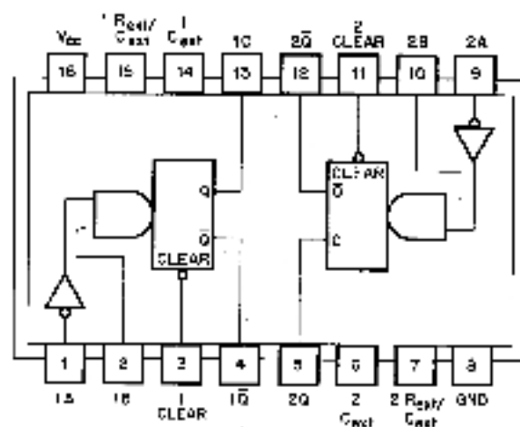
FUNCTIONAL LOGIC/PIN LOCATION
