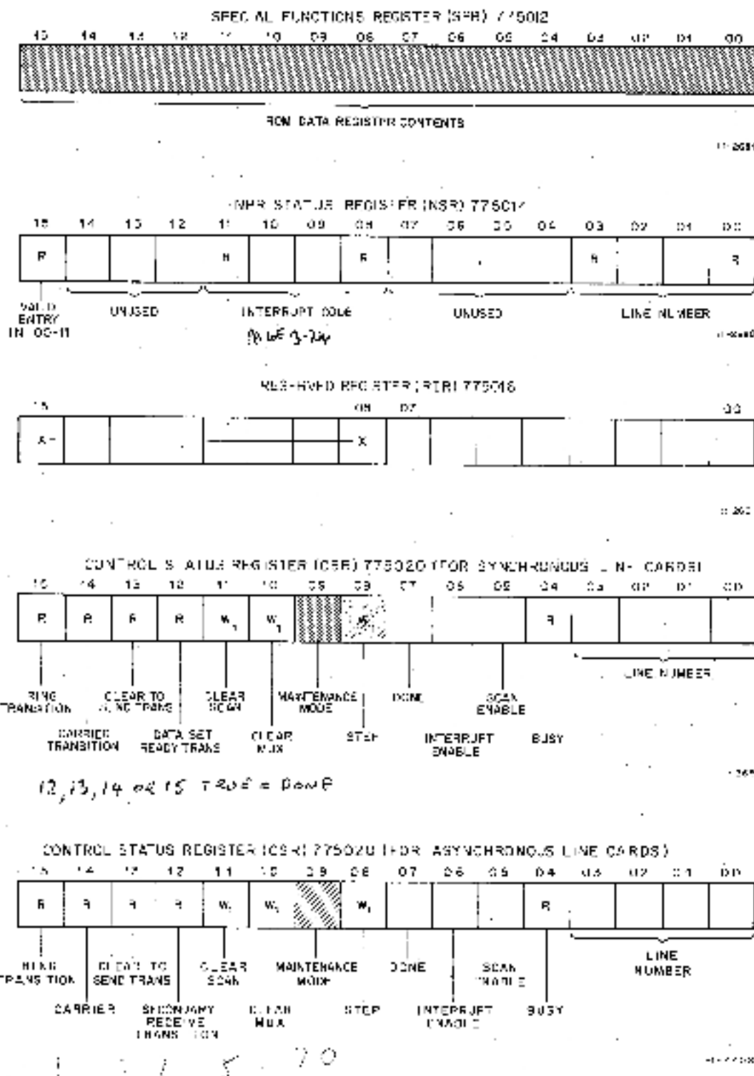
Figure 3-3 DV11 Primary Registers (Sheet 2 of 3)
