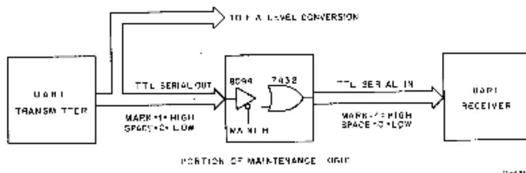
Figure 5-4 Typical Internal Maintenance Mode Path (Asynchronous)
