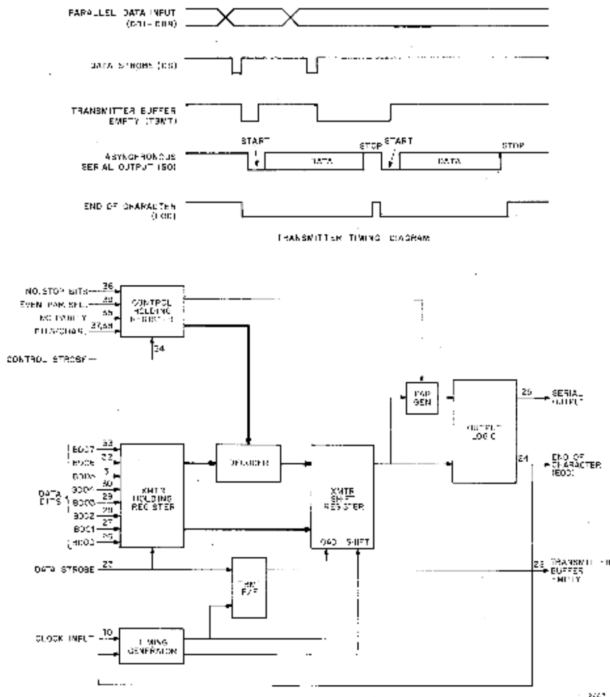
Figure B-8 UART Transmitter. Block Diagram and Simplified Timing Diagram
