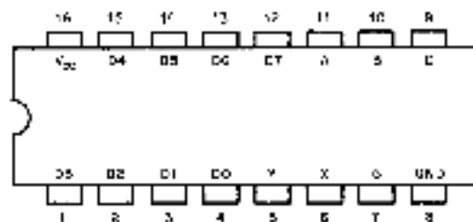
PIN LOCATOR TOP VIEW OF DIP
