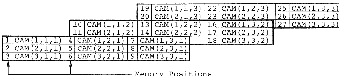
3-Dimensional Array CAM(3,3,3)
