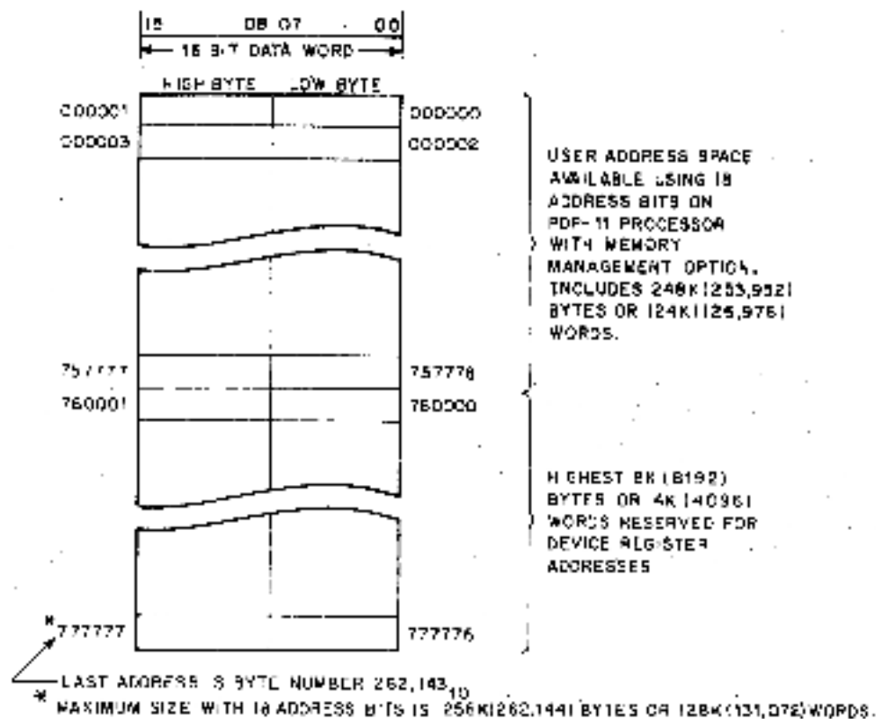
Figure A-1 Memory Organization for Maximum Size Using 15 Address Bits
