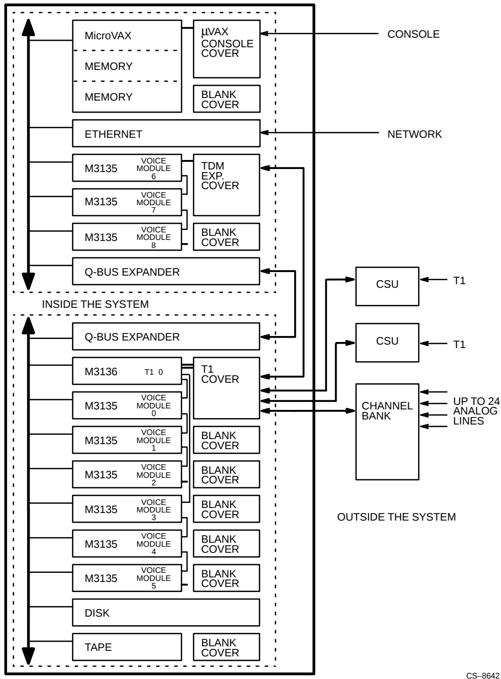
Figure 16 Voice/T1 Module MDM Numbering for 72-Line DECvoice-T1 System
