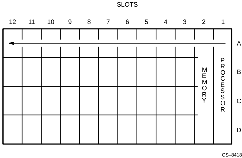
Figure 8 Bus Grant Continuity Path
