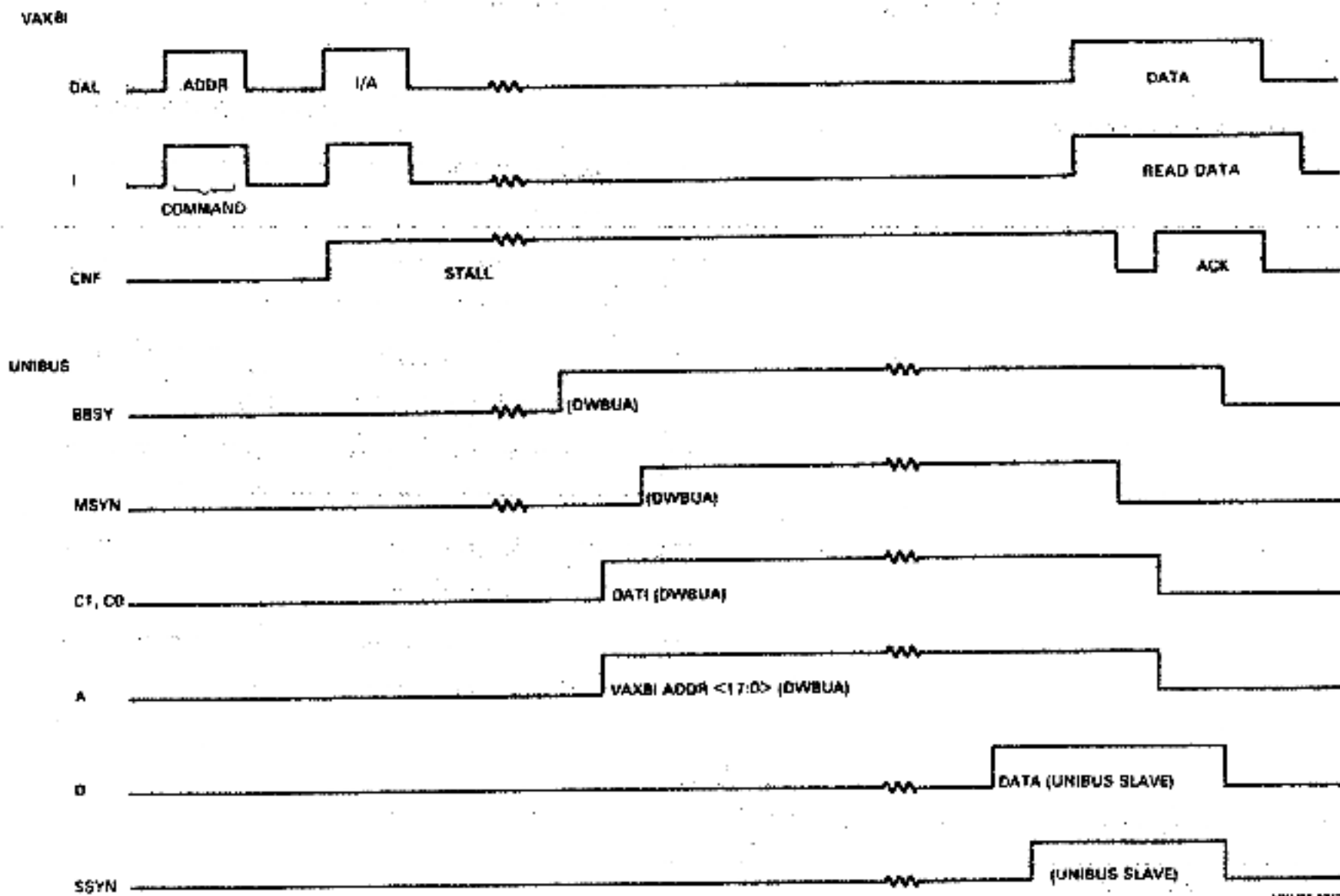
Figure 4-8 VAXBI-to-UNIBUS READ Timing Diagram
