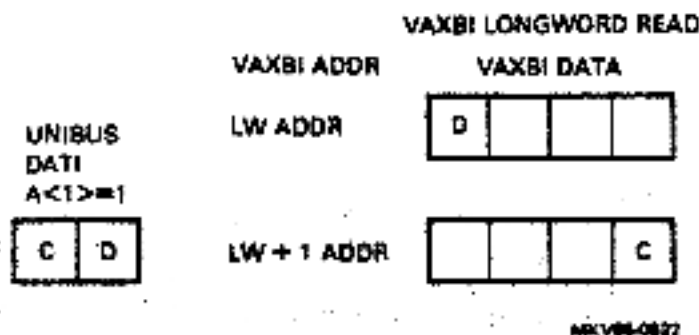
Figure 1-2 DATI with UNIBUS Address Bit <01> Set
