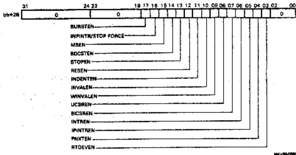
Figure 3-9 BCI Control Register
