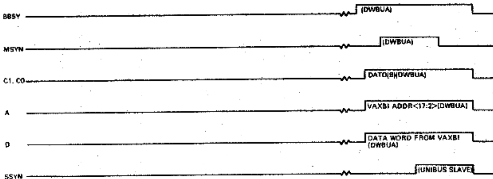
Figure 4-7 VAXBI-to-UNIBUS WRITE Timing Diagram
