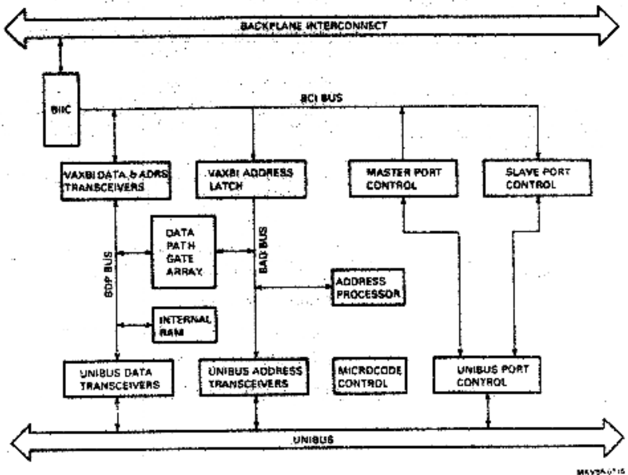
Figure 4-1 DWBUA Block Diagram
