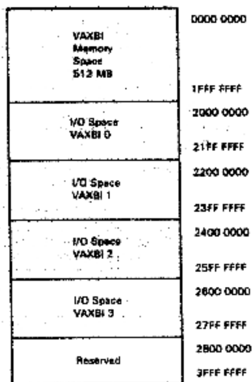
Figure 3-1 System Address Space Distribution
