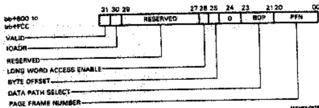
Figure 3-20 UNIBUS Map Register
