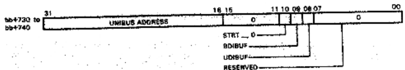
Figure 3-17 Microdiagnostic Register
