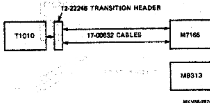
Figure 2-2 DWBUA Configuration
