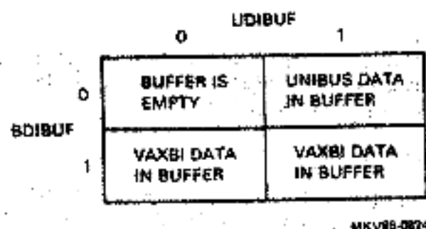
Figure 1-3 BDIBUF and UDIBUF Flags
