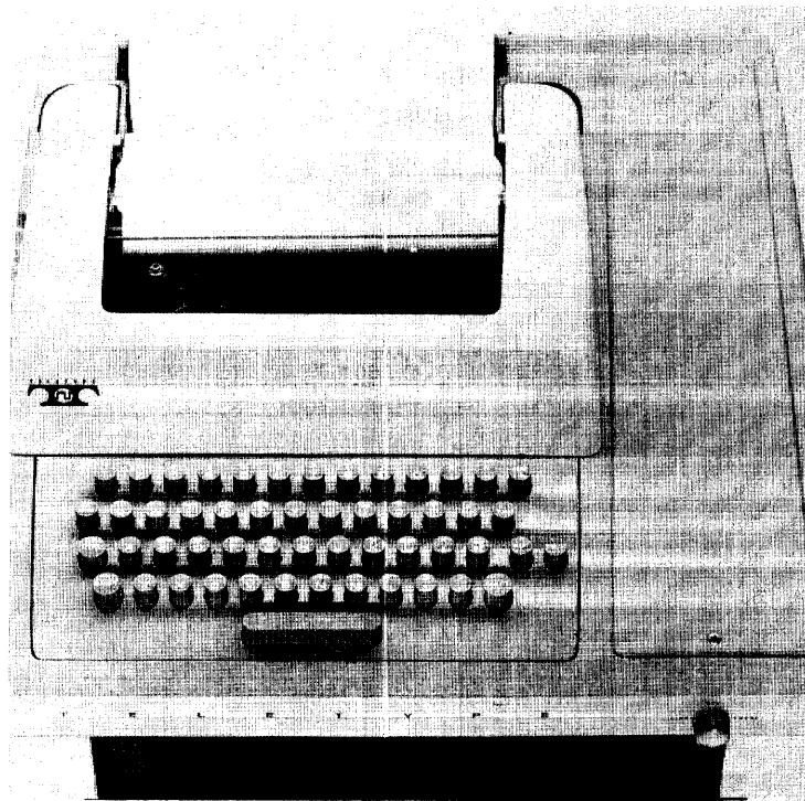
Figure 3-6 Keyboard-Printer Type 626
