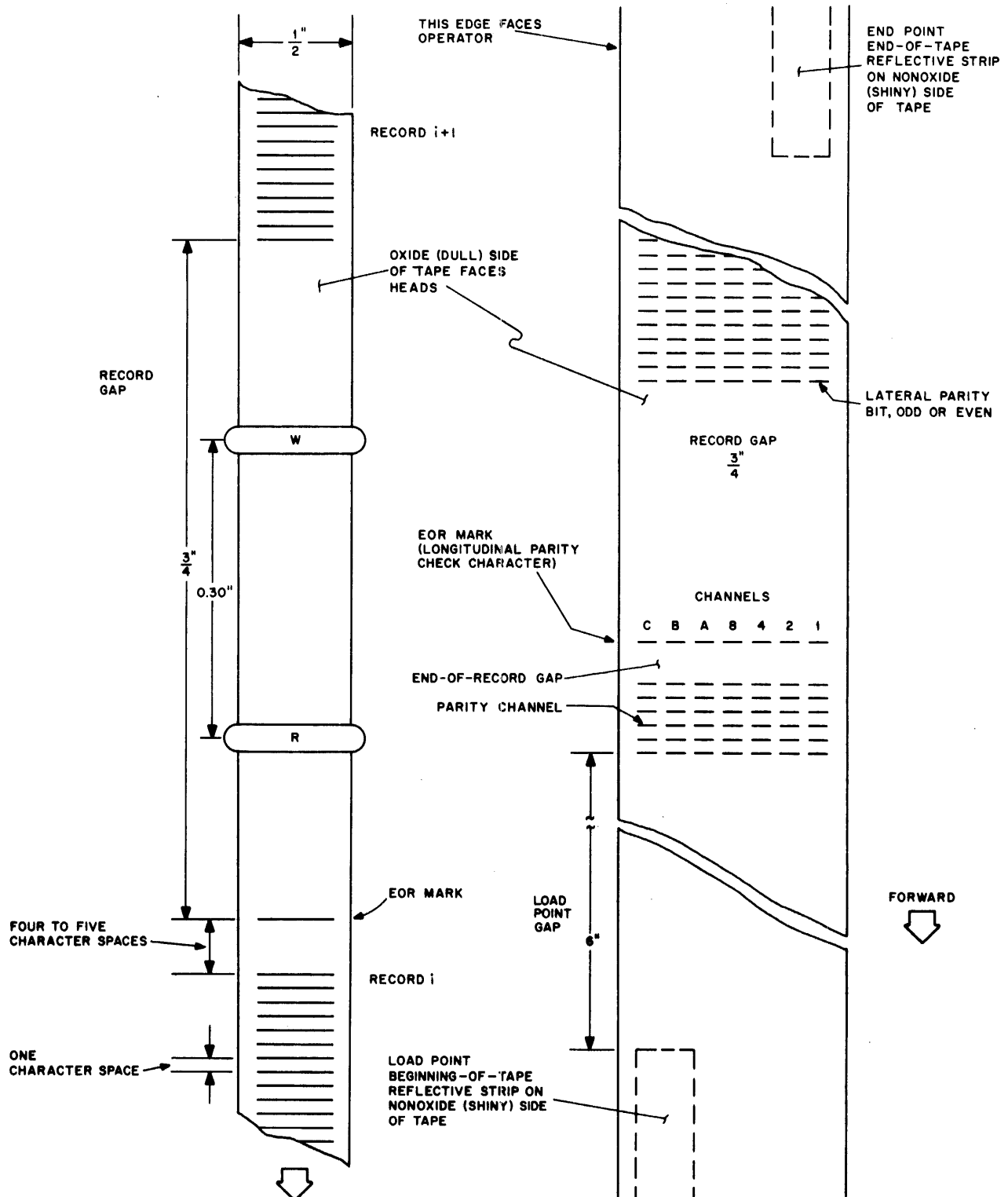
Figure 1-3 Tape Format
