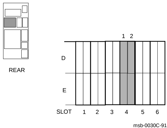
Figure 2-7: XMI Backplane Segments D and E
