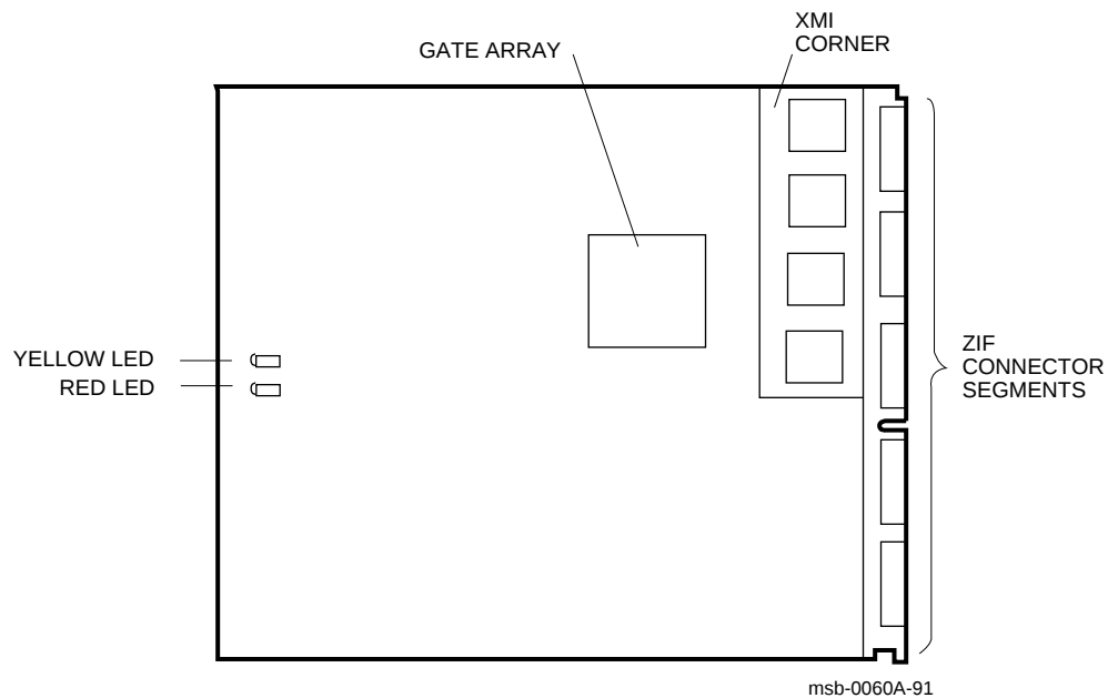
Figure 1–2: T2018 Module
