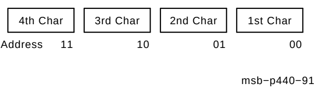
Figure B-4 Byte String Storage
