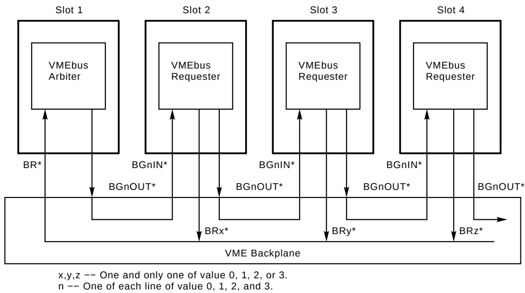
Figure 3-3 VME Arbitration Bus
