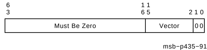
Figure 6–4 XMI IDENT Response Format
