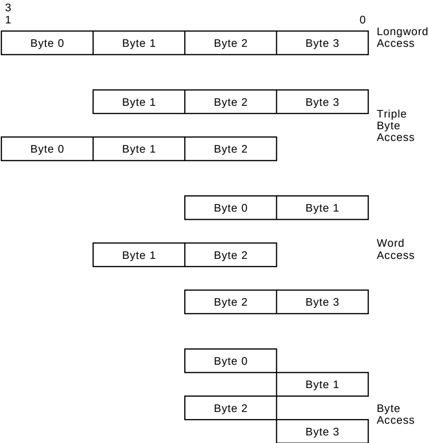
Figure B-1 Big Endian VME Byte Lane Formats
