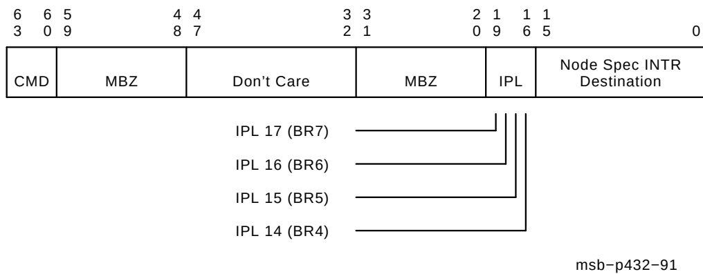
Figure 6–2 XMI IDENT Command Format
