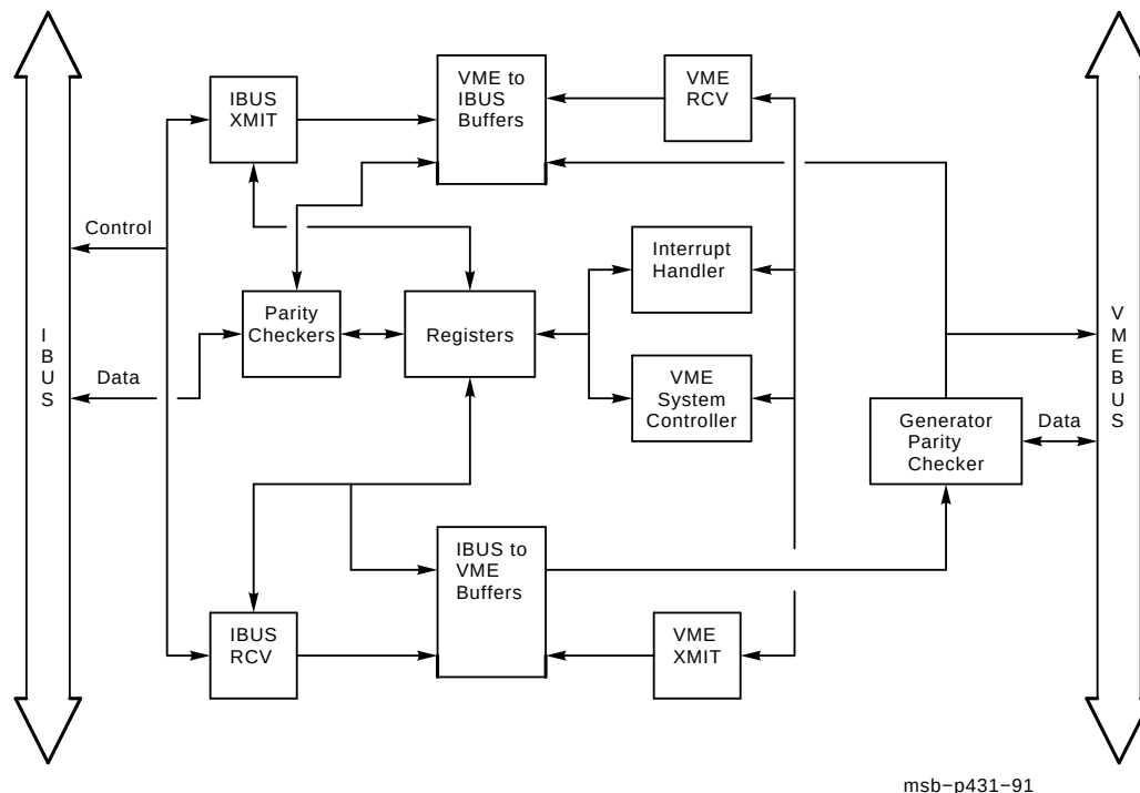
Figure 4–1 C3200 Block Diagram
