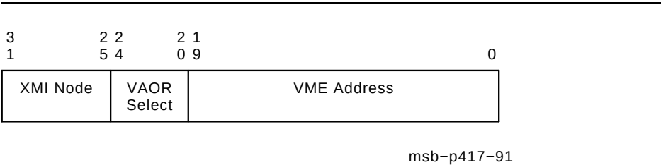
Figure 2–4 CPU Transaction Command Format
