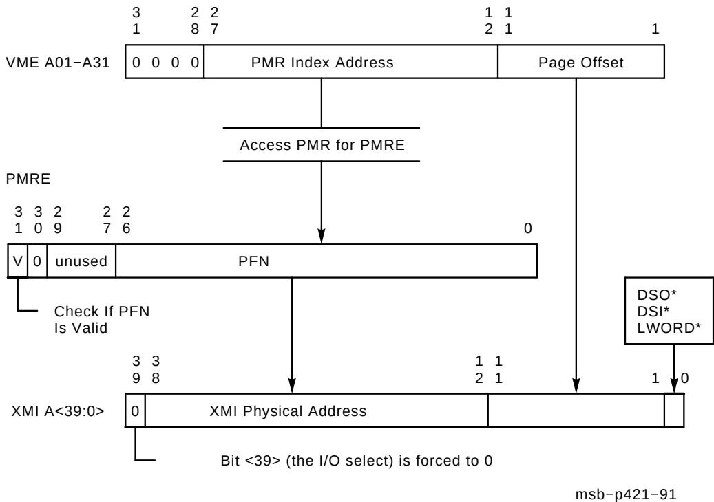
Figure 2–9 40-Bit VAX Address Translation Using 4-Kbyte Page Size
