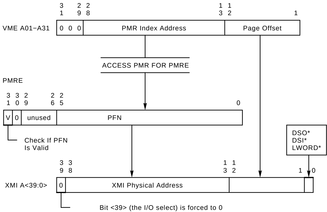
Figure 2–10 40-Bit VAX Address Translation Using 8-Kbyte Page Size
