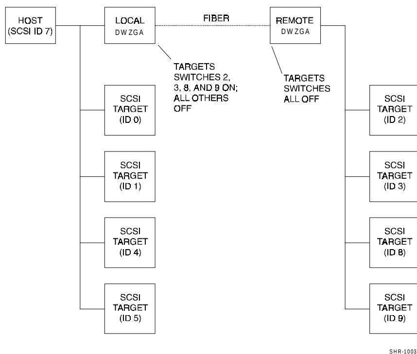
Figure 2-1 Typical Fiber-Optic UltraSCSI Extender Configuration
