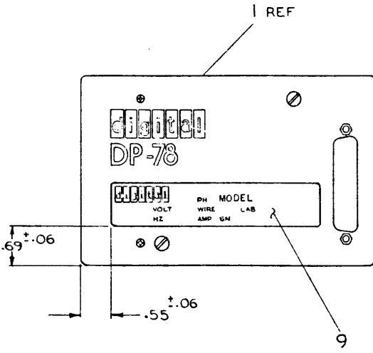
DETAIL "A" (BOTTOM SIDE OF ENCLOSURE)
