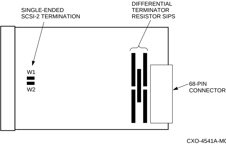
Figure 3–2 End-Bus DWZZB Bus Terminators
