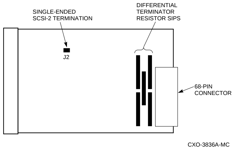
Figure 2-2 End-Bus DWZZA Bus Terminators
