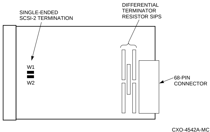
Figure 3-4 Mid-Bus DWZZB Bus Terminators
