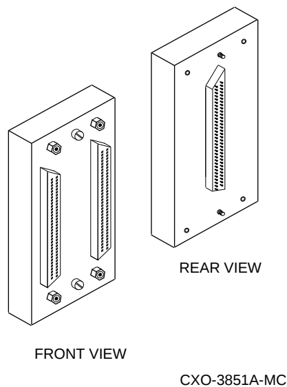
Figure 2-3 H885-A Trilink Connector
