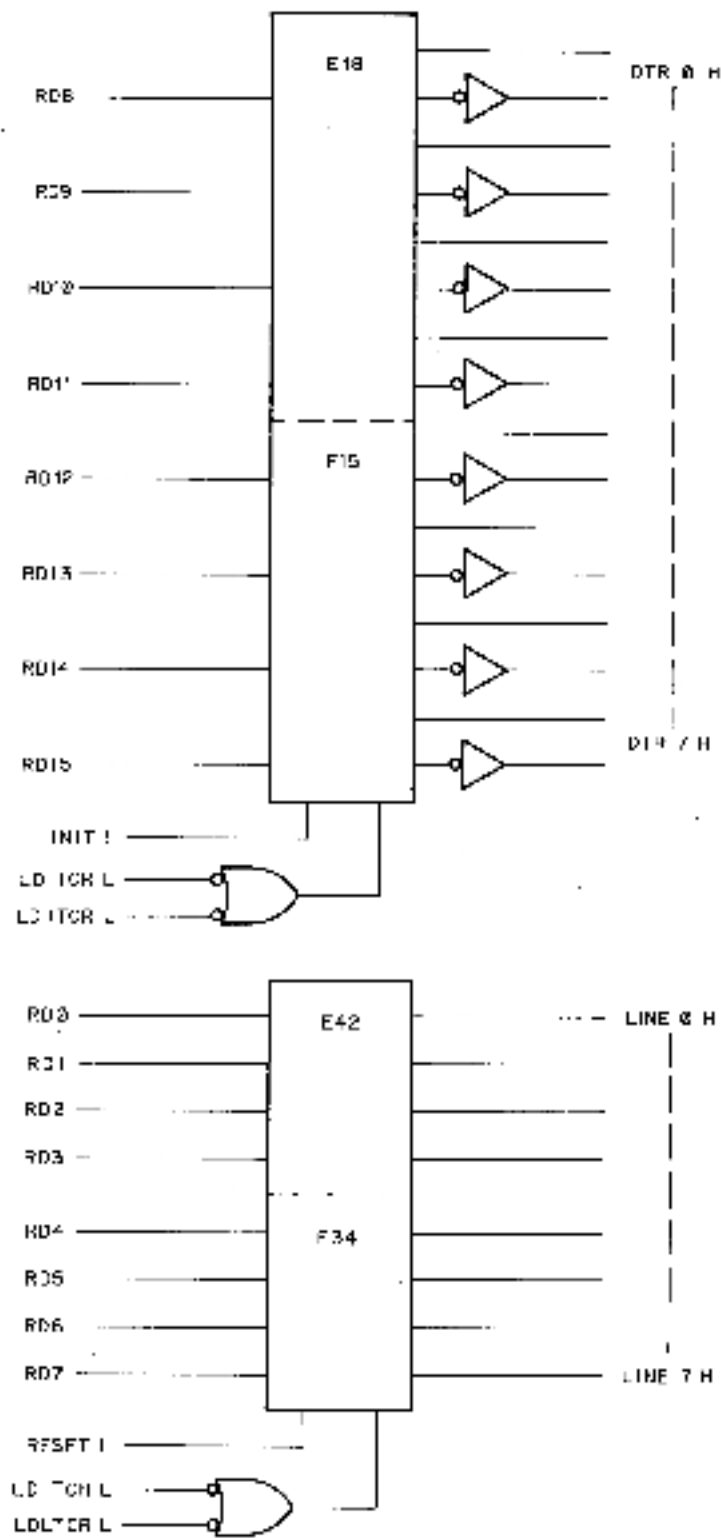
Figure 4-19 TCR Diagram
