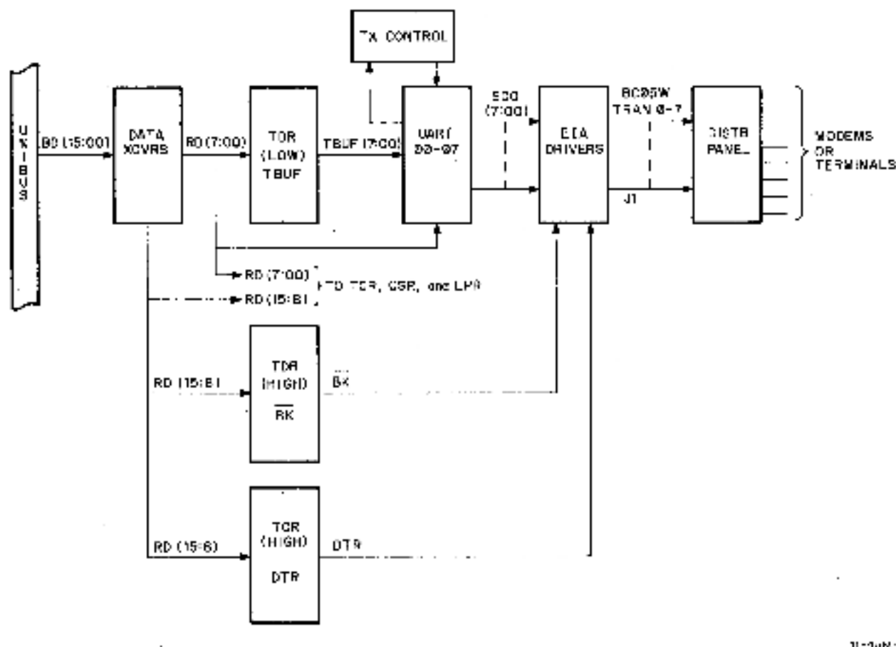
Figure 4-2 Unibus-to-Modem Data Flow (Transmit)
