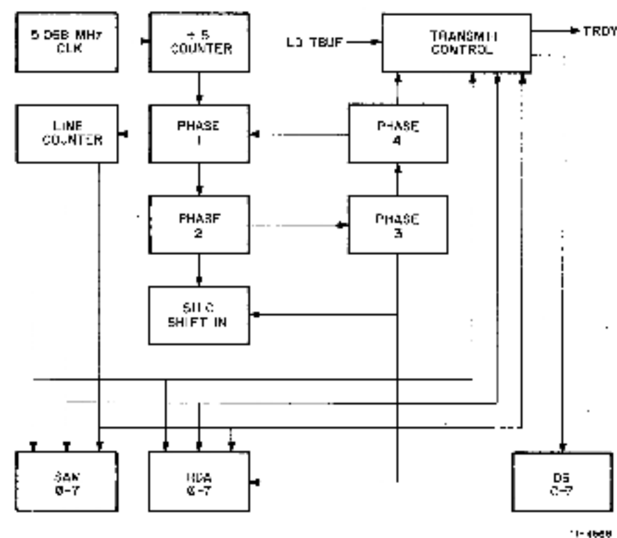
Figure 4-11 Scanner Block Diagram
