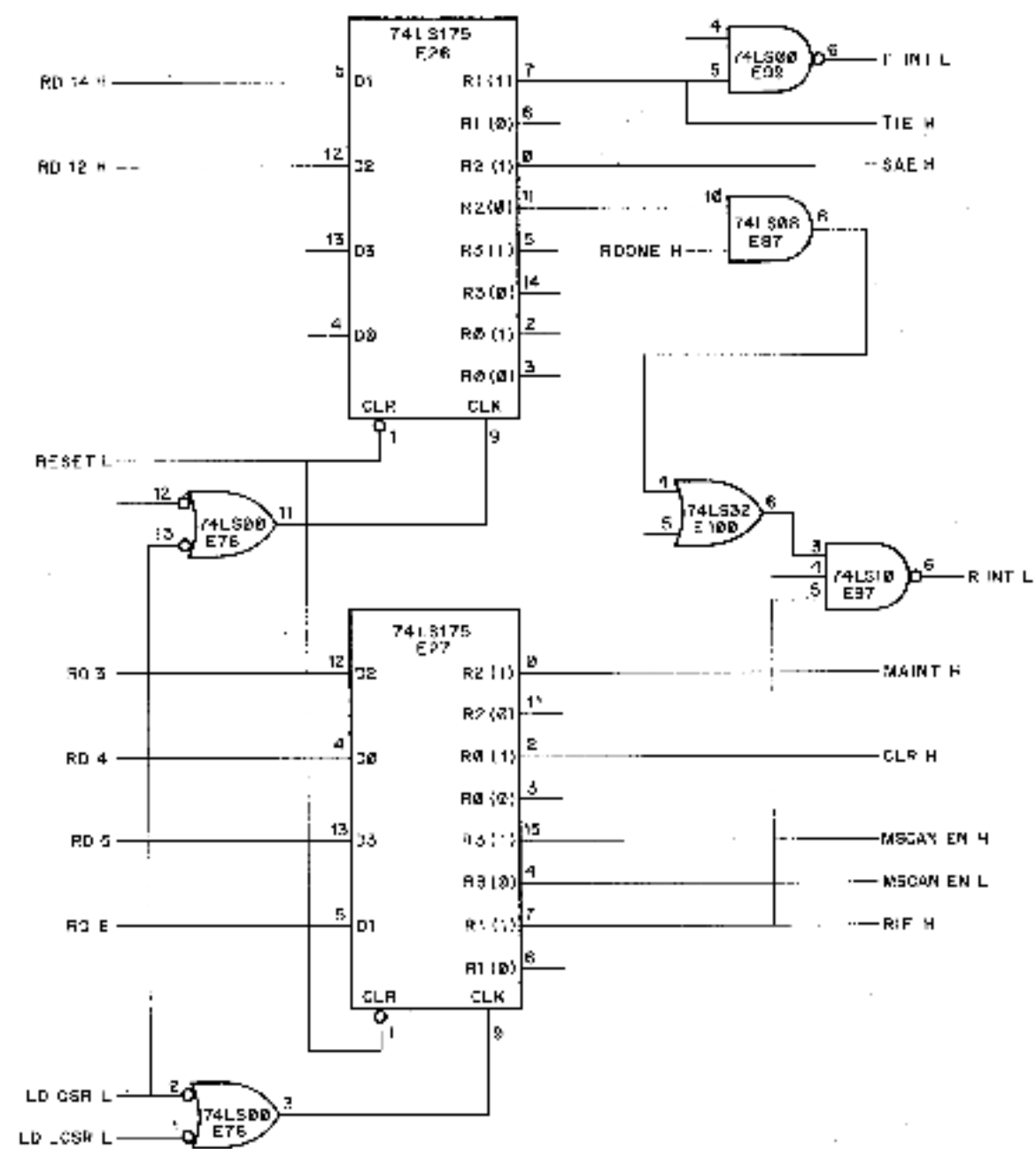
Figure 4-17 CSR Diagram
