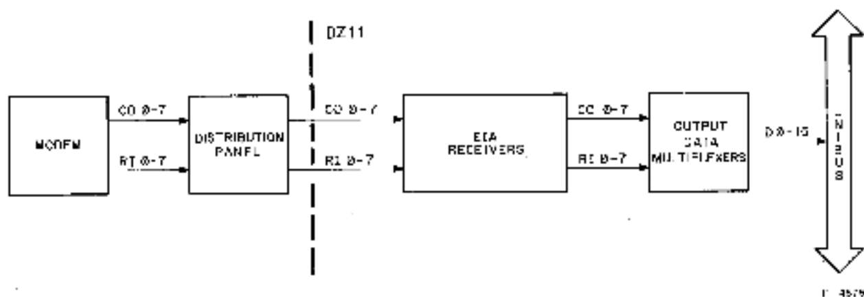
Figure 4-20 MSR Diagram
