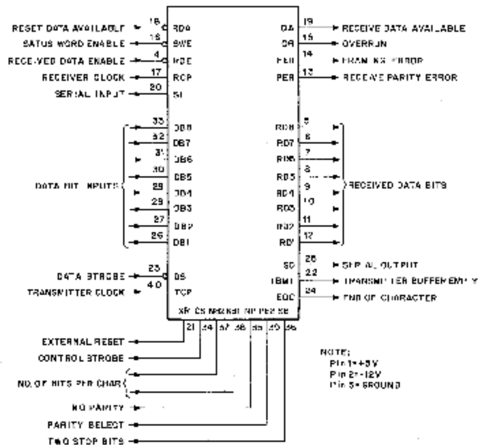
Figure C-4 UART Signal/Pin Designations
