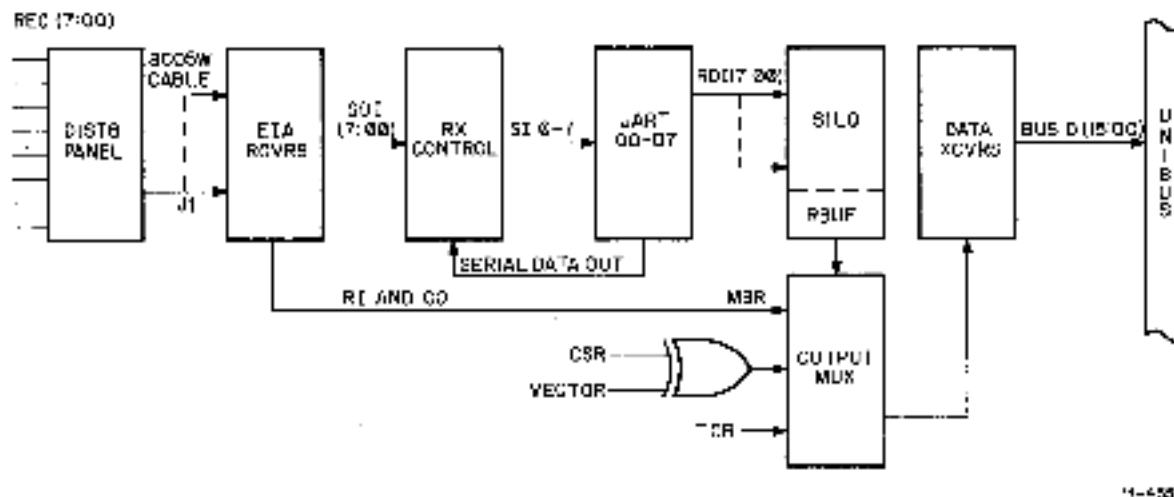
Figure 4-1 Modem-to-Unibus Data Flow (Receive)
