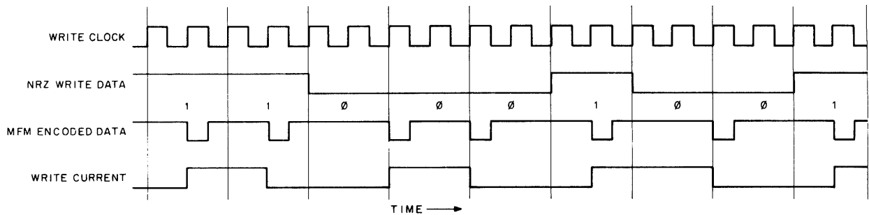
Figure 2-15 Modified Frequency Modulation Waveform Example
