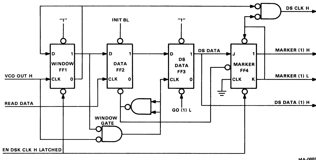
Figure 4-16 Data Separator Circuit
