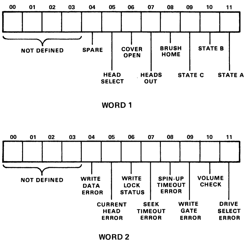
Figure 2-6 Disk Status Register Format
