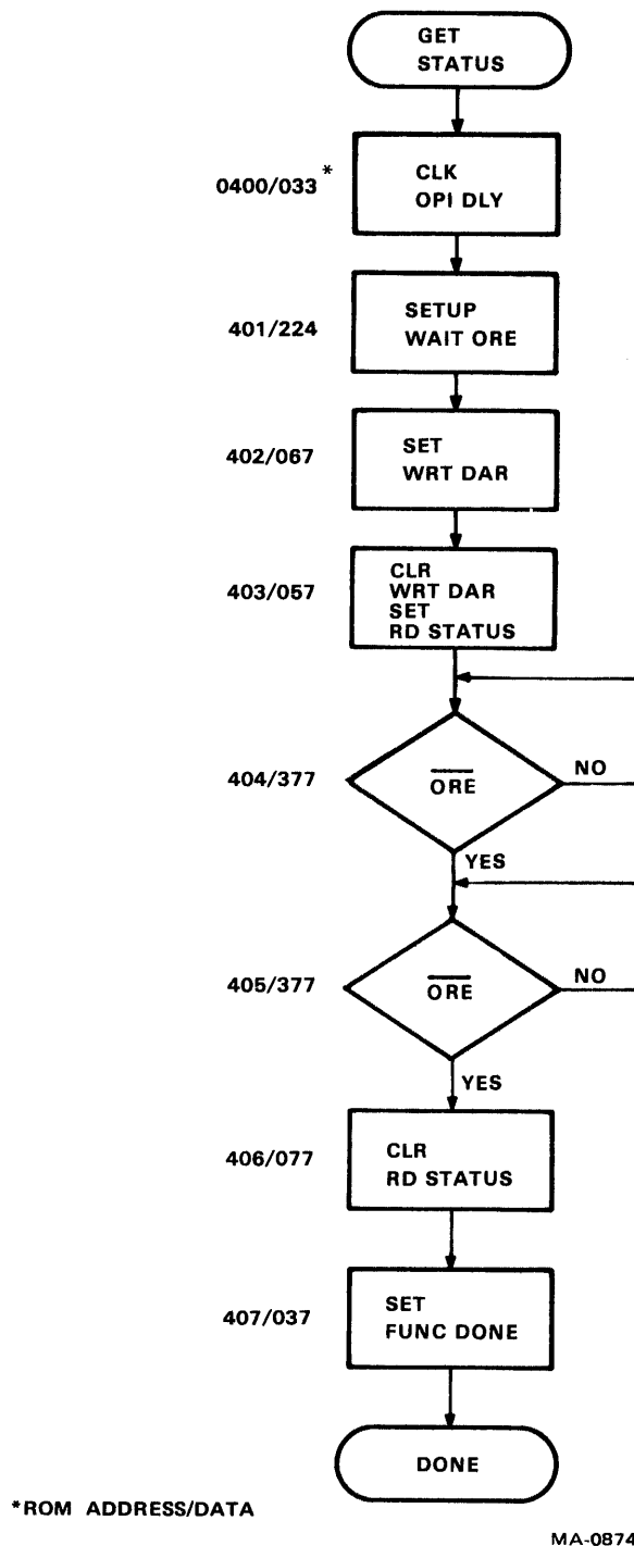
Figure 4-5 Get Status Mode Flow Diagram
