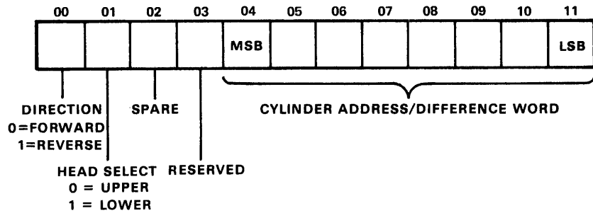
Figure 2-4 Command Register A Format
