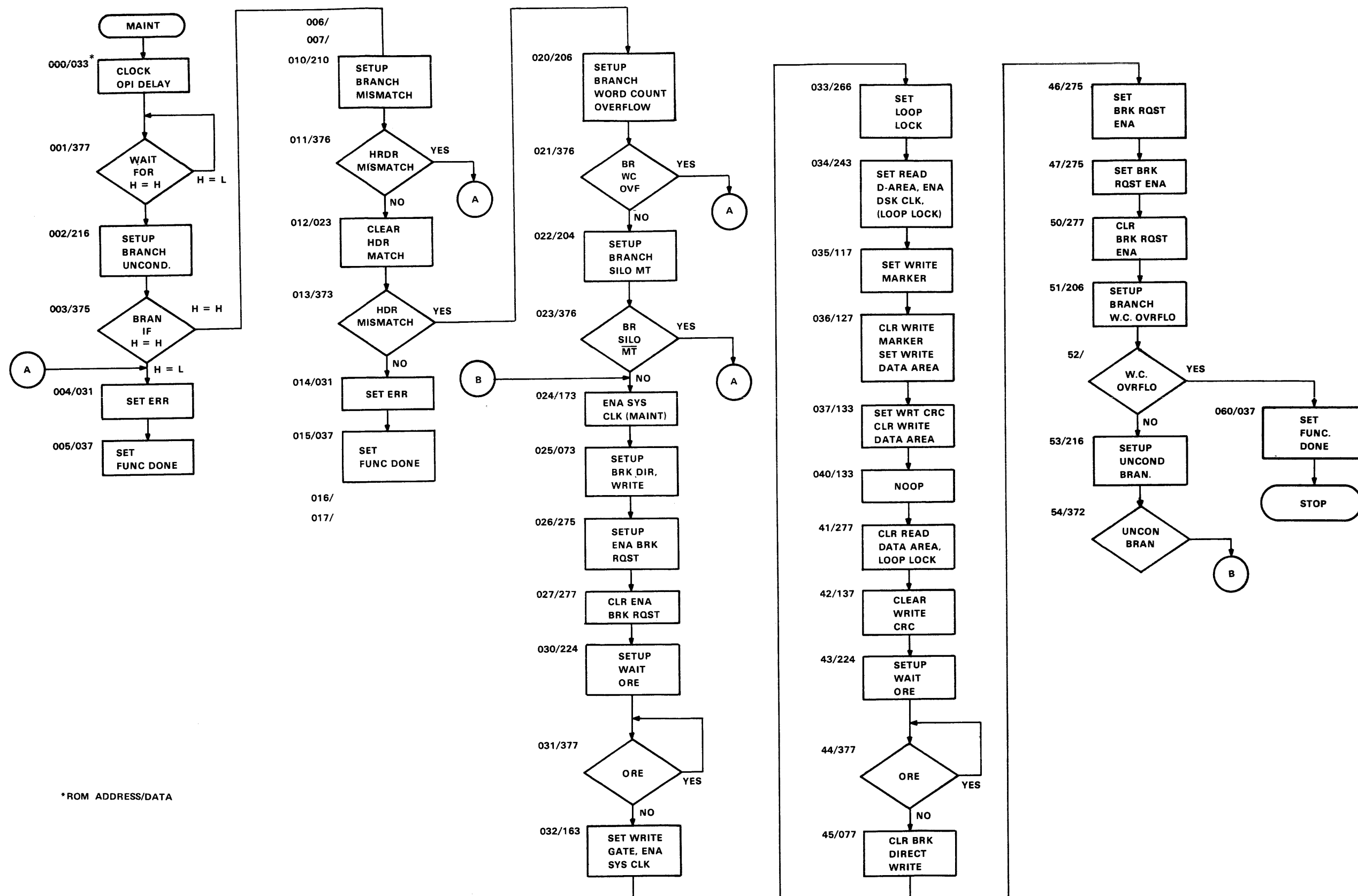
Figure 4-3 Maintenance Mode Flow Diagram
