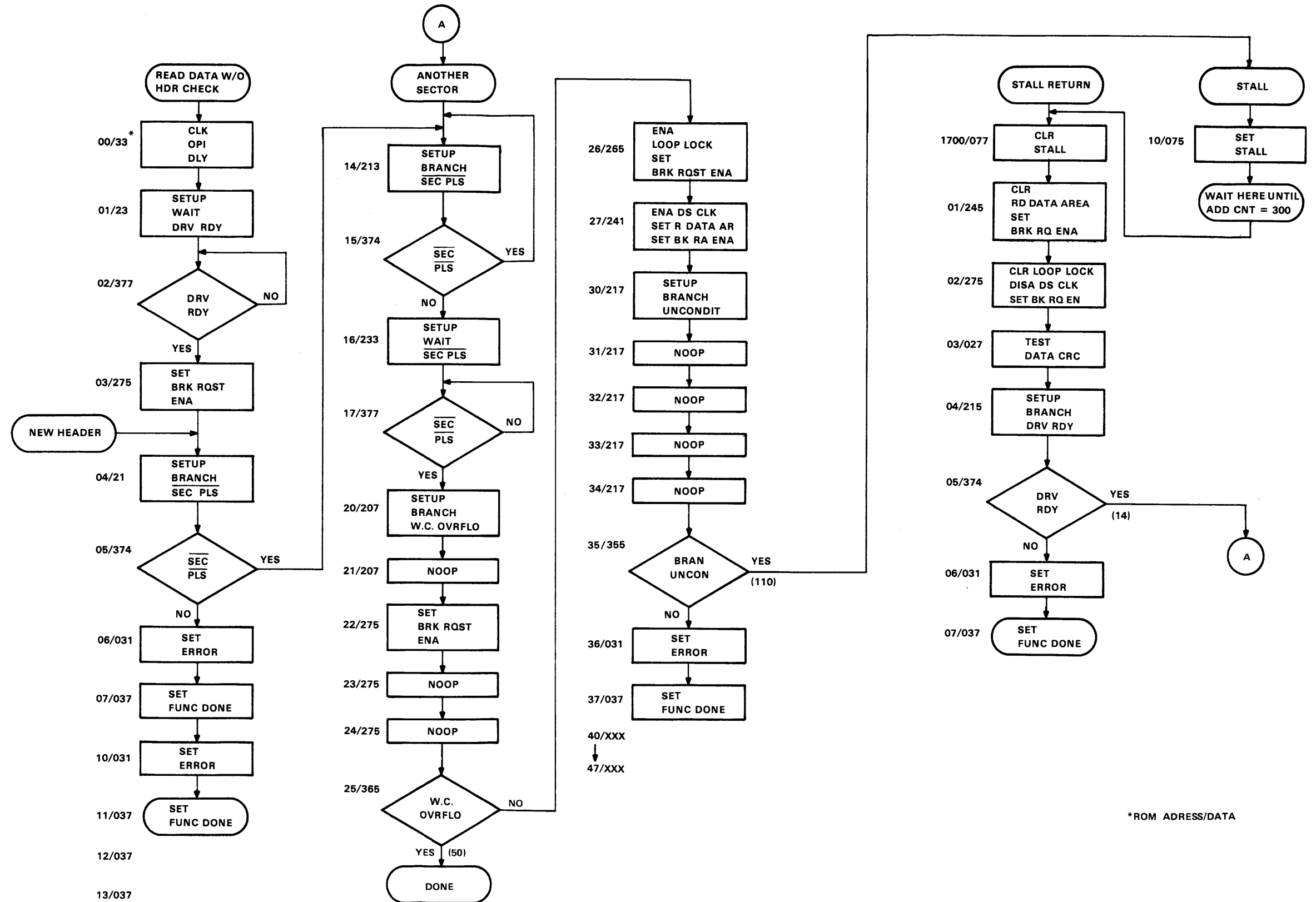
Figure 4-10 Read Data W/O HDR CK Mode Flow Diagram
