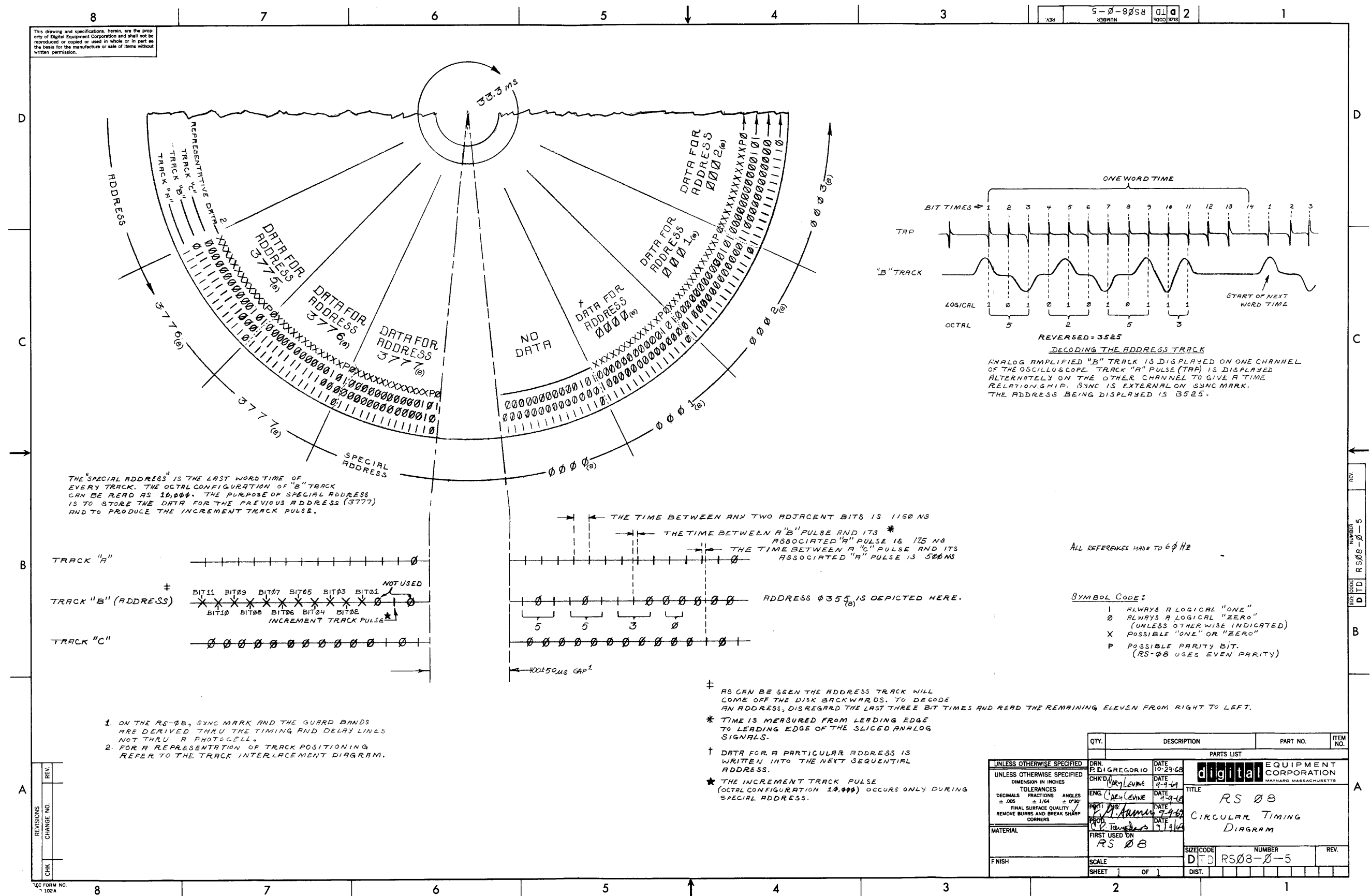
Figure 3-2 Circular Timing Diagram
