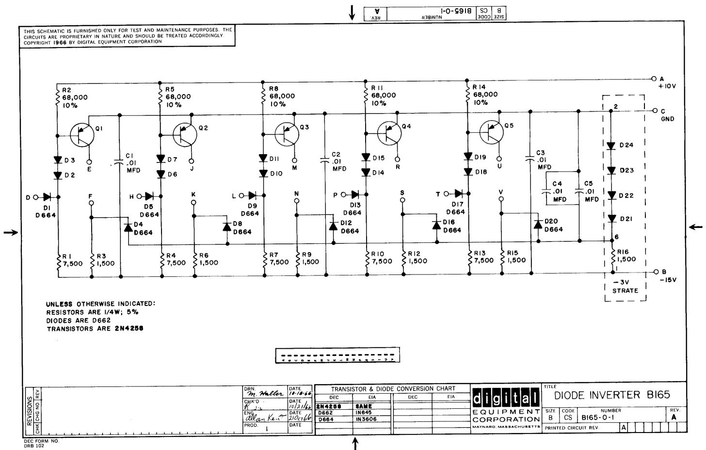
Figure 5-5 Diode Inverter B165
