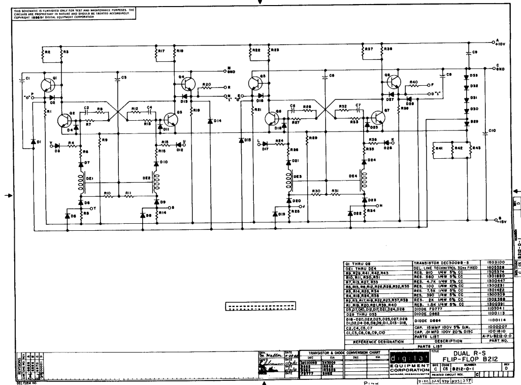
Figure 5-6 Dual R-S Flip-Flop B212
