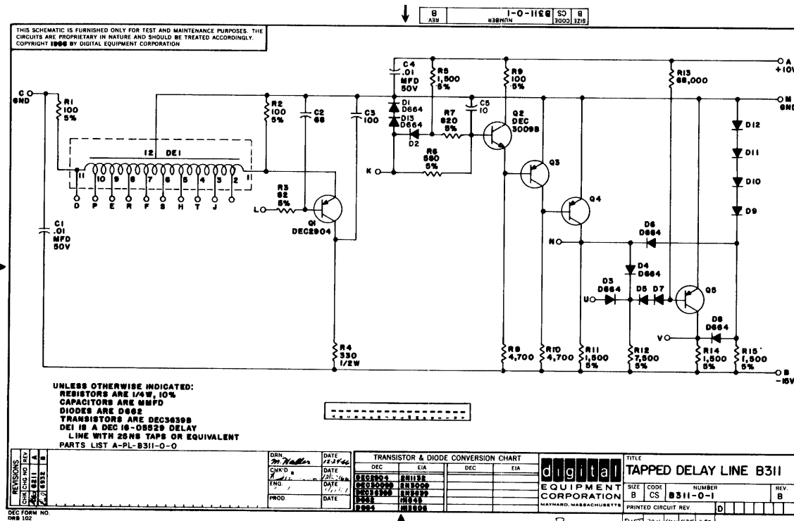
Figure 5-8 Tapped Delay Line B311
