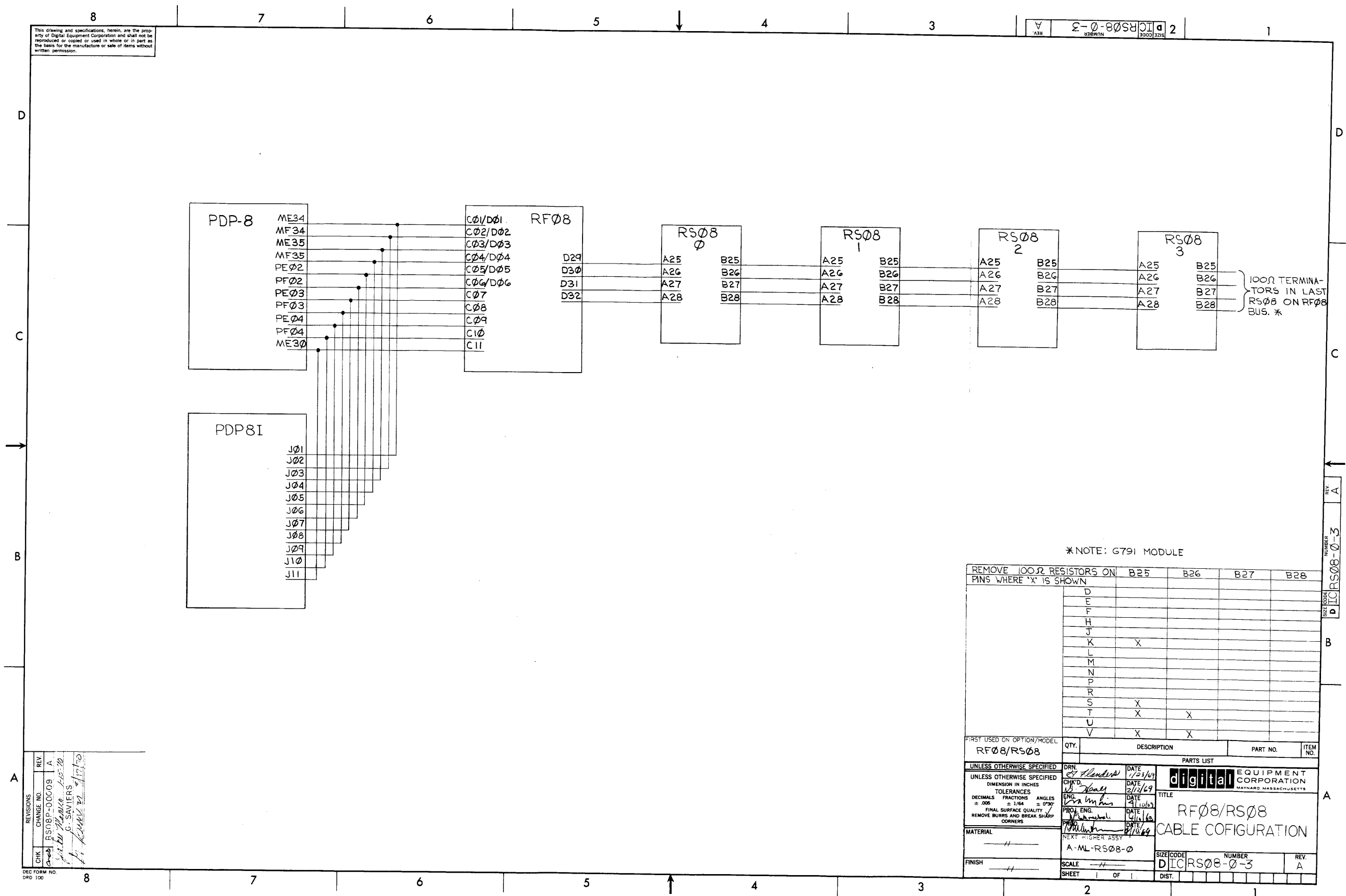
Figure 2-6 RF08 to RS08 Interconnection Cable Diagram
