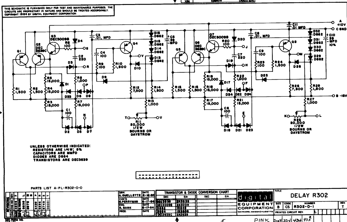
Figure 5-26 Delay R302
