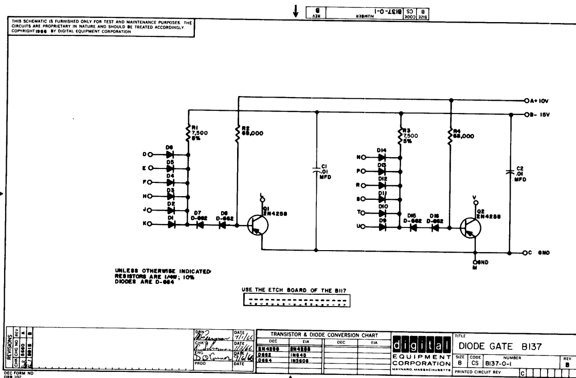
Figure 5-4 Diode Gate B137
