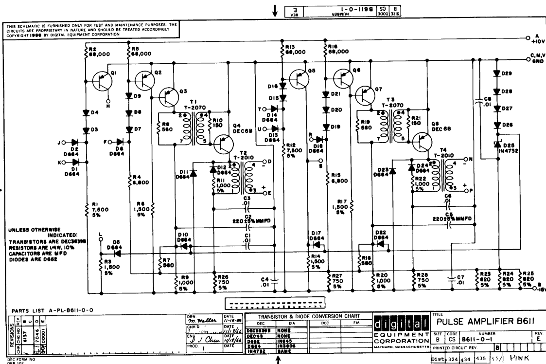
Figure 5-10 Pulse Amplifier B611
