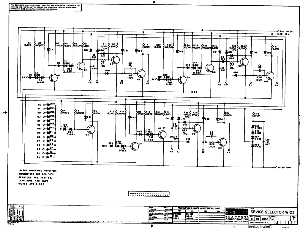
Figure 5-16 Device Selector W103
