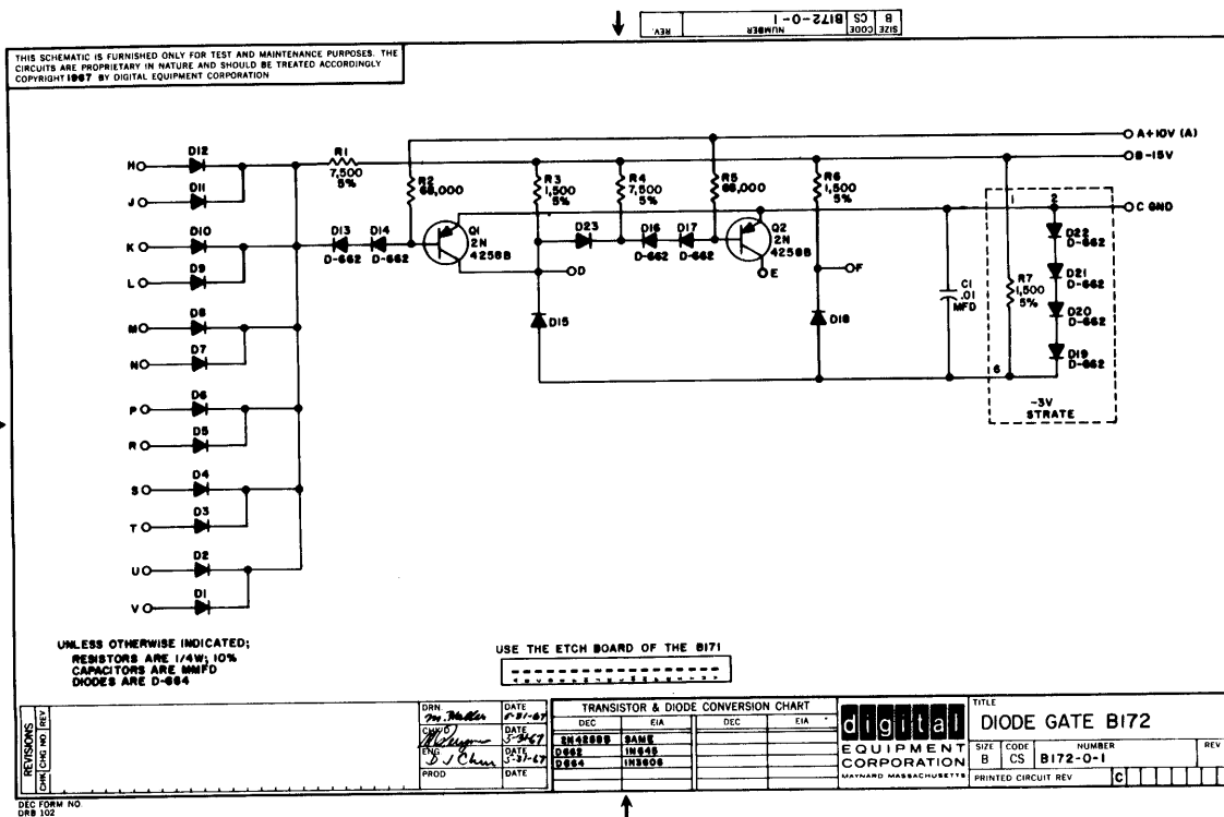
Figure 5-18 Diode Gate B172
