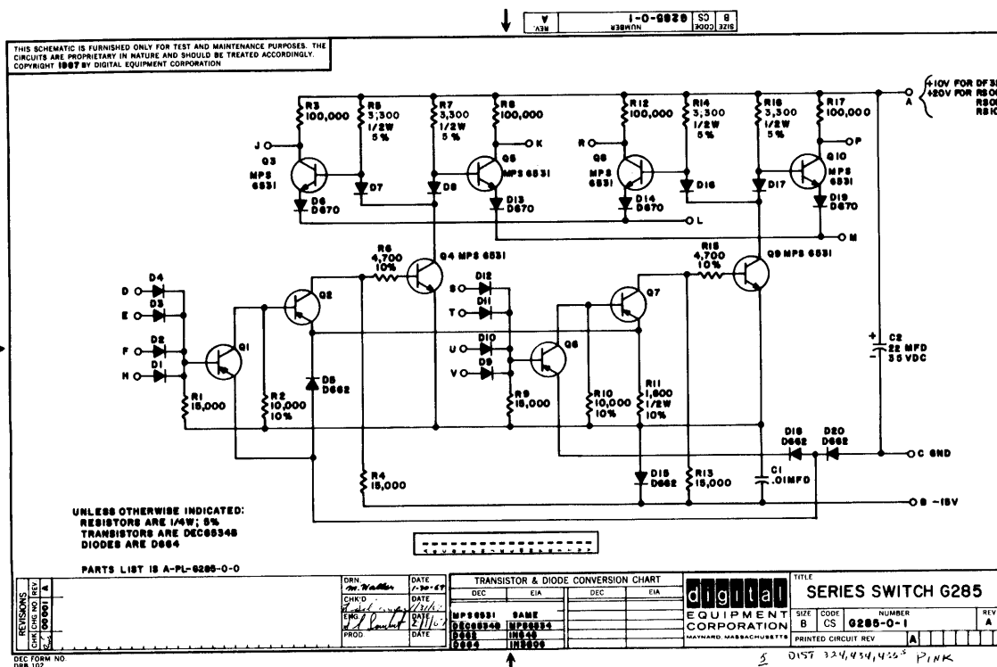
Figure 5-22 Series Switch G285
