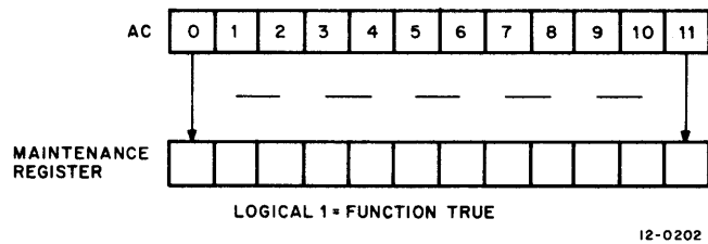
Figure 4-5 DMNT Instruction Register Diagram
