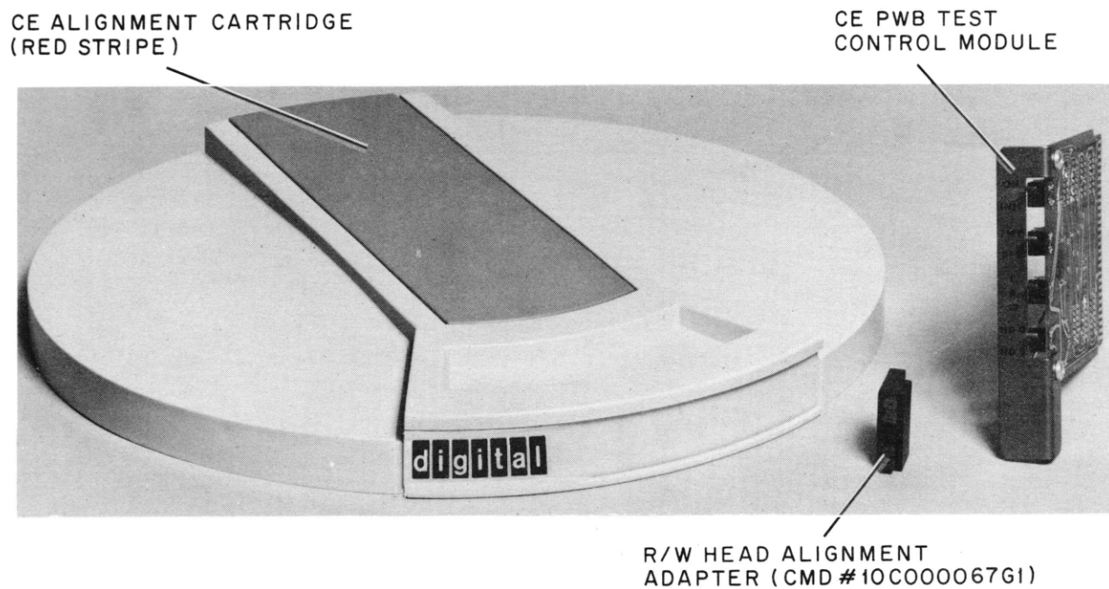
Figure 6-1 Alignment Cartridge, Control Module and Alignment Adapter
