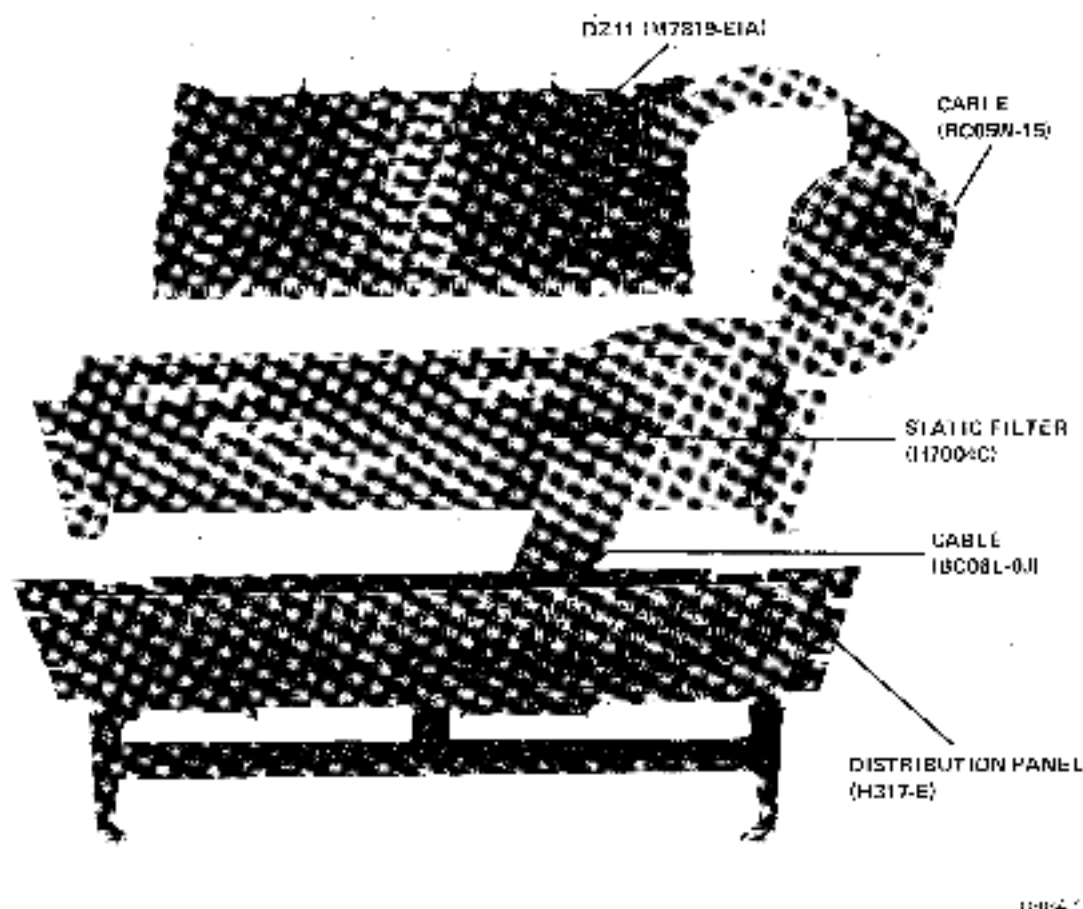
Figure 1-2 DZ11 EIA Module (M7819), Distribution Panel (H317-E), Static Filter (H7004C), and Cables (BC06L-0J and BC05W-15)
