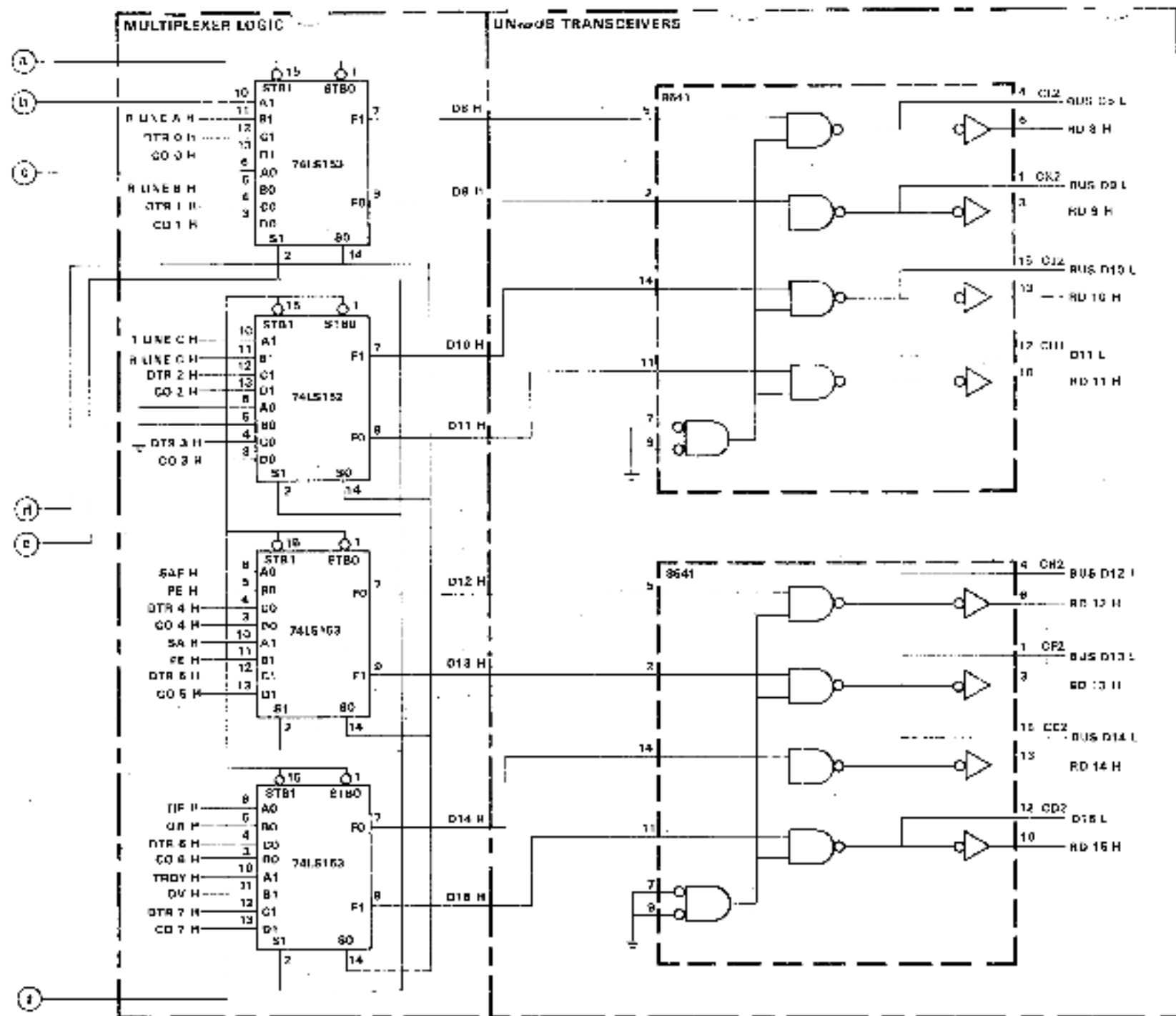
Figure 4-11 Unibus Data Flow (Sheet 2 of 2)
