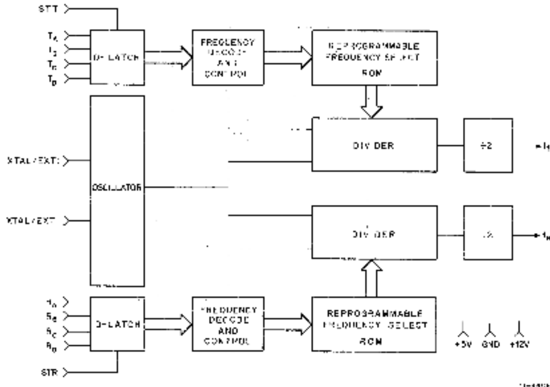
Figure C-1 Dual Baud Rate Generator Block Diagram
