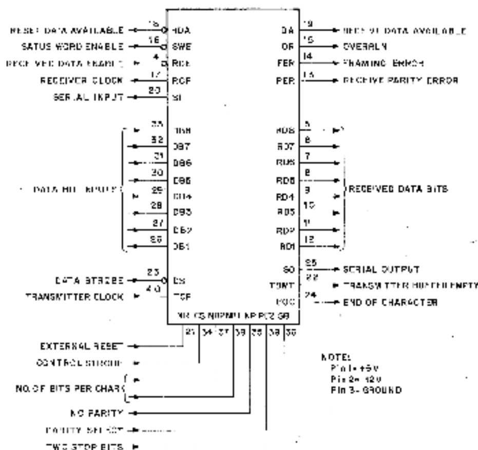
Figure B-4 UART Signal/Pin Designations
