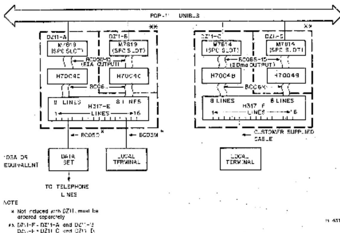
Figure 1-4 DZ11 Hardware Interconnections
