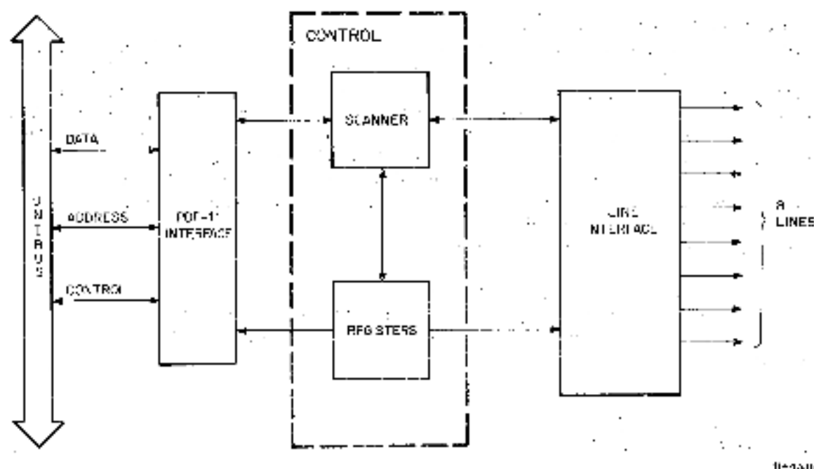
Figure 1-3 General Functional Block Diagram
