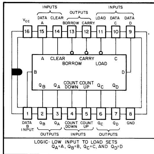
Figure A-2 74193 IC Pin Location (Top View)
