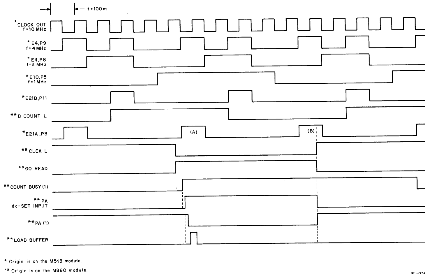
Figure 4-56 Load Buffer Register Timing
