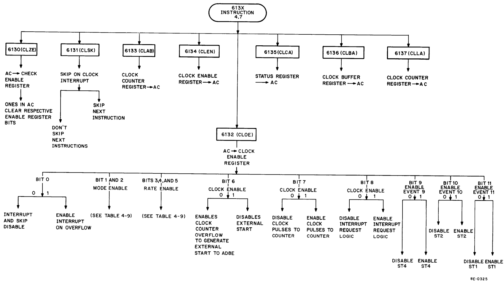
Figure 4-4 Real-Time Programmable Clock Flow Chart
