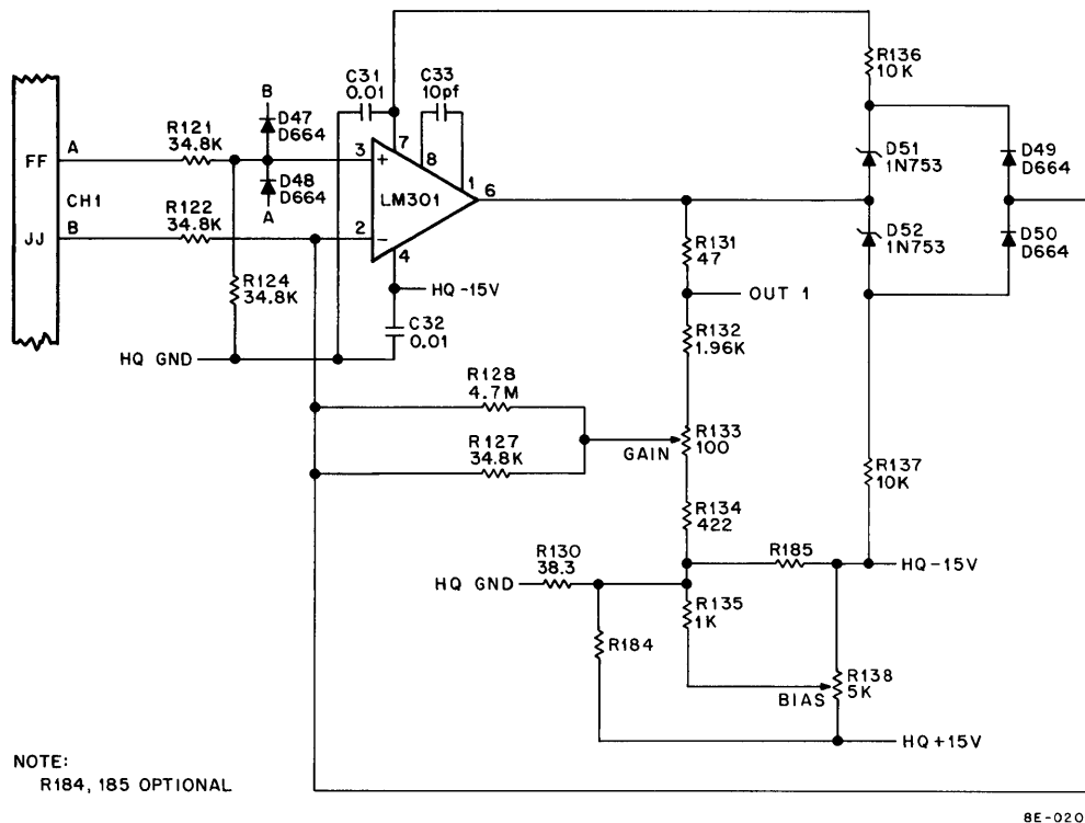
Figure 4-28 Differential Amplifier
