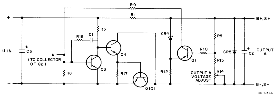
Figure 4-67 Regulator Circuitry
