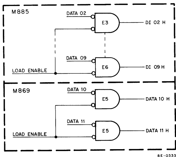
Figure 4-41 Data Gates
