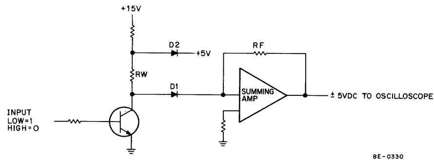
Figure 4-35 One Analog Switch and Summing Amplifier
