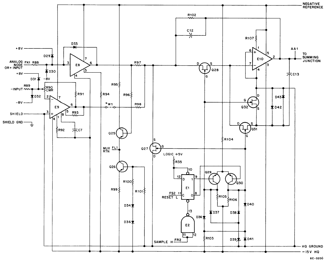
Figure 4-15 Analog Buffer and Sample and Hold Circuits
