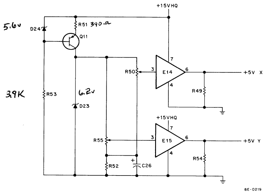
Figure 4-44 +5V Reference
