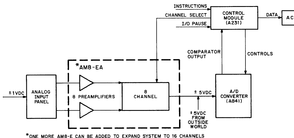
Figure 4-26 Analog Preamplifier and Multiplexer Block Diagram
