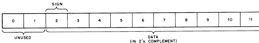
Figure 4-33 AC Input Data Format
