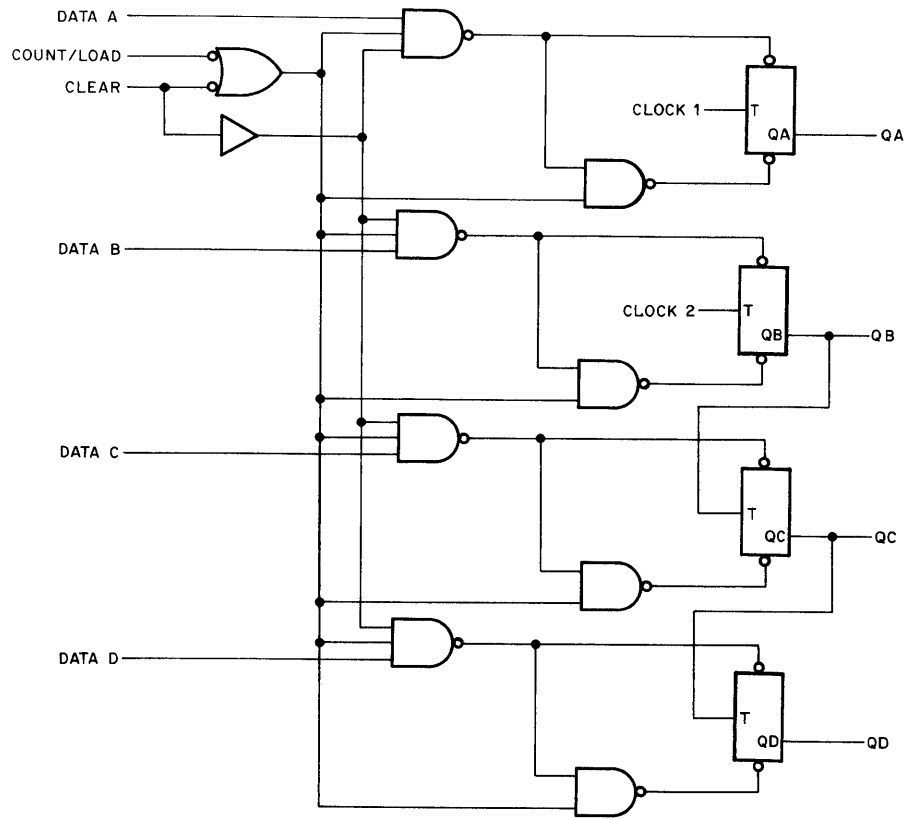
Figure A-7 DEC 74197 IC Illustrations
