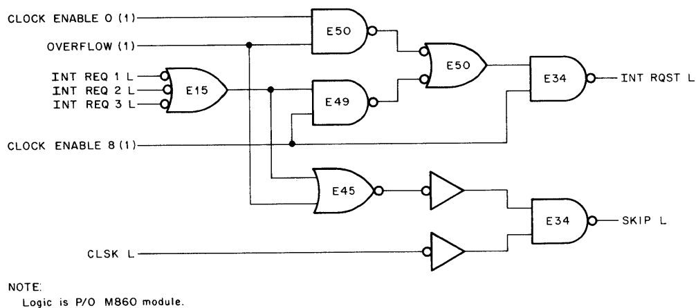
Figure 4-61 Interrupt/Skip Logic
