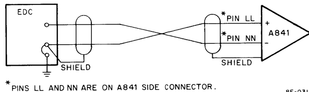
Figure 2-8 Negative Input Checkout
