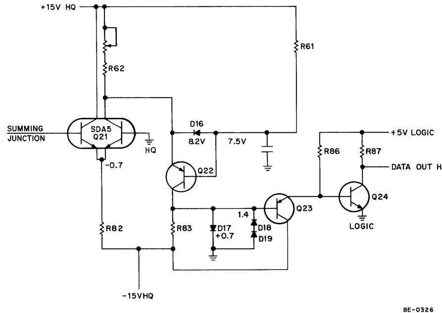
Figure 4-21 Comparator Circuits
