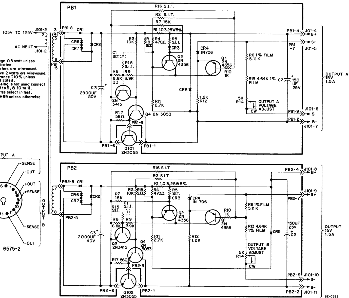
Figure 4-69 Deltron (C13495) HQ Power Supply
