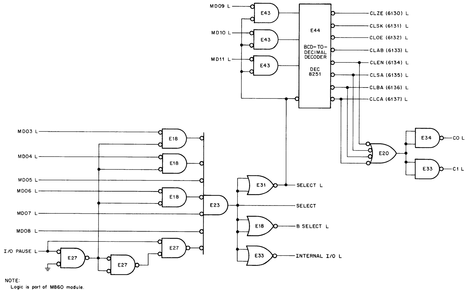
Figure 4-52 IOT Decoder Logic
