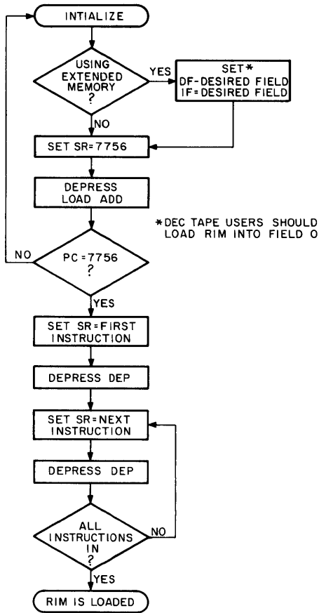
Figure 3-6 Loading the RIM Loader
