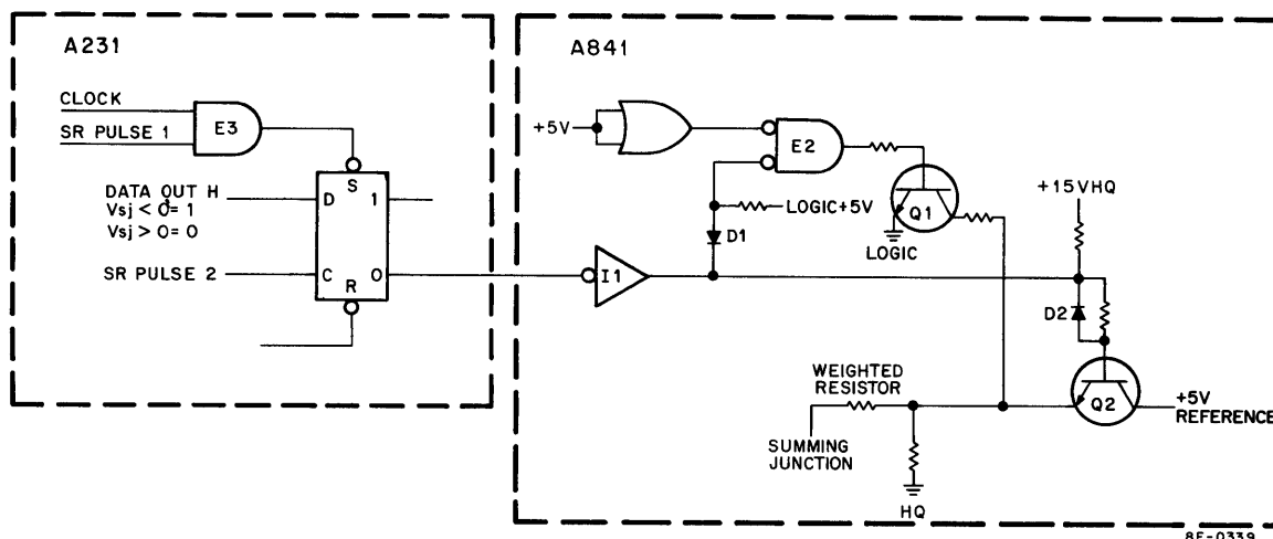
Figure 4-9 A/D Buffer and Switch Logic
