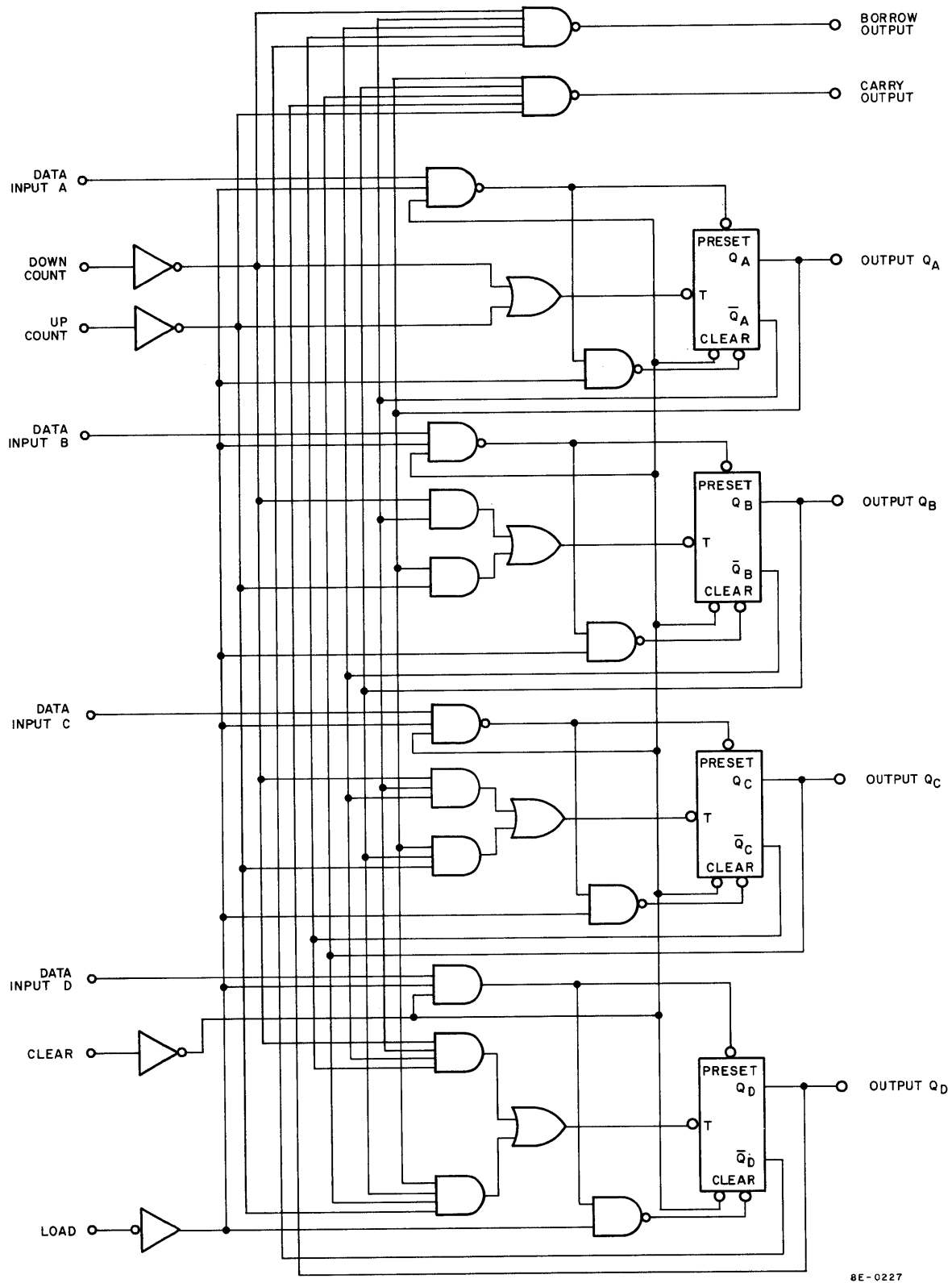
Figure A-1 74193 IC Logic Diagram
