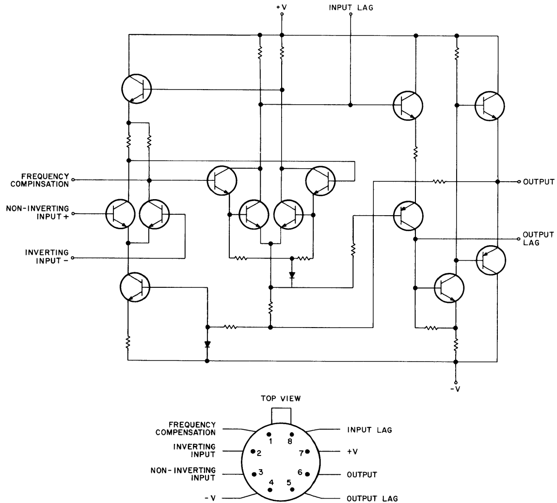
Figure A-3 DEC 1709C IC Illustrations
