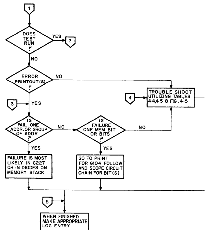
Figure 5-4 Memory Troubleshooting Flowchart
