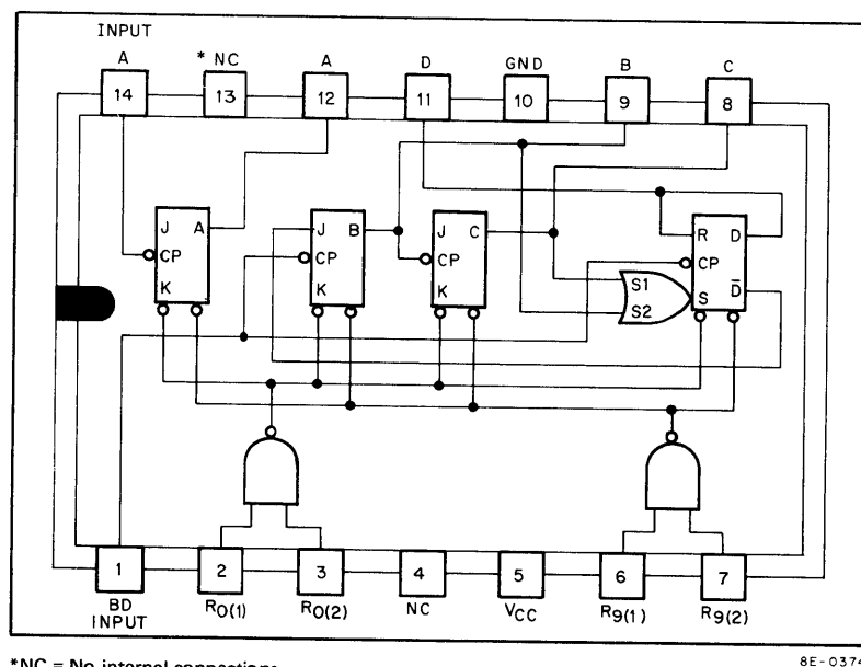
Figure A-5 DEC 7490 IC Illustrations
