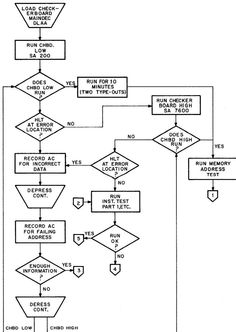
Figure 5-4 Memory Troubleshooting Flowchart
