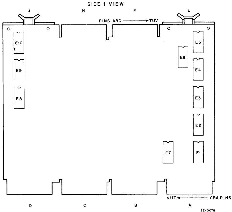
Figure 5-2 IC Location
