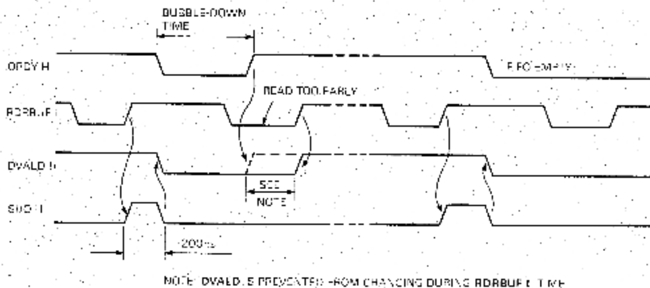
Figure 5-13 FIFO Output Timing
