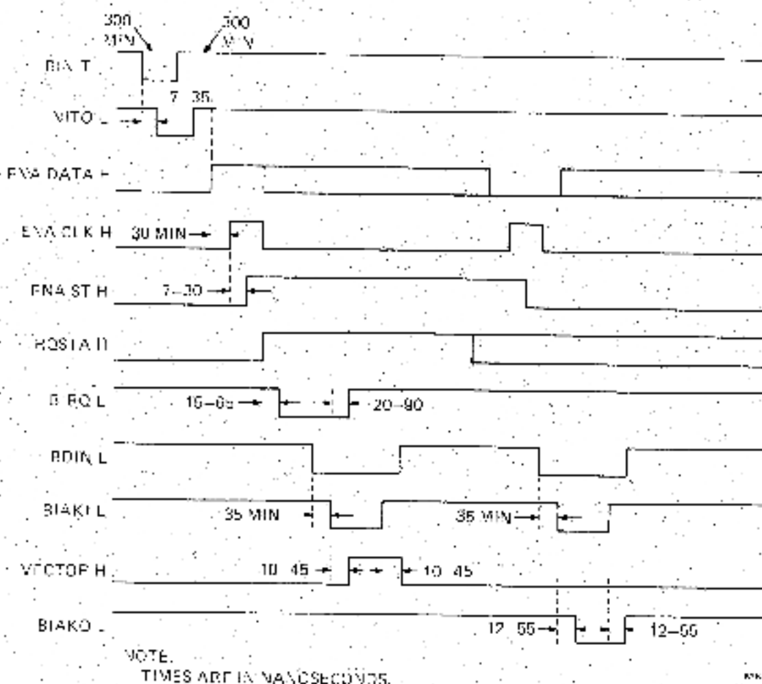
Figure A-2 DC003.A Section Timing
