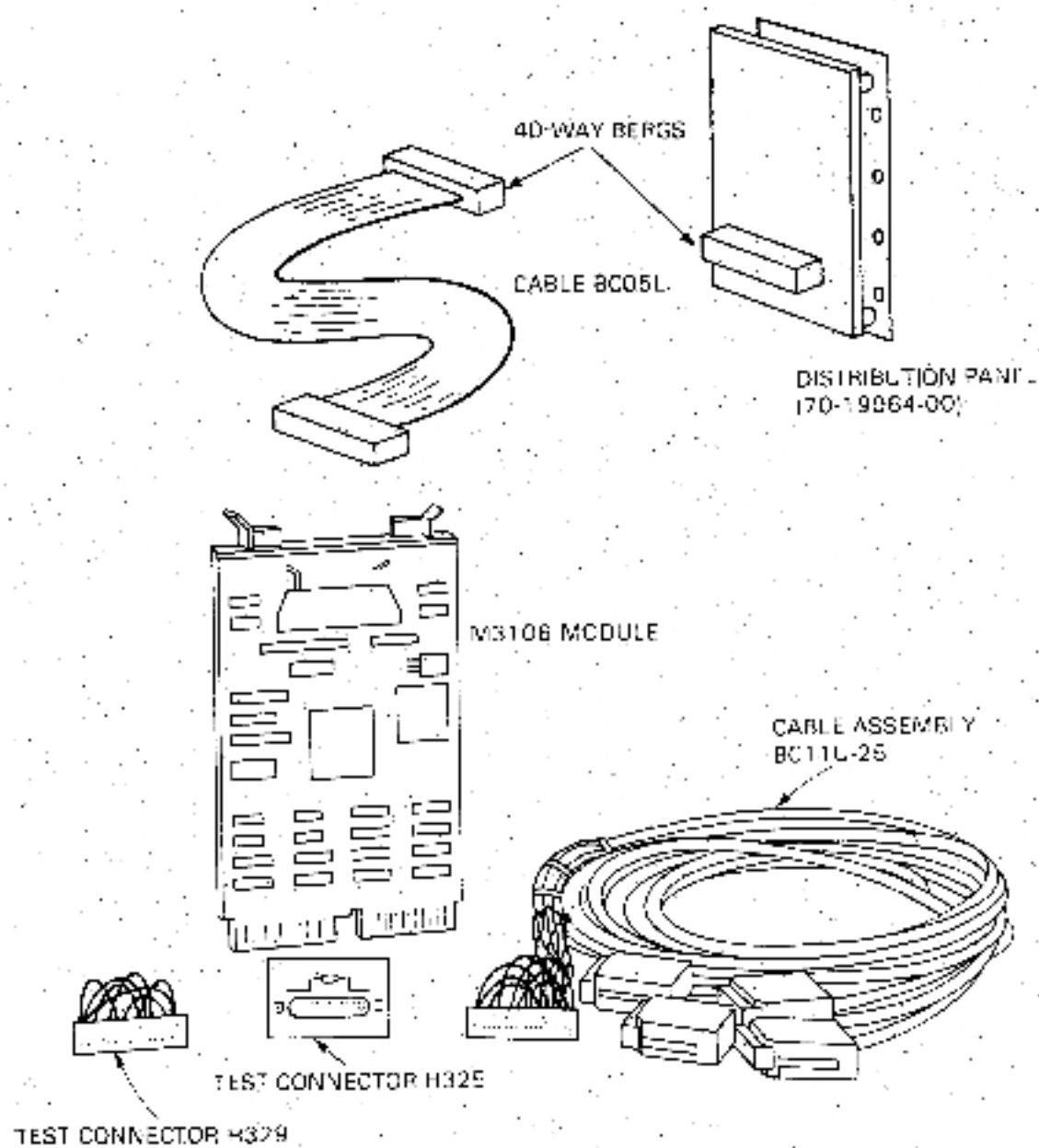
Figure 1-3 Elements of the JZQ11 Option
